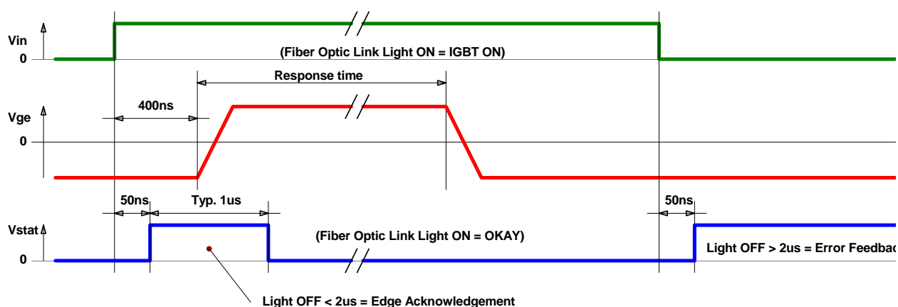
Fig. 5 Failure status feedback; signals under short circuit or over-current conditions
