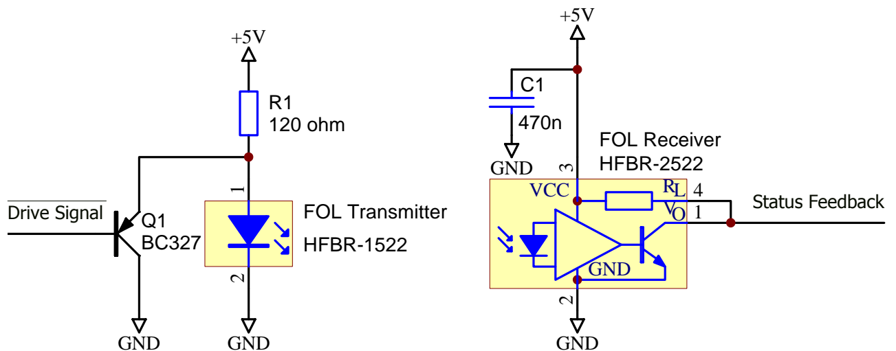
Fig. 6 Recommended circuitry for the "versatile" fiber-optic links (standard version)
