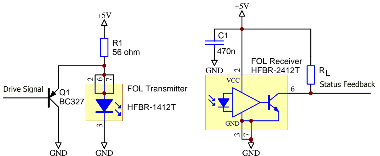
Fig. 7 Recommended circuitry for the "ST" fiber-optic links (Opt. 1)
