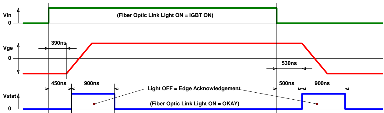
Fig. 10 Failure status feedback; signals for normal operation
