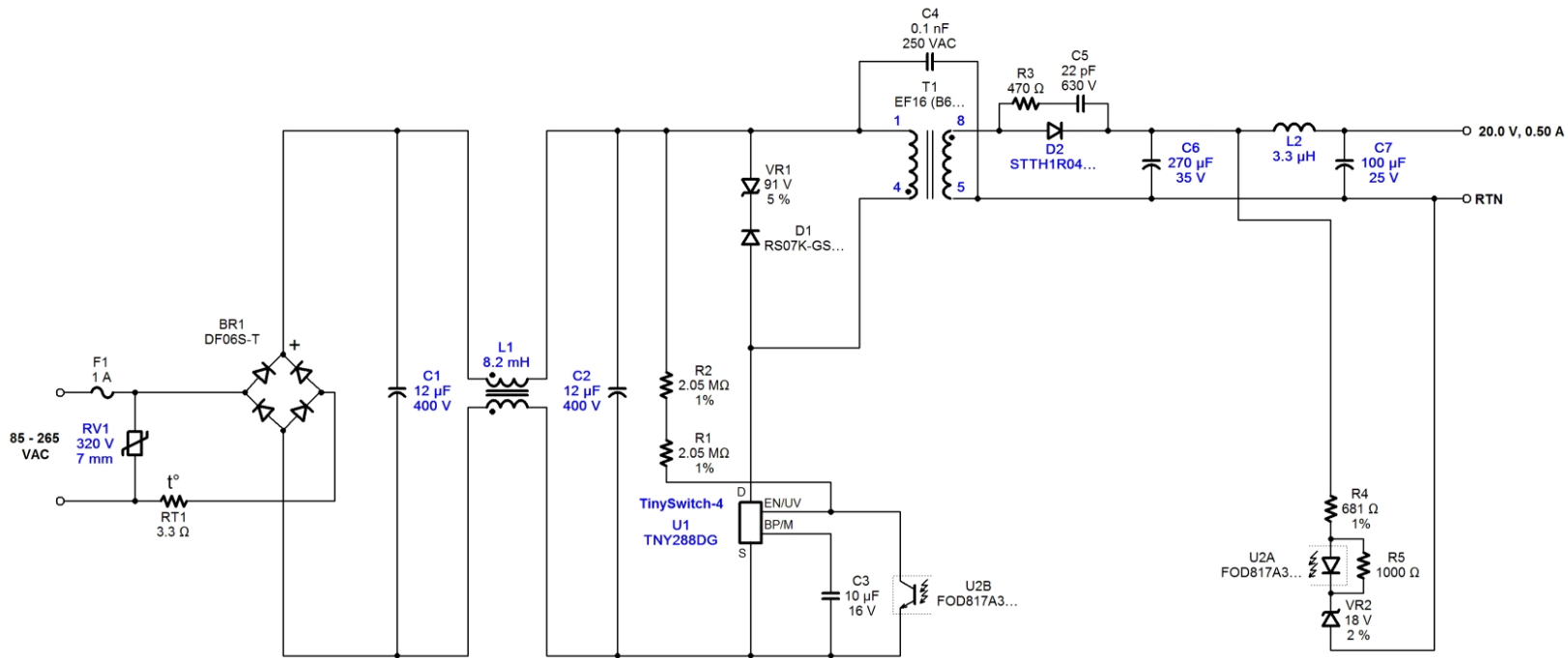
Schematic components that have been frozen by the user will appear with blue designators.
