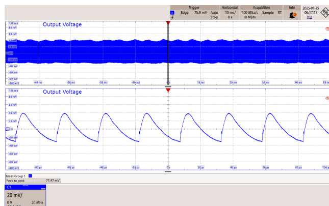
Figure 74 – 85 VAC 60 Hz.
