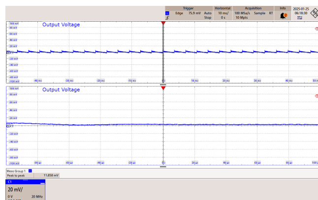
Figure 82 – 85 VAC 60 Hz.
