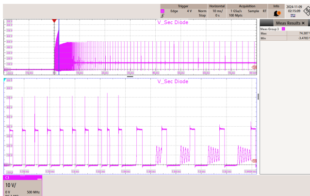
Figure 62 – 230 VAC 50 Hz.
