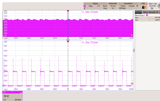
Figure 49 – 115 VAC 60 Hz.
