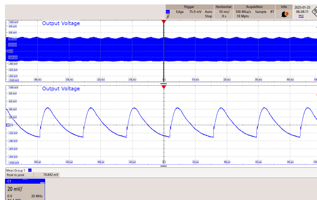
Figure 77 – 265 VAC 50 Hz.
