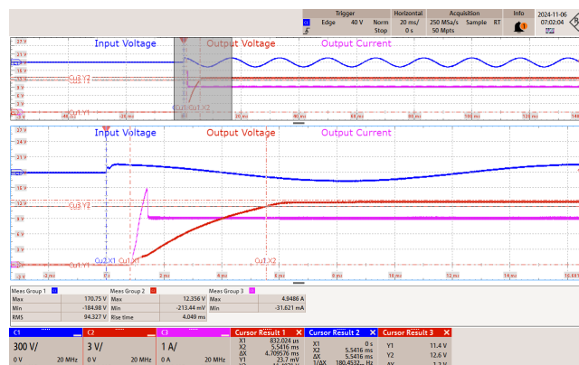
Figure 21 – 115 VAC 60 Hz.
