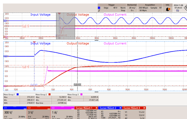
Figure 23 – 265 VAC 50 Hz.
