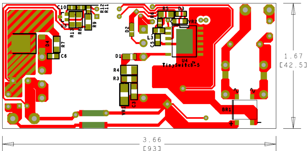
Figure 6 – Printed Circuit Board, Bottom View.
