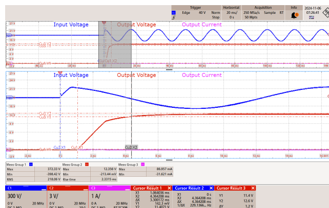
Figure 31 – 265 VAC 50 Hz.
