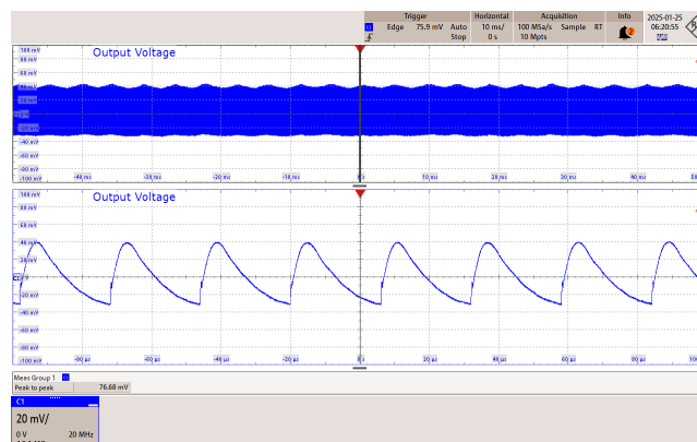
Figure 75 – 115 VAC 60 Hz.
