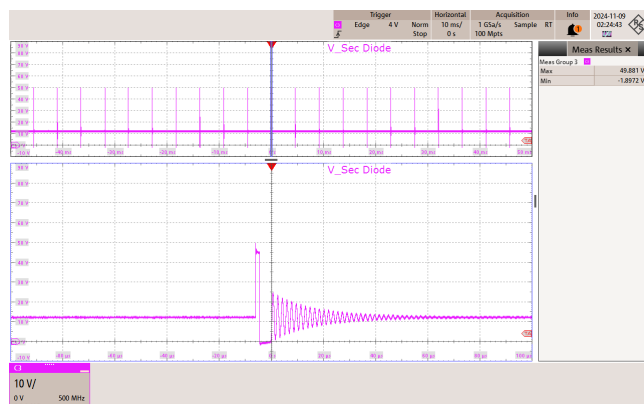
Figure 54 – 230 VAC 50 Hz.
