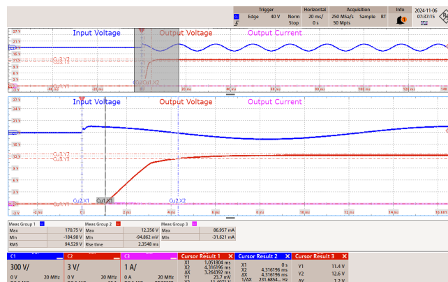
Figure 29 – 115 VAC 60 Hz.
