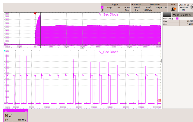
Figure 59 – 265 VAC 50 Hz.
