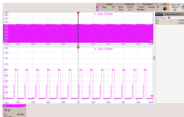
Figure 51 – 265 VAC 50 Hz.
