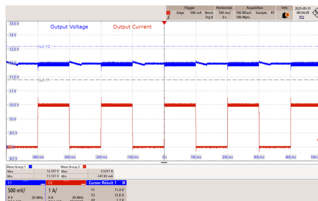
Figure 19 – 265 VAC 50 Hz.
