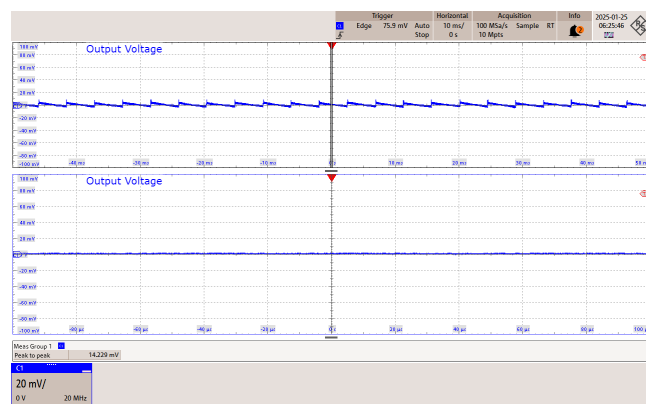
Figure 84 – 230 VAC 50 Hz.
