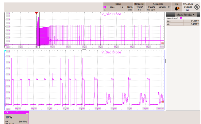
Figure 63 – 265 VAC 50 Hz.
