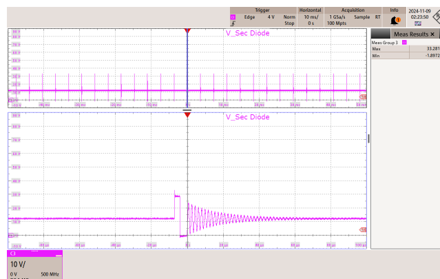
Figure 53 – 115 VAC 60 Hz.
