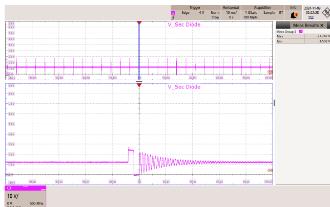
Figure 52 – 85 VAC 60 Hz.
