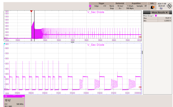
Figure 61 – 115 VAC 60 Hz.
