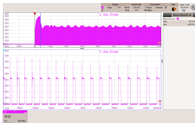
Figure 58 – 230 VAC 50 Hz.
