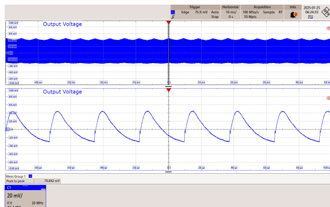
Figure 76 – 230 VAC 50 Hz.
