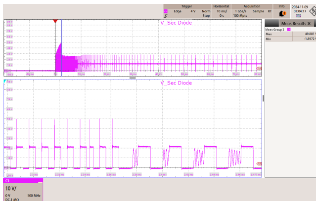
Figure 60 – 85 VAC 60 Hz.
