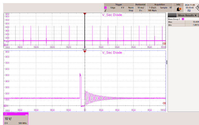
Figure 55 – 265 VAC 50 Hz.
