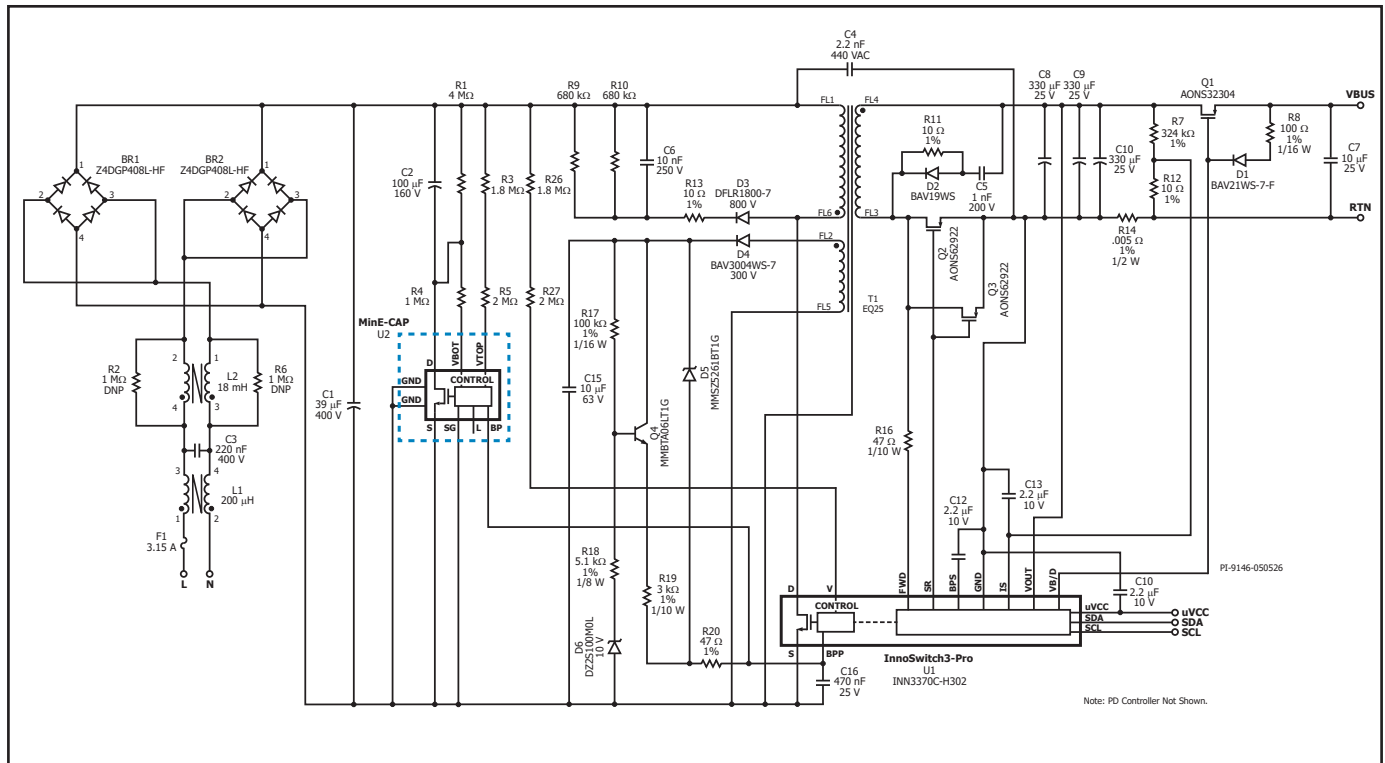
Figure 8. Schematic of a 65 W USB PD 3.0 Adapter Design.
