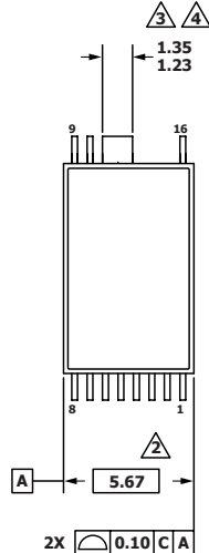
BOTTOM VIEW
