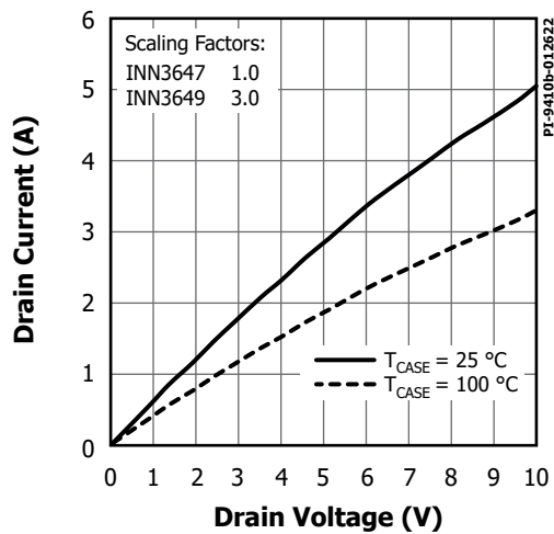
Figure 46. Output Characteristics.
