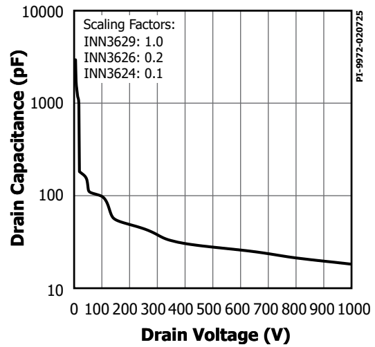
Figure 48. C_{oss} vs. Drain Voltage.
