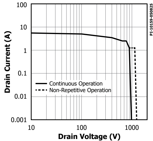
Figure 52. Maximum Allowable Drain Current vs. Drain Voltage INN3626.
