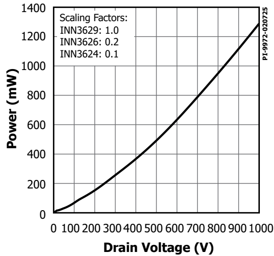
Figure 47. Drain Capacitance Power.
