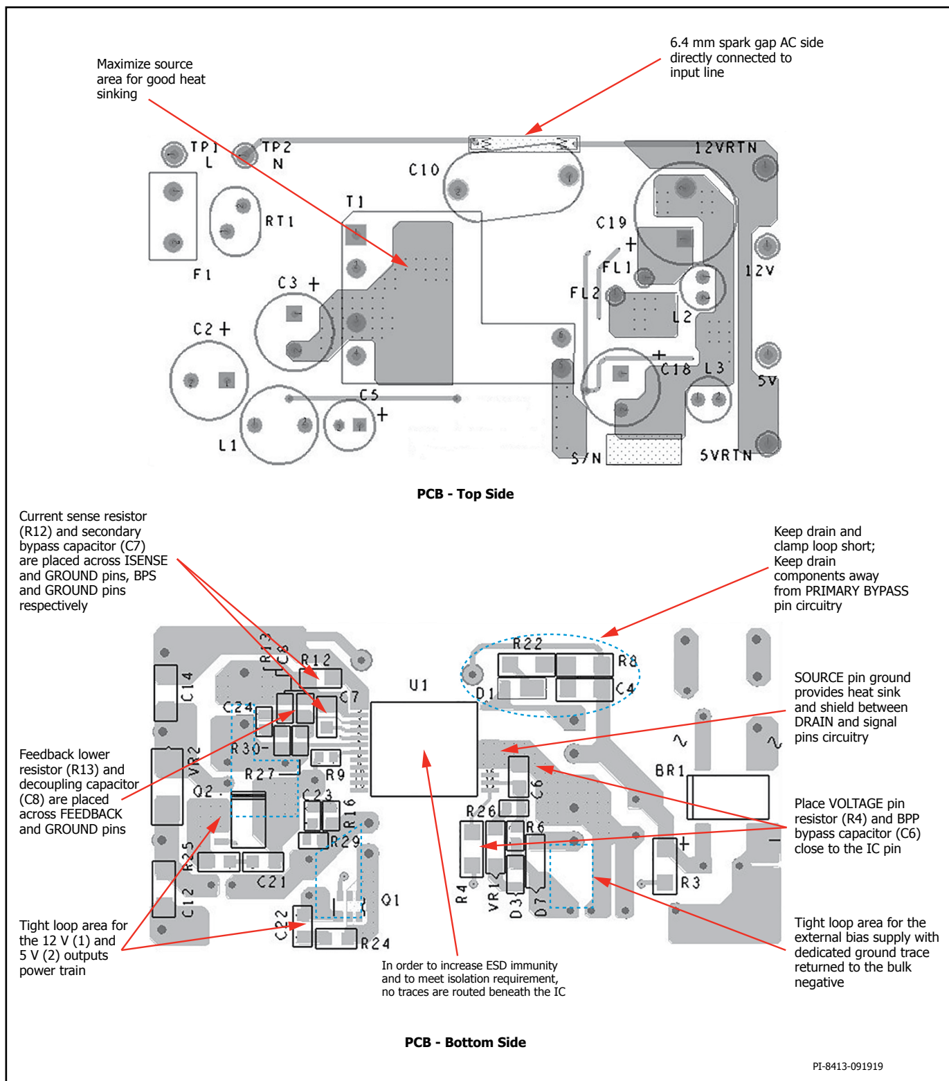
Figure 19. PCB.
