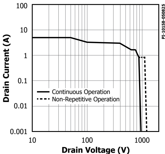
Figure 51. Maximum Allowable Drain Current vs. Drain Voltage INN3624.
