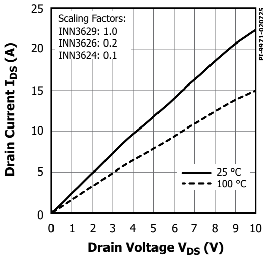
Figure 49. Output Characteristics.
