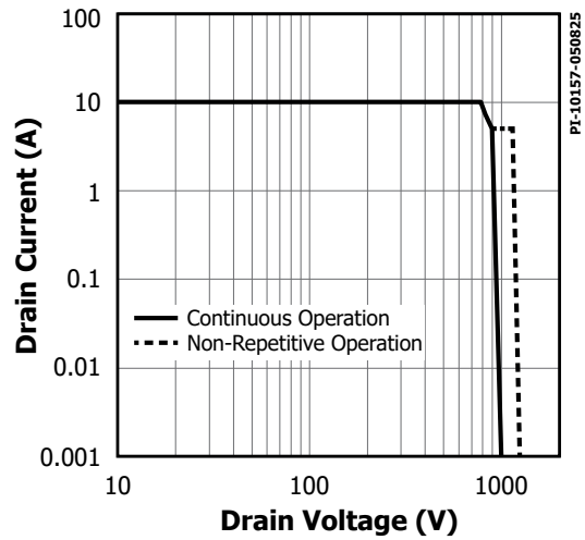
Figure 50. Maximum Allowable Drain Current vs. Drain Voltage INN3629.
