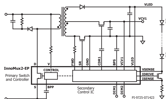
Figure 1. Typical Application with LED Driver. (IMX2353F (1700 V) does not support LED Driver)
