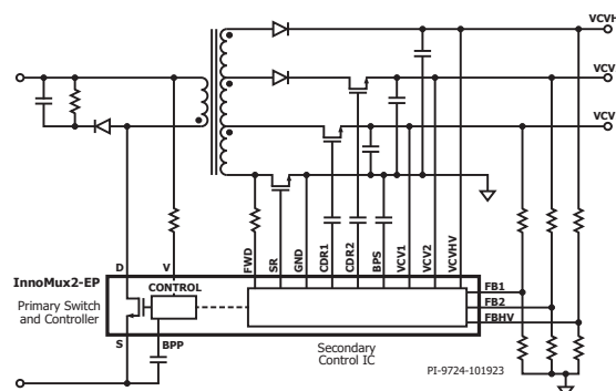
Figure 3. Typical Application with Three Constant Voltages.
