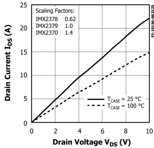
Figure 31. Output Characteristics.
