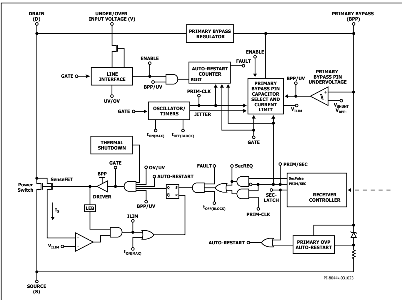
Figure 6. InnoMux2-EP Primary Block Diagram.
