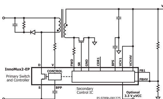
Figure 4. Typical Application with One Output.
