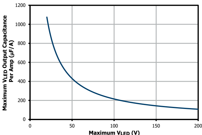
Figure 19. Maximum LED Output Capacitance.
