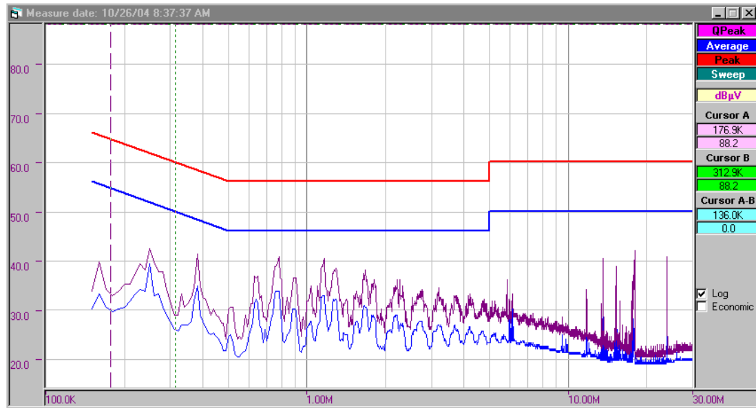
Figure 25 - Conducted EMI, Maximum Steady State Load, 230 VAC, 50 Hz, and EN5022 B Limits Secondary Ground Floating
