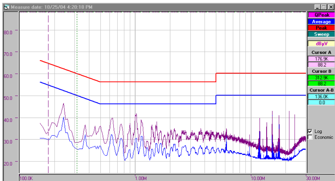
Figure 26 - Conducted EMI, Maximum Steady State Load, 230 VAC, 50 Hz, and EN5022 B Limits Secondary Ground connected to Artificial Hand
