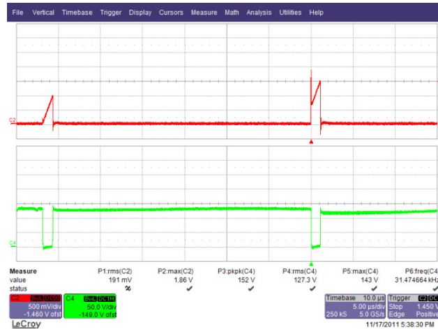
Figure 46 – 90 VAC, 60 Hz Output Short Condition. Upper: I_{DRAIN} , 500 mA / div. Lower: V_{DRAIN} , 50 V, 5 μs / div.
