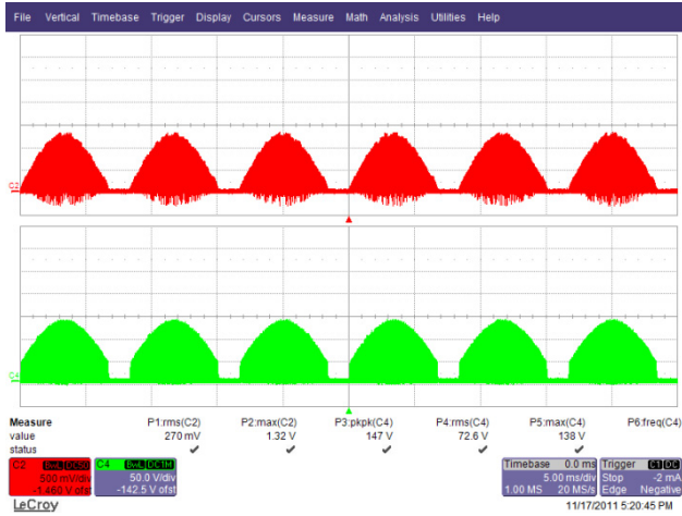
Figure 39 – 90 VAC, 60 Hz. Upper: I_{DRAIN} , 500 mA / div. Lower: V_{DRAIN} , 50 V, 5 ms / div.
