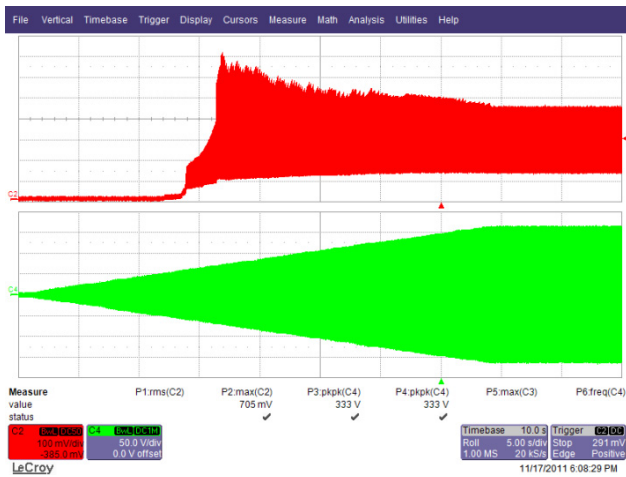
Figure 53 – 0 VAC – 115 VAC, 3 V / \mu s Slew Rate. Upper: I_{OUT} , 100 mA / div. Lower: V_{INAC} , 50 V, 5 s / div.
