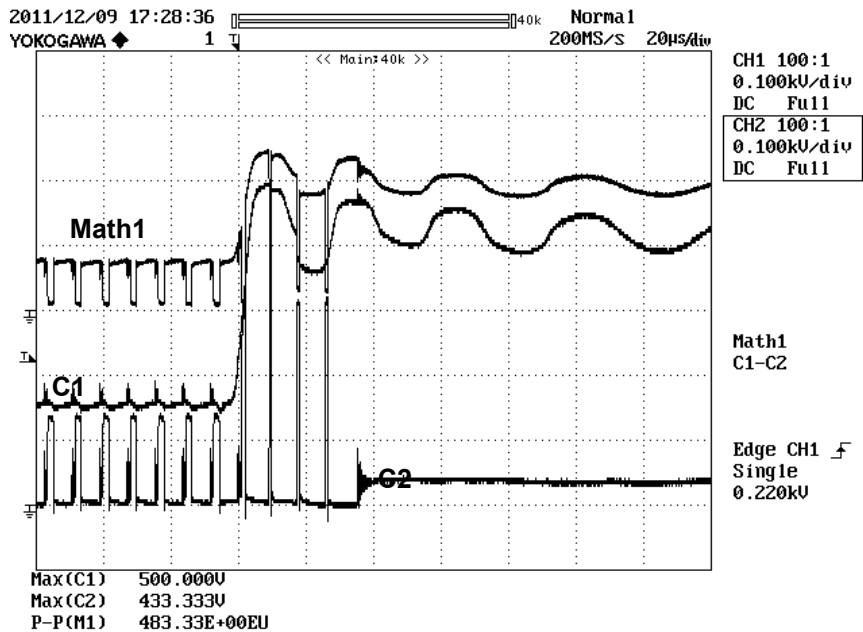
Figure 57 – 1 kV (90° Injection Phase) Differential Surge VDS Waveforms.
