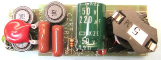
Figure 2 – Populated Circuit Board, Top View.
