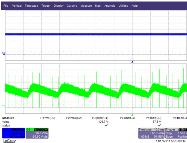
Figure 49 – 90 VAC, 60 Hz Open Load Characteristic. Upper: V_{OUT} , 20 V / div. Lower: V_{DRAIN} , 20 V / div., 5 ms / div.
