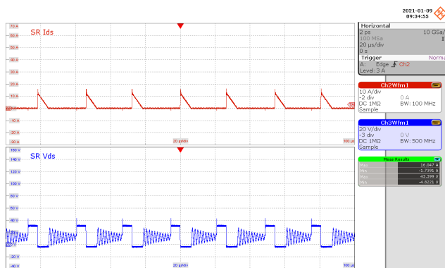
Figure 110 – SR FET Drain Voltage and Current. 100 VAC, 15.0 V, 3 A Load (43.4 V MAX ). CH3: V DRAIN(SR) , 20 V / div. CH2: I DRAIN(SR) , 10 A / div. Time: 20 μs / div.
