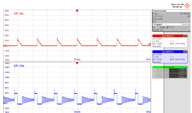
Figure 111 – SR FET Drain Voltage and Current. 132 VAC, 15.0 V, 3 A Load (56.05 V MAX ). CH3: V DRAIN(SR) , 20 V / div. CH2: I DRAIN(SR) , 10 A / div. Time: 20 μs / div.
