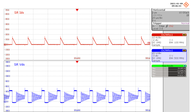
Figure 113 – SR FET Drain Voltage and Current. 132 VAC, 20.0 V, 3.25 A Load (55.26 V MAX ). CH3: V DRAIN(SR) , 20 V / div. CH2: I DRAIN(SR) , 10 A / div. Time: 20 μs / div.
