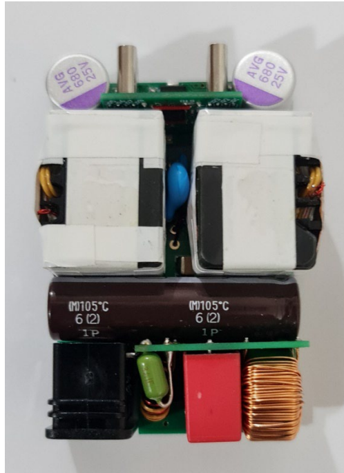
Figure 2 – Populated Circuit Board Photograph - Top.
