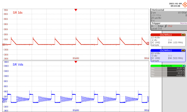
Figure 108 – SR FET Drain Voltage and Current. 100 VAC, 12.0 V, 3 A Load (44.19 V MAX ). CH3: V DRAIN(SR) , 20 V / div. CH2: I DRAIN(SR) , 10 A / div. Time: 20 μs / div.
