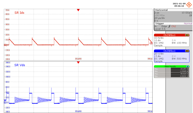
Figure 109 – SR FET Drain Voltage and Current. 132 VAC, 12.0 V, 3 A Load (58.42 V MAX ). CH3: V DRAIN(SR) , 20 V / div. CH2: I DRAIN(SR) , 10 A / div. Time: 20 μs / div.
