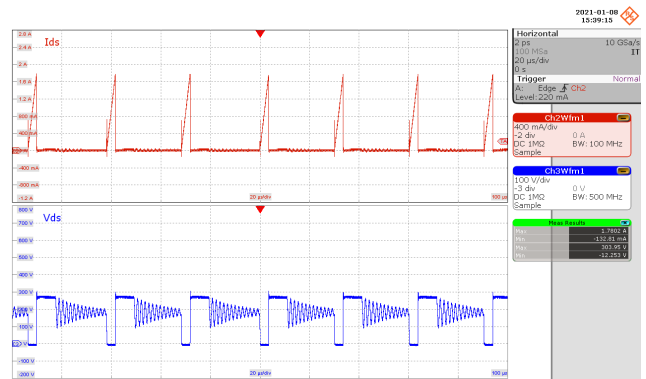
Figure 99 – Primary Drain Voltage and Current. 132 VAC, 12.0 V, 3 A Load (303.95 V MAX ). CH3: V DRAIN , 100 V / div. CH2: I DRAIN , 0.4 A / div. Time: 20 μs / div.
