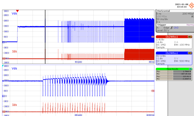
Figure 50 – Primary Drain Voltage and Current. 100 VAC, 5.0 V, 5 A Load (223.91 V MAX ). CH3: V DRAIN , 50 V / div. CH2: I DRAIN , 1 A / div. Time: 50 ms / div. (250 μs / div. Zoom)
