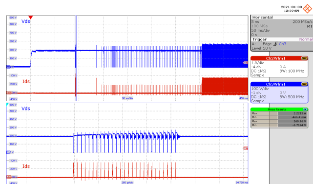
Figure 51 – Primary Drain Voltage and Current. 132 VAC, 5.0 V, 3 A Load (269.96 V MAX ). CH3: V DRAIN , 100 V / div. CH2: I DRAIN , 1 A / div. Time: 50 ms / div. (250 μs / div. Zoom)
