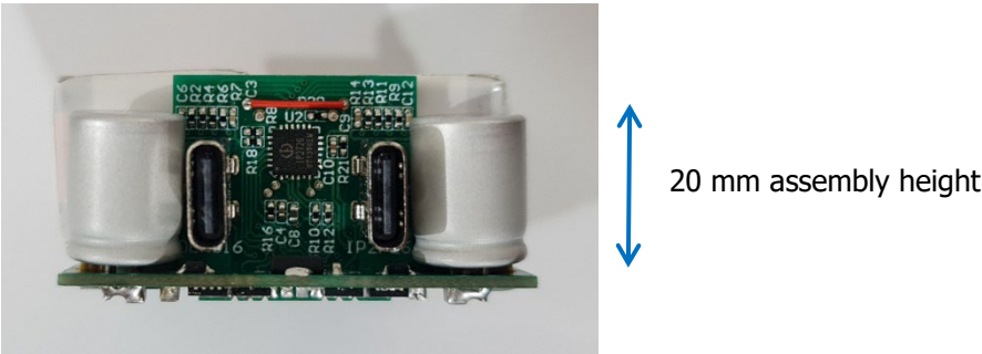
Figure 4 – Populated Circuit Board Photograph - Front.
