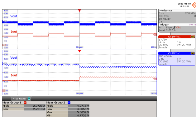
Figure 60 – Transient Response. 100 VAC, 5.0 V, 2.25 – 3.0 A Load Step. V_{MIN} : 4.7739 V, V_{MAX} : 5.0032 V. CH2: V_{OUT} , 0.2 V / div. CH1: I_{LOAD} , 1 A / div. Time: 50 ms / div. (250 \mu s / div. Zoom)
