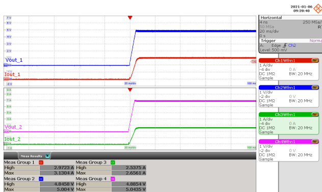
Figure 48 – Output Voltage and Current. 100 VAC, 5.0 V, 3 A Load (5.04 V MAX ). CH2: V OUT1 , 1 V / div. CH1: I LOAD1 , 1 A / div. CH4: V OUT2 , 1 V / div. CH3: I LOAD2 , 1 A / div. Time: 20 ms / div.
