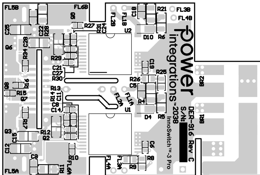
Main Board Bottom Overlay Figure 11 – Main Board Rev C PCB Overlay Layers.
