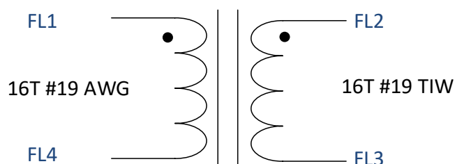
Figure 15 – Inductor Electrical Diagram.
