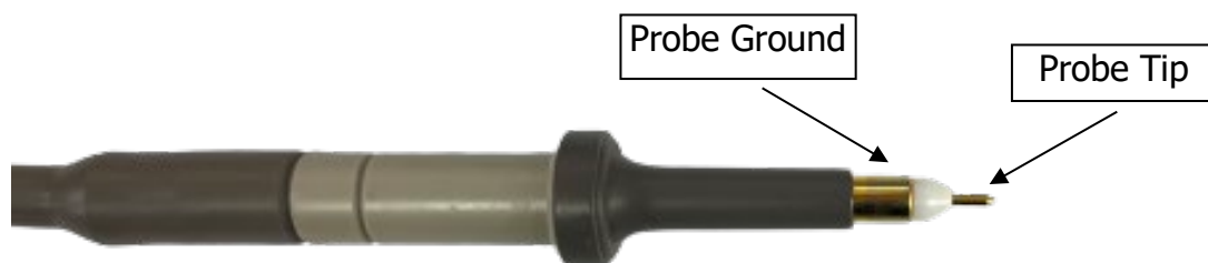
Figure 56 – Oscilloscope Probe Prepared for Ripple Measurement (End Cap and Ground Lead Removed).
