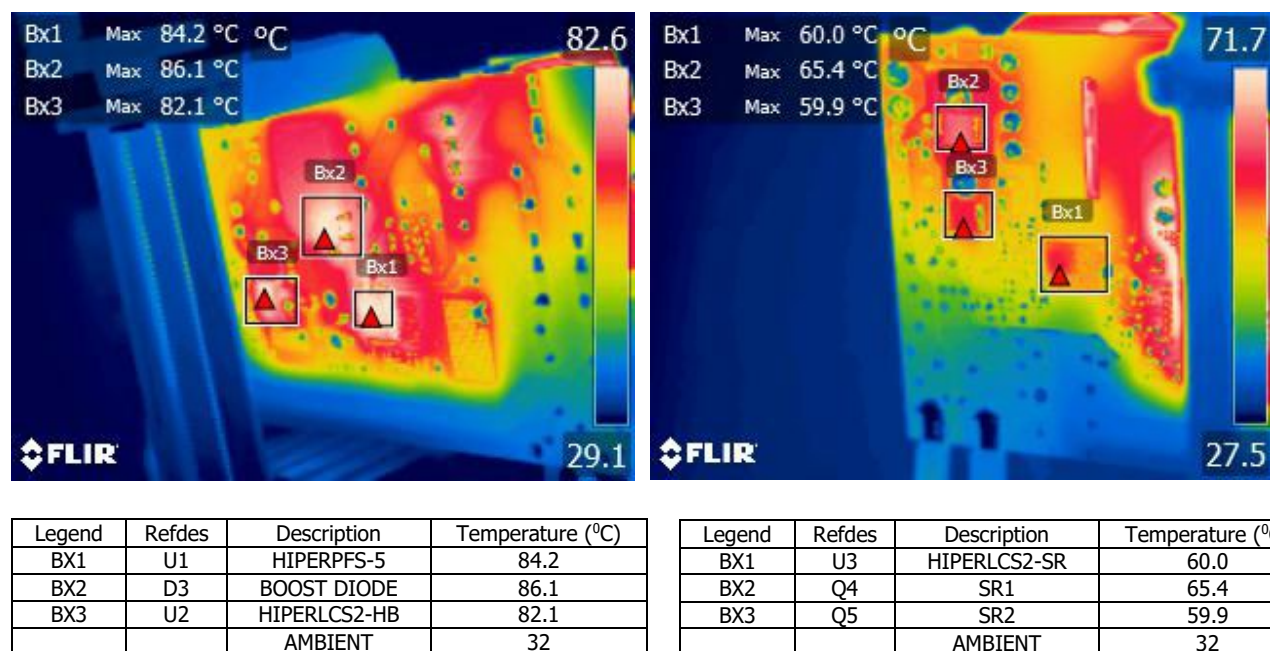
Figure 66 – Bottom Side Thermal Picture, 100% Load, 90 VAC.
