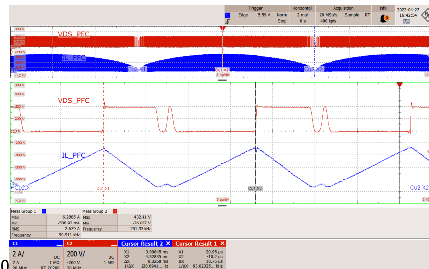
Figure 37 – VDS and Choke Current, 115 VAC.
