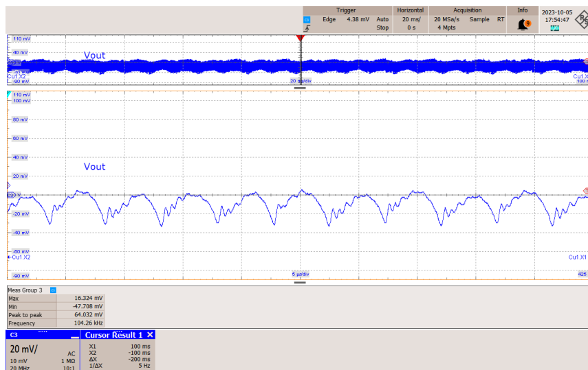
Figure 58 – Output Ripple at Full Load (9.2 A), 230 VAC. Time Division: 20 ms/div. Zoom Time Division: 5 μs/div. CH3: V_{OUT} , 20 mV/div.
