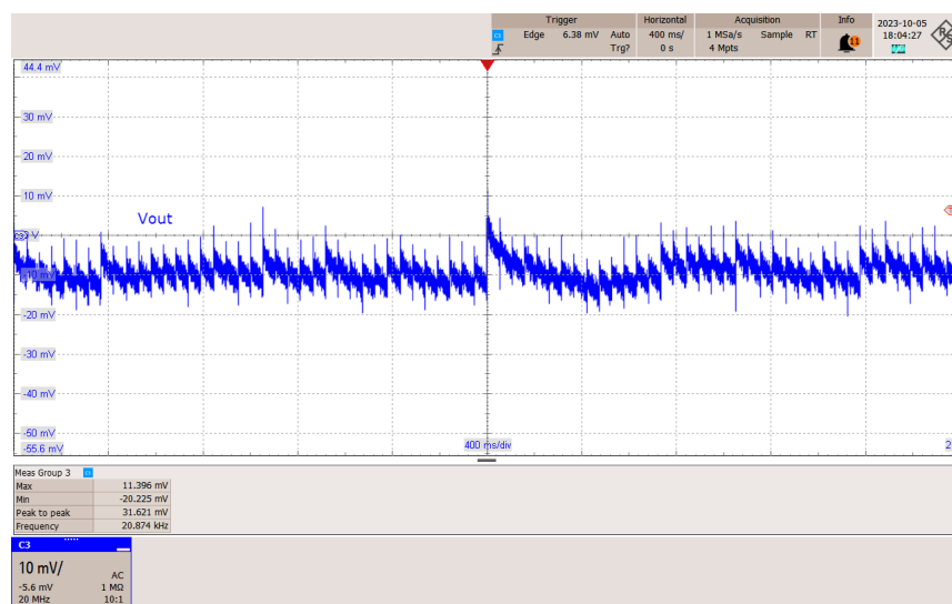
Figure 62 – Output Ripple at No Load, 230 VAC.
