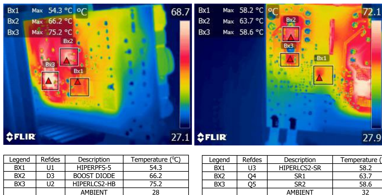
Figure 70 – Bottom Side Thermal Picture, 100% Load, 265 VAC.
