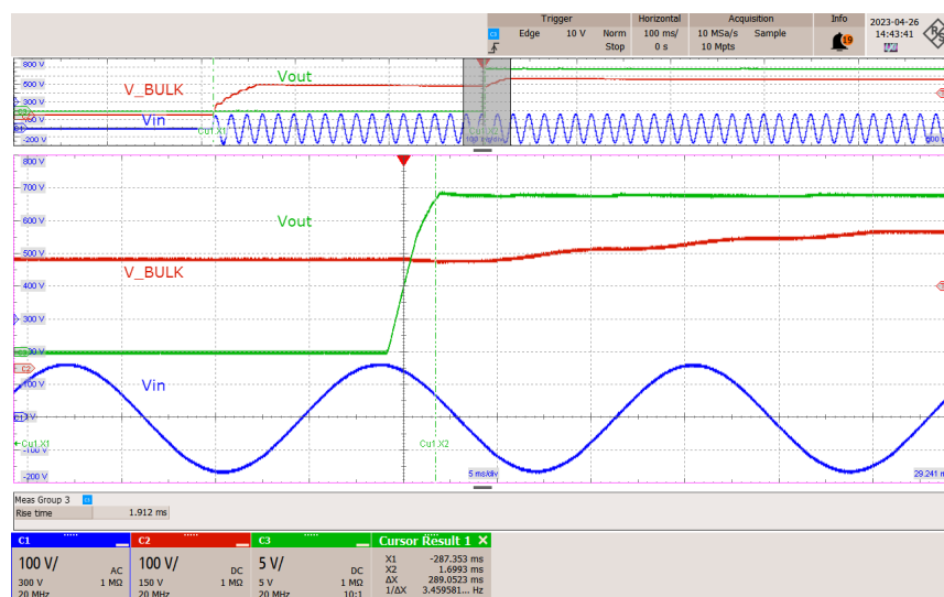
Figure 43 – Unit Start-up, 115 VAC, No Load.
