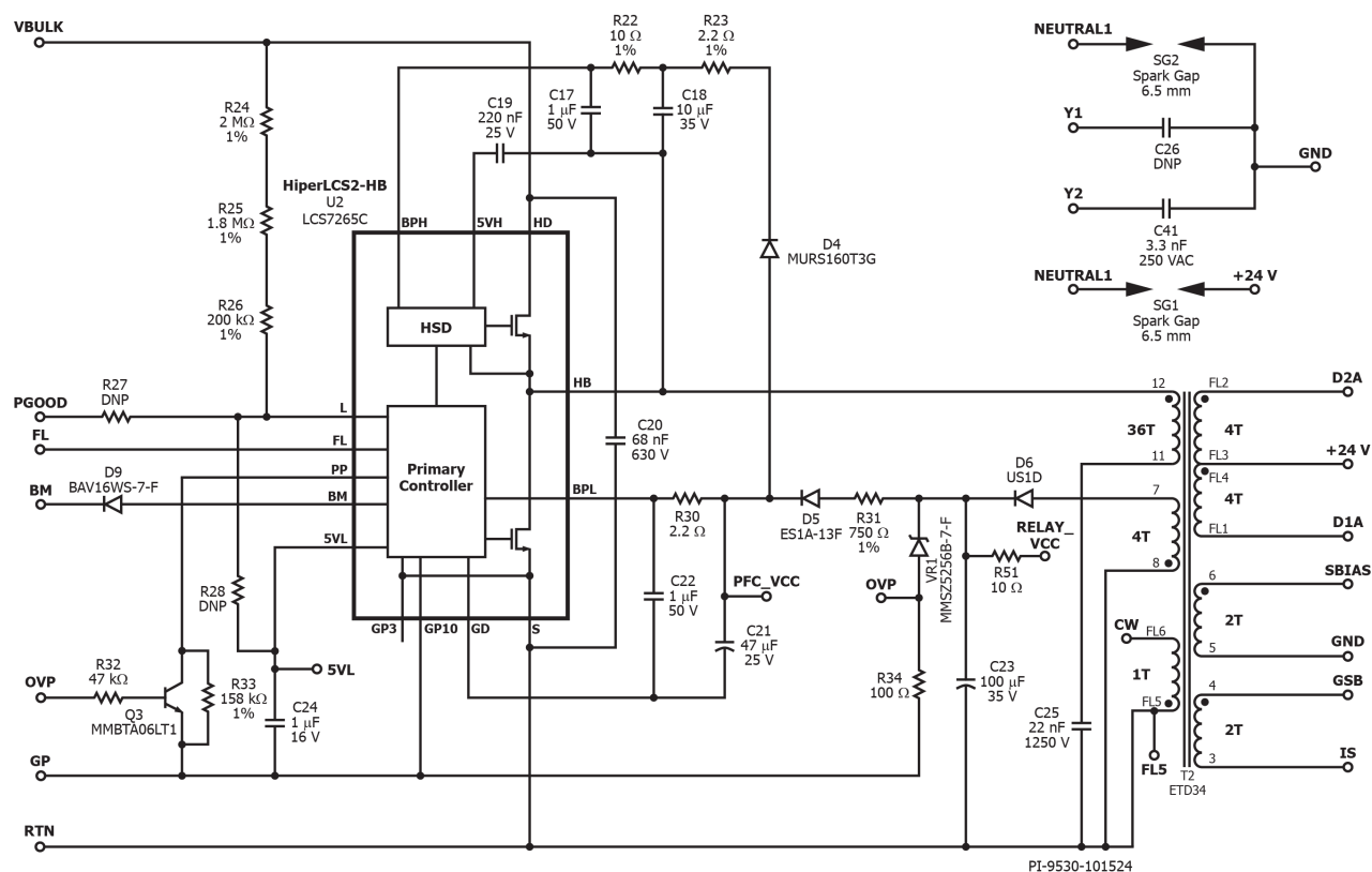
Figure 5 – LLC Stage (Primary Section) Schematic.
