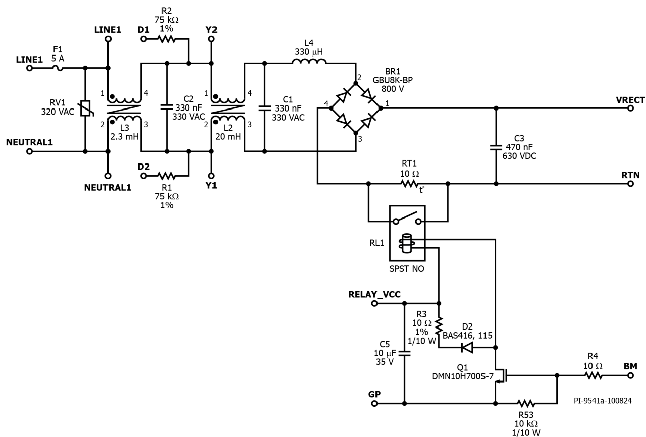
Figure 3 – Input Filter and Bridge Rectifier Schematic.
