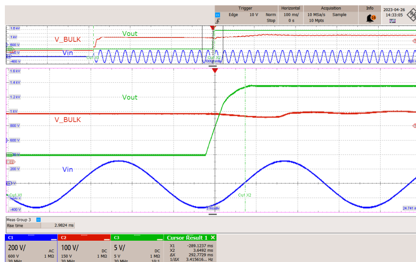
Figure 44 – Unit Start-up, 230 VAC, Full Load.
