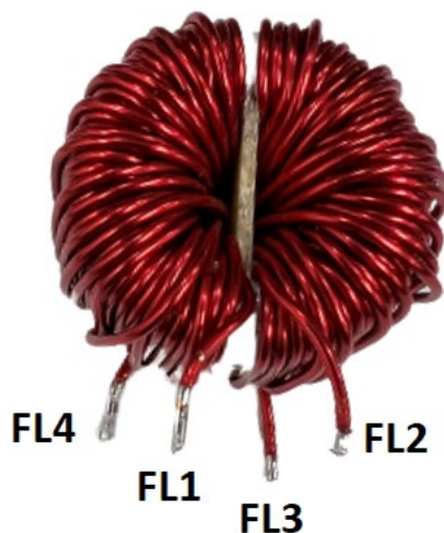
Figure 21 – Finished Inductor.
