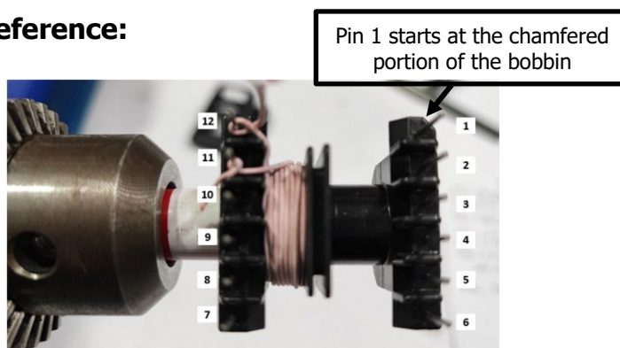
Figure 14 – LLC Transformer Bobbin Pin-out.
