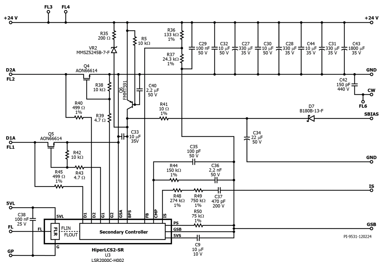
Figure 6 – LLC Stage (Secondary Section) Schematic.
