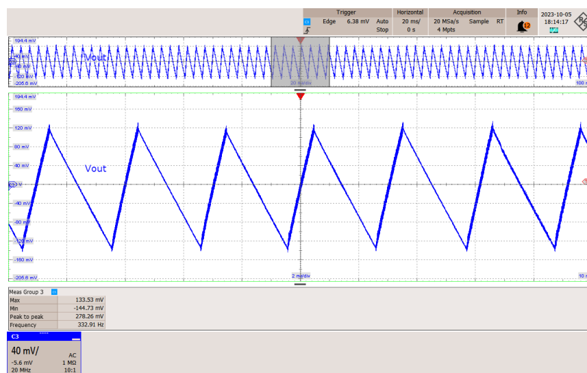
Figure 60 – Output Ripple at Light Load Condition (0.5 A), 230 VAC. Time Division: 20 ms/div. Zoom Time Division: 2 ms/div. CH3: V_{OUT} , 40 mV/div.
