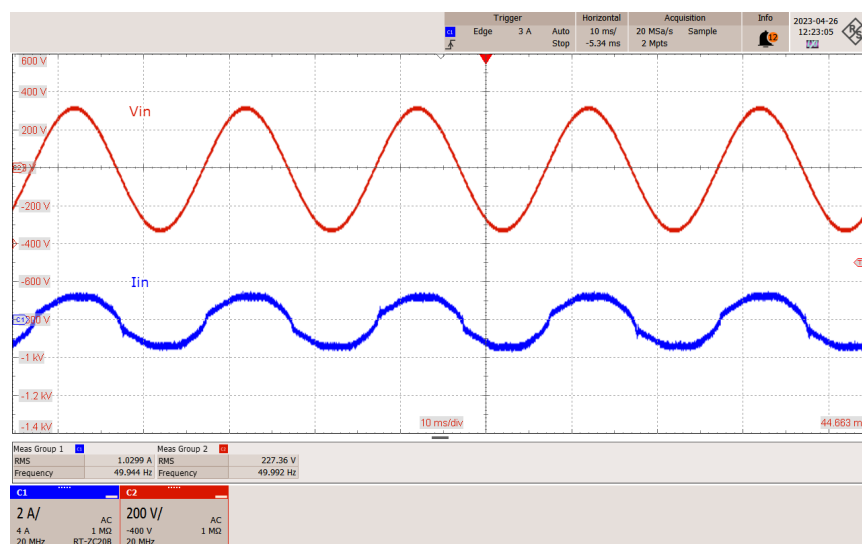
Figure 31 – Input Current, 230 VAC. 50 Hz, 10 ms/div.
