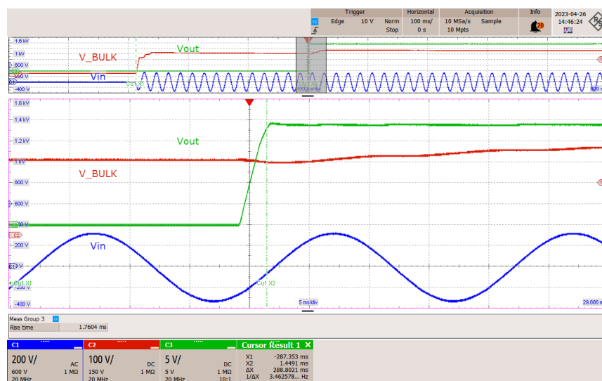
Figure 45 – Unit Start-up, 230 VAC, No Load.
