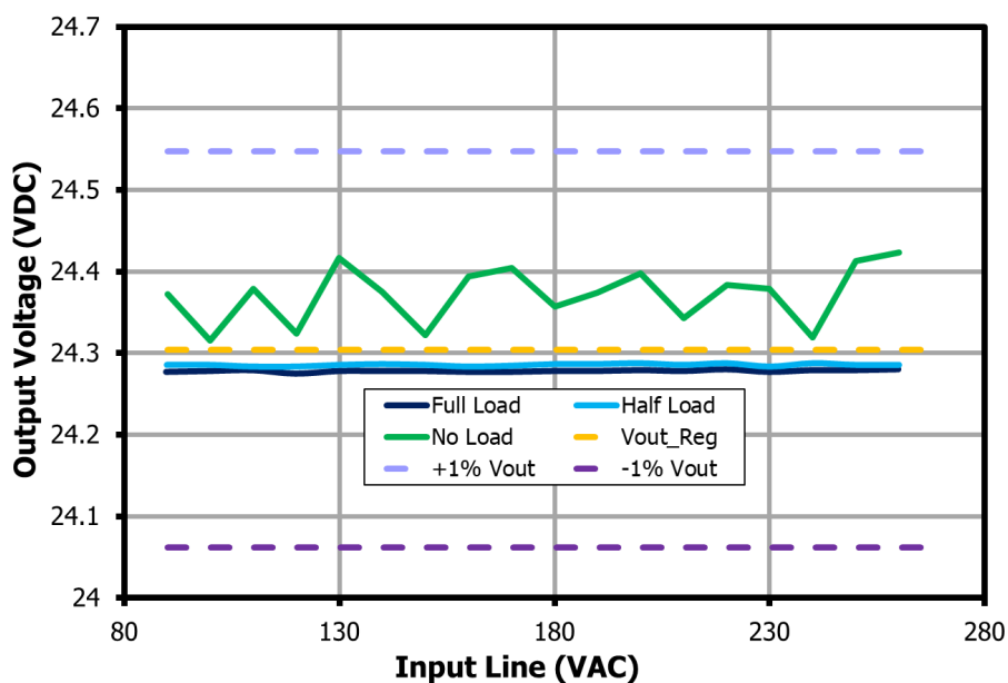
Figure 28 – Line Regulation.
