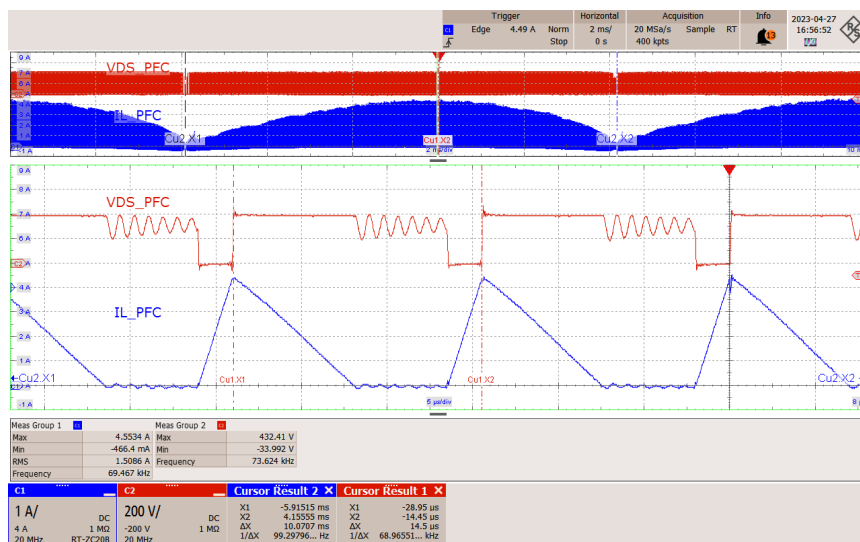
Figure 38 – VDS and Choke Current, 230 VAC.
