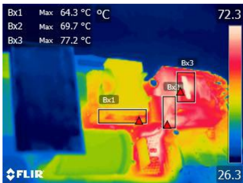
Figure 68 – Bridge Rectifier Side Thermal Picture, 100% Load, 265 VAC.
