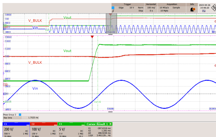
Figure 47 – Unit Start-up, 265 VAC, No Load.
