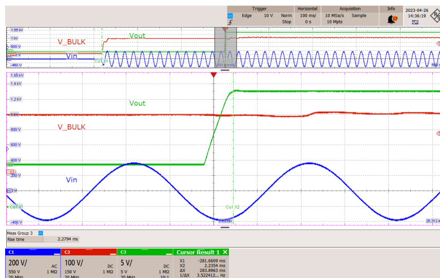
Figure 46 – Unit Start-up, 265 VAC, Full Load.
