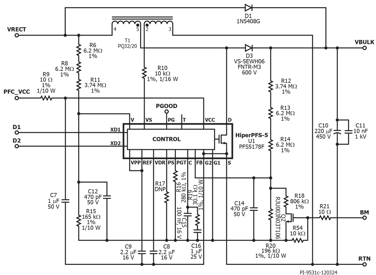
Figure 4 – PFC Stage Schematic.
