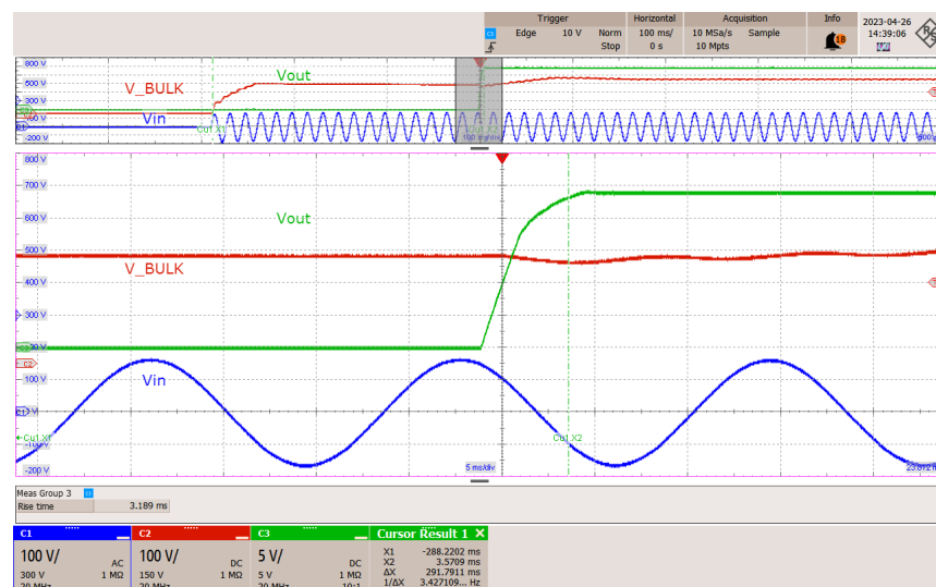
Figure 42 – Unit Start-up, 115 VAC, Full Load.
