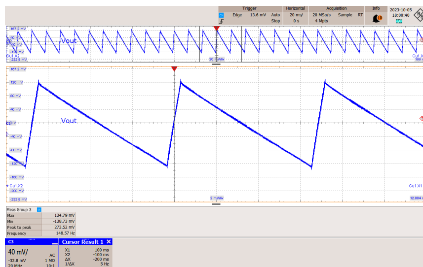
Figure 61 – Output Ripple at Light Load Condition (0.3 A), 230 VAC.
