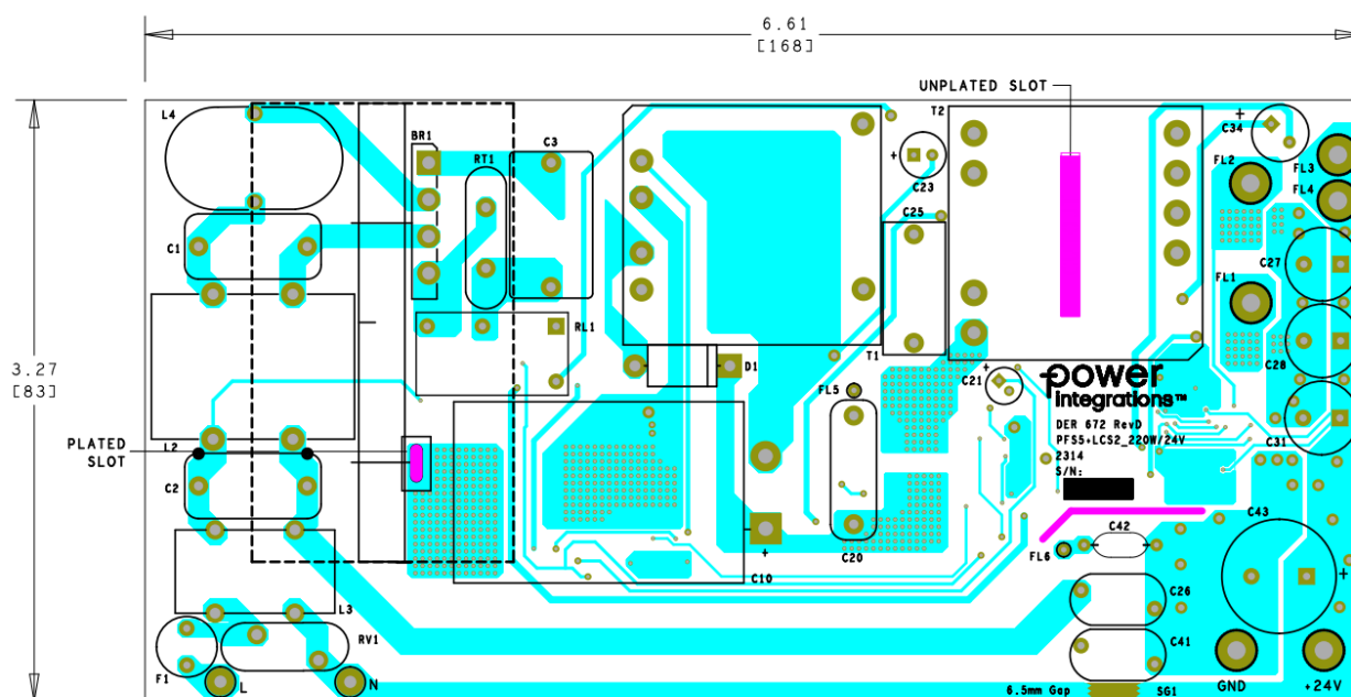
Figure 7 – Top Side PCB.
