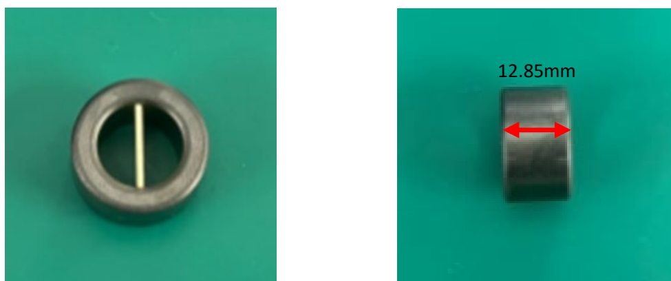
Figure 18 – Core Preparation.
