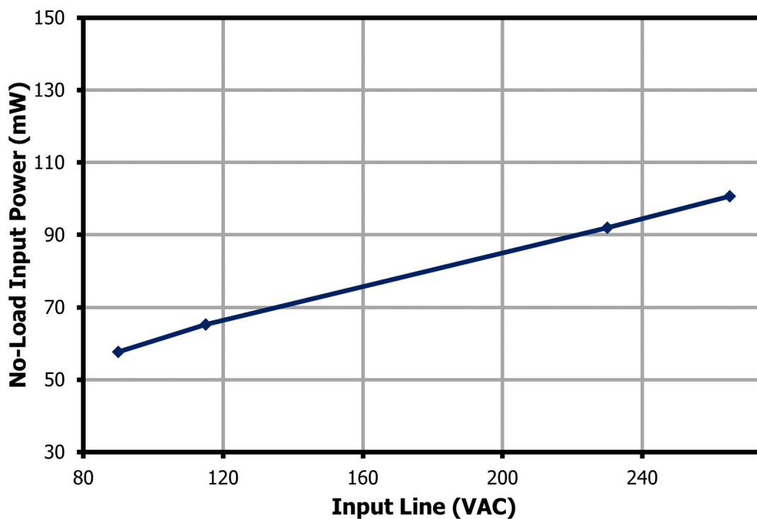
Figure 25 – No-Load Input Power vs. Input Voltage.
