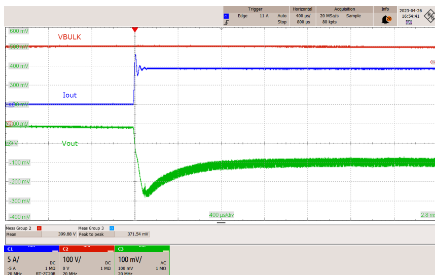
Figure 52 – Dynamic Loading, 115 VAC, 0-100% Load.
