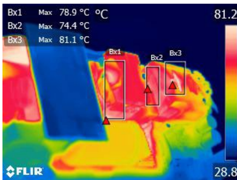
Figure 64 – Bridge Rectifier Side Thermal Picture, 100% Load, 90 VAC.
