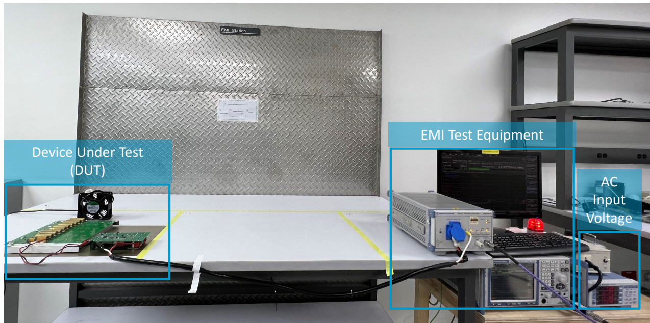
Figure 71 – EMI Test Set-up
