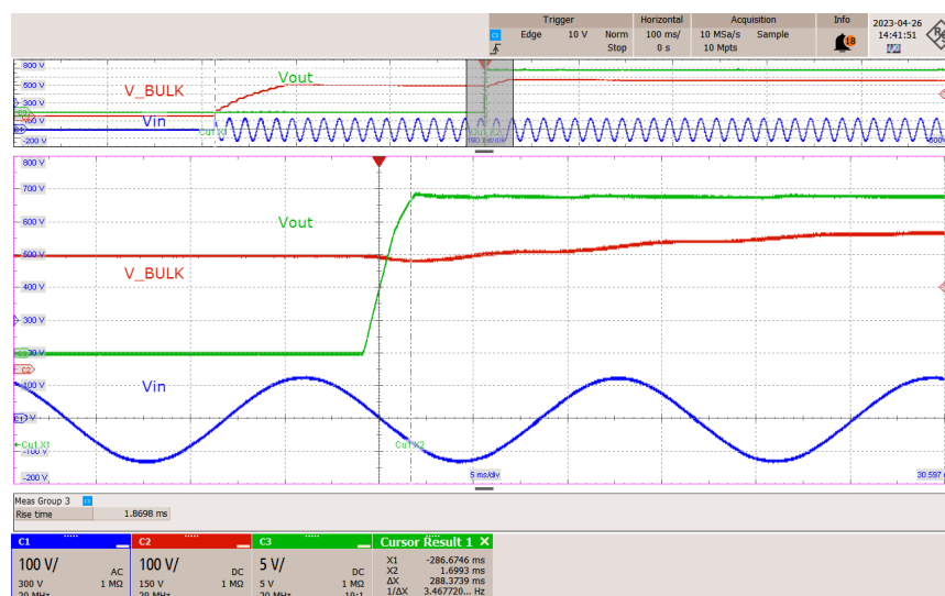
Figure 41 – Unit Start-up, 90 VAC, No Load.
