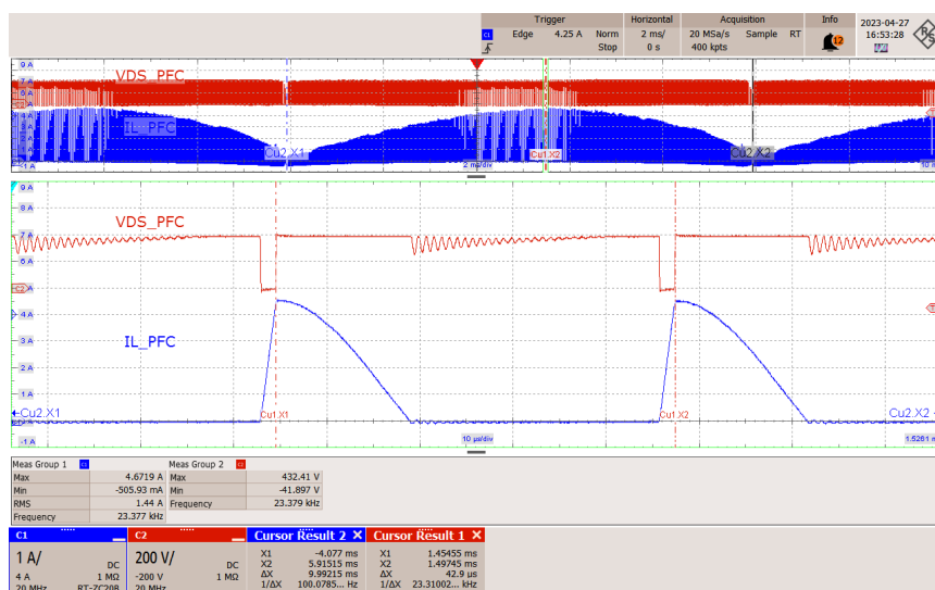
Figure 39 – VDS and Choke Current, 265 VAC.
