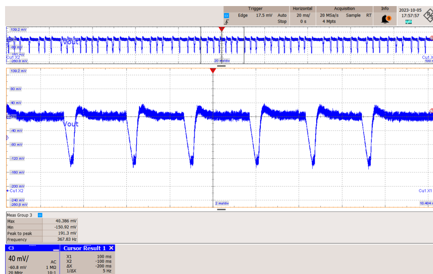
Figure 59 – Output Ripple at Light Load Condition (2.0 A), 230 VAC. Time Division: 20 ms/div. Zoom Time Division: 2 ms/div. CH3: V_{OUT} , 40 mV/div.
