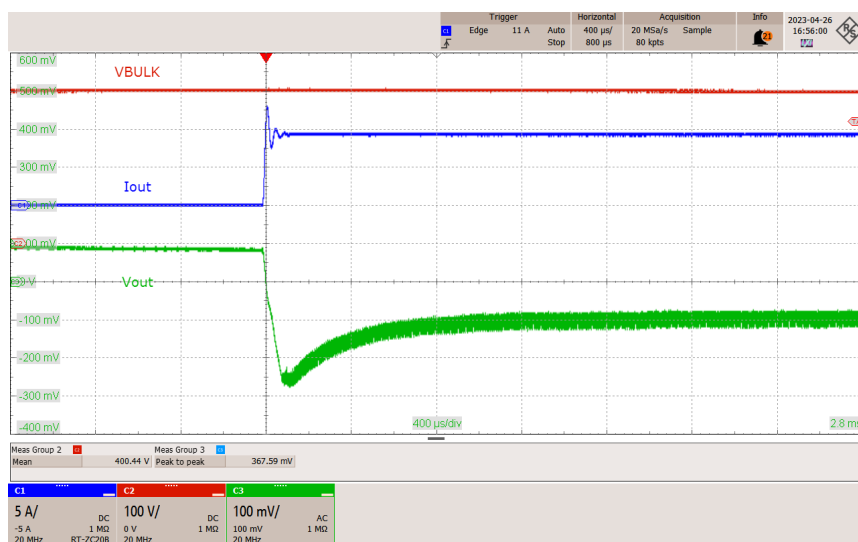
Figure 54 – Dynamic Loading, 230 VAC, 0-100% Load.
