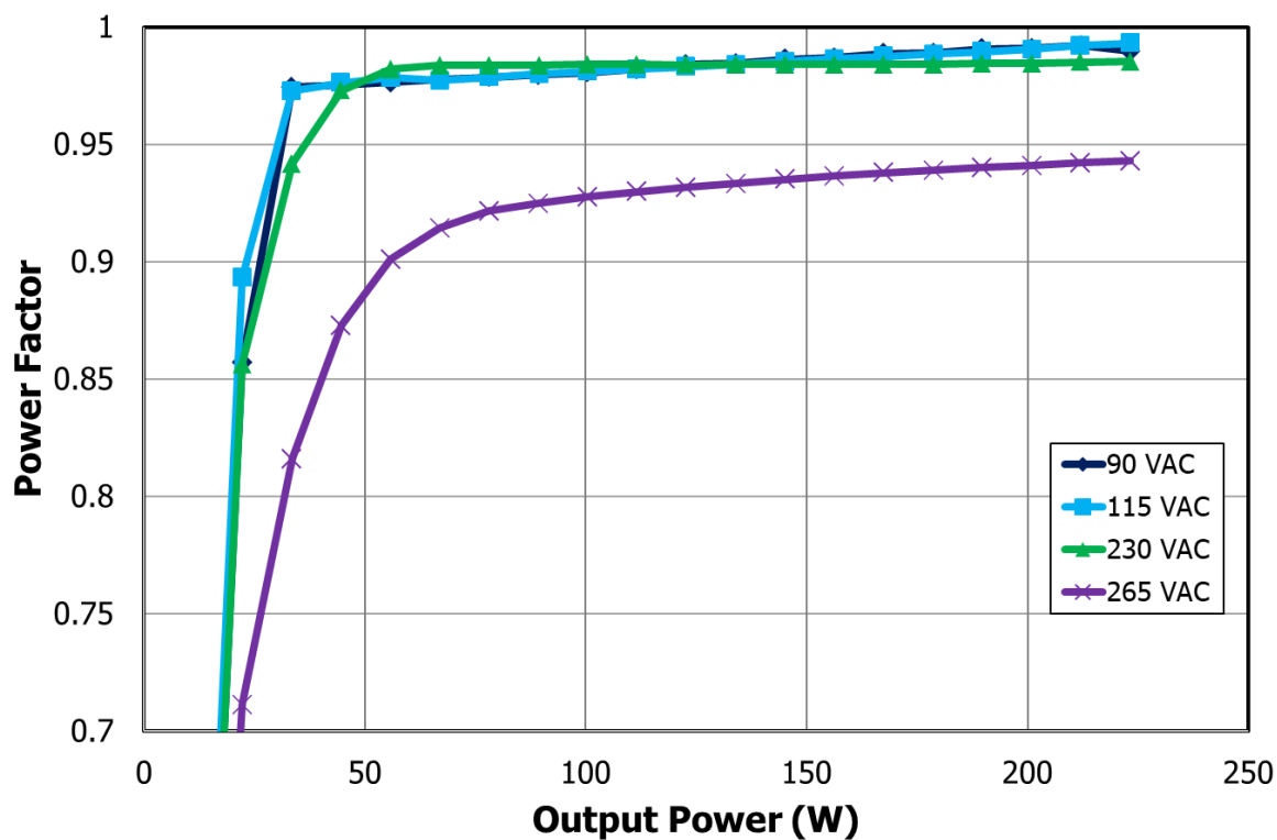
Figure 26 – Power Factor vs. Output Power.
