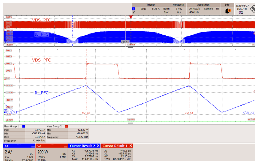
Figure 36 – VDS and Choke Current, 90 VAC.
