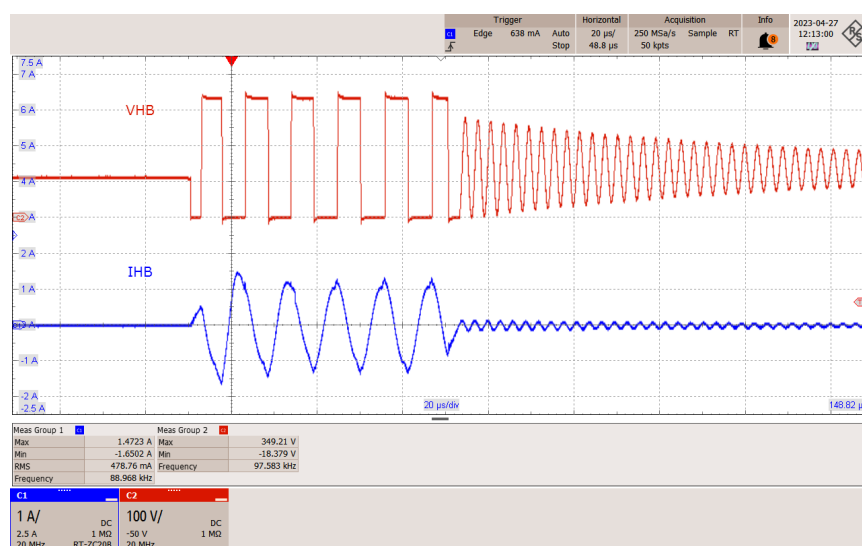
Figure 34 – LLC Stage Primary Voltage and Current, No-Load.
