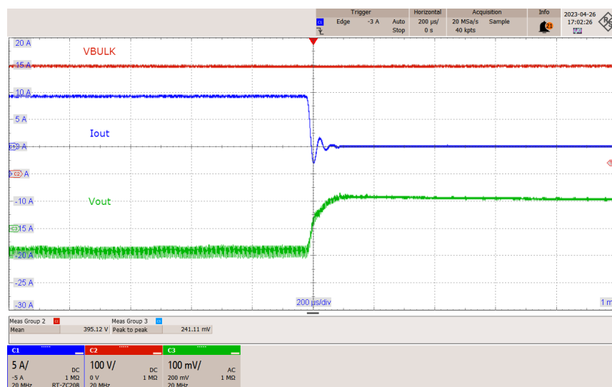
Figure 55 – Dynamic Loading, 230 VAC, 100-0% Load.
