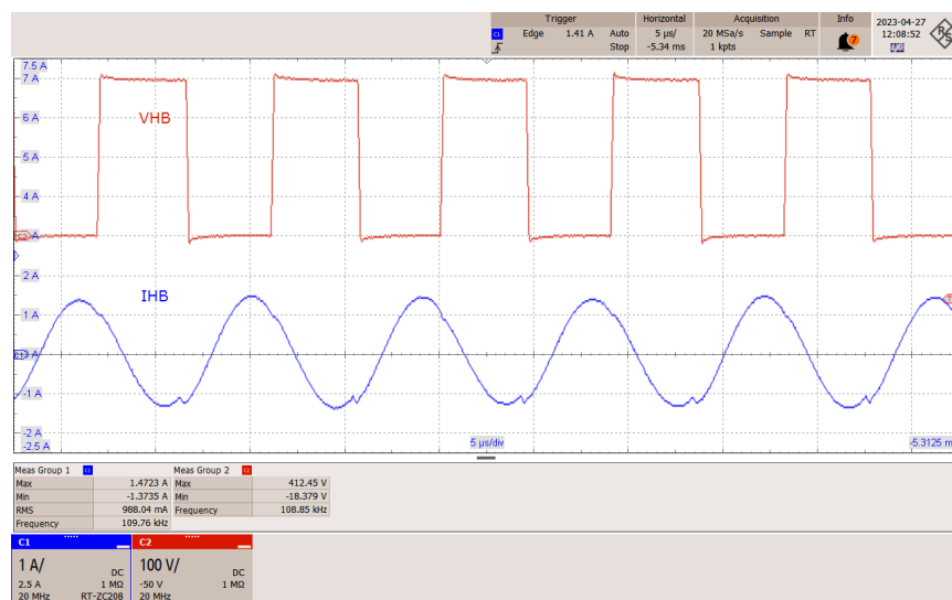
Figure 33 – LLC Stage Primary Voltage and Current, 50% Load.
