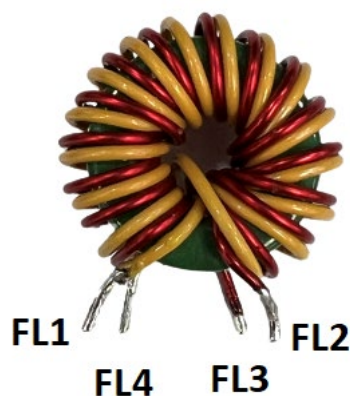
Figure 16 – Finished Inductor.
