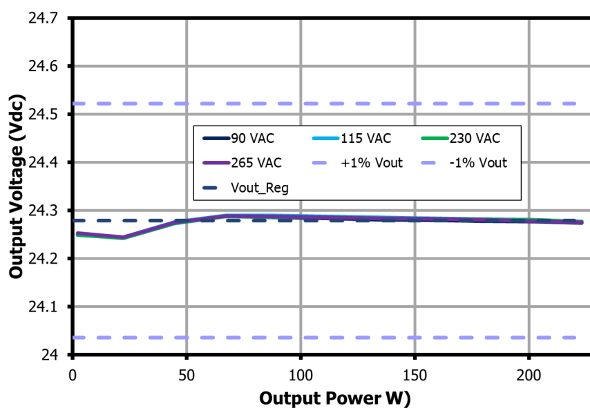
Figure 29 – Load Regulation.
