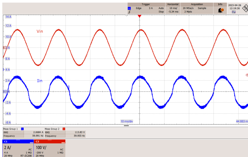
Figure 30 – Input Current, 115 VAC. 60 Hz, 10 ms/div. CH1: I_{IN} , 2 A/div. CH2: V_{IN} , 100 V/div.
