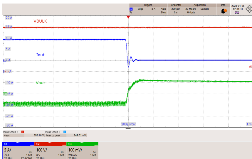
Figure 53 – Dynamic Loading, 115 VAC, 100-0% Load.
