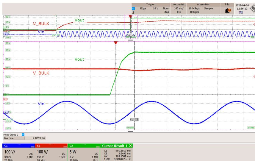
Figure 40 – Unit Start-up, 90 VAC, Full Load.
