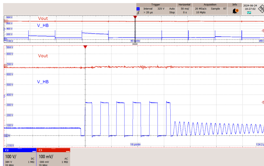
Figure 51 – Burst Operation During No Load Condition, 230 VAC.
