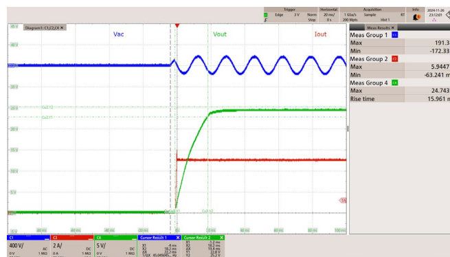
Figure 28 – 115 VAC 60 Hz.
