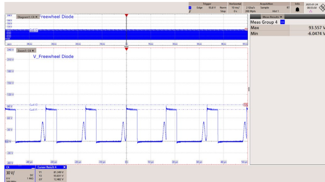
Figure 61 – 230 VAC 50 Hz.
