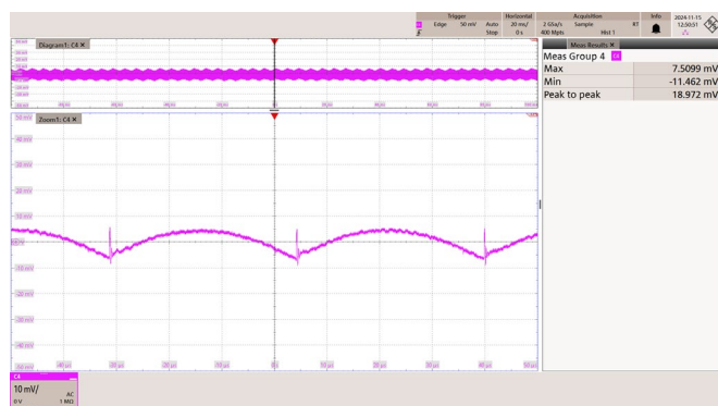
Figure 88 – 265 VAC 50 Hz.
