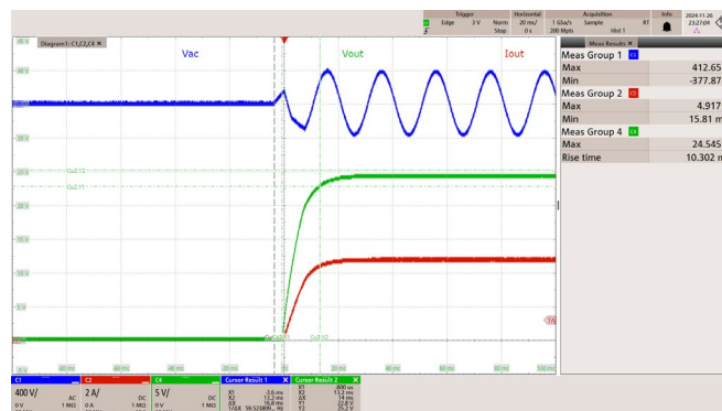
Figure 34 – 265 VAC 50 Hz.
