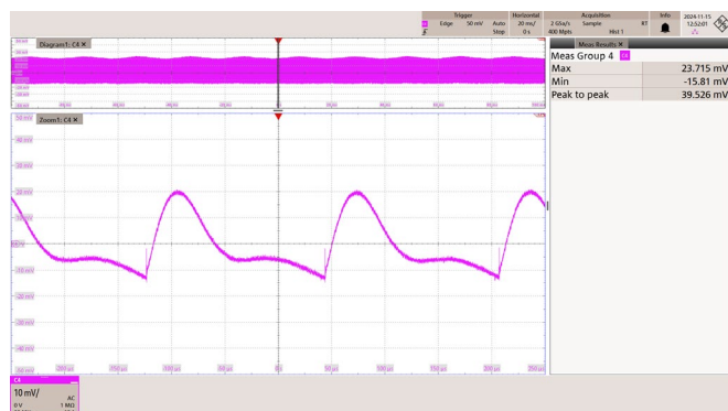
Figure 96 – 265 VAC 50 Hz.
