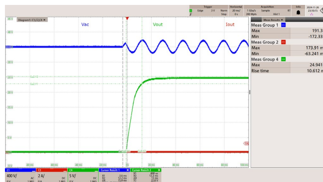
Figure 36 – 115 VAC 60 Hz.
