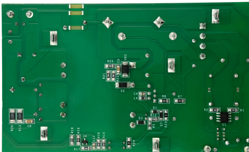
Figure 2 –Bottom View.
