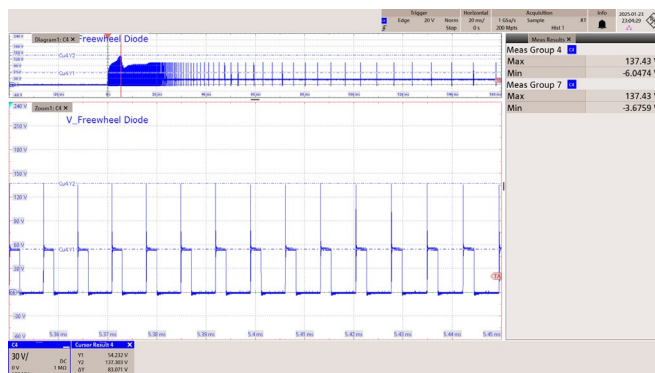
Figure 74 – 265 VAC 50 Hz.
