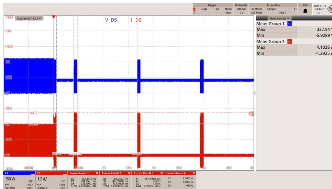
Figure 104 – 85 VAC 60 Hz. Output Short.
