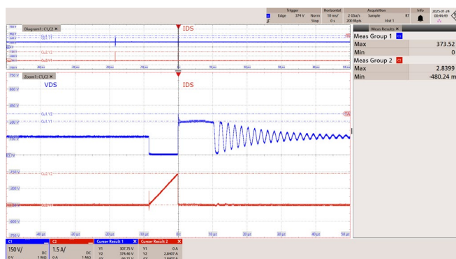
Figure 48 – 115 VAC 60 Hz.
