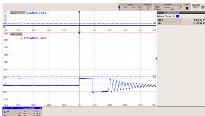
Figure 64 – 115 VAC 60 Hz.
