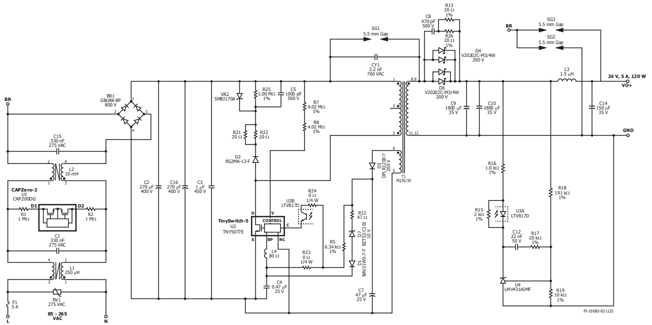
Figure 4 – DER-1027 Schematic
