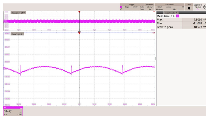
Figure 87 – 230 VAC 50 Hz.
