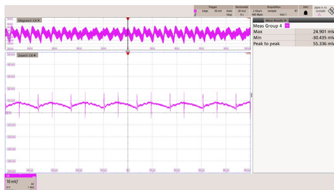
Figure 77 – 85 VAC 60 Hz.
