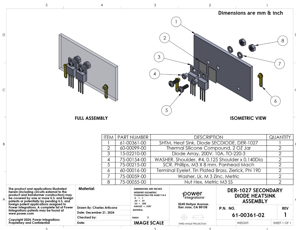
Figure 19 – DER-1027 Secondary Diode Heat Sink Assembly.
