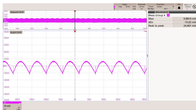
Figure 90 – 115 VAC 60 Hz.
