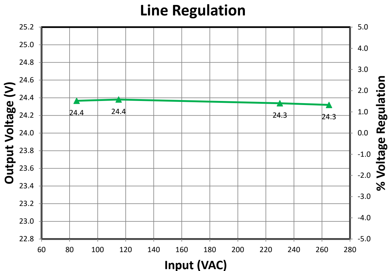
Figure 21 – Output Voltage vs. Line Voltage.
