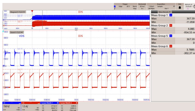
Figure 52 – 115 VAC 60 Hz.
