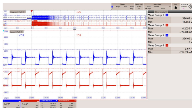
Figure 55 – 85 VAC 60 Hz.
