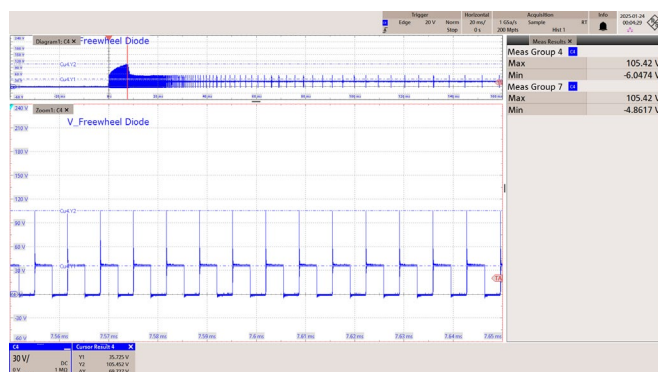
Figure 71 – 85 VAC 60 Hz.
