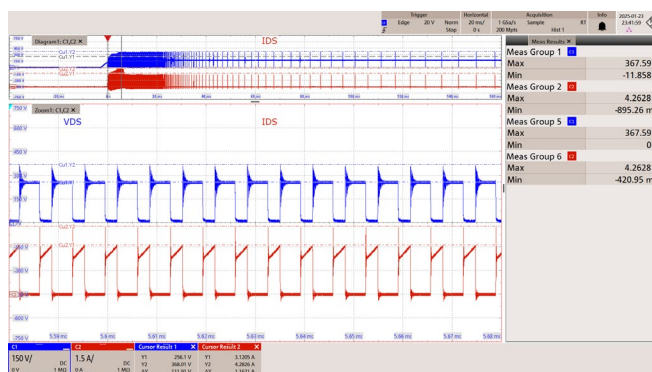
Figure 56 – 115 VAC 60 Hz.
