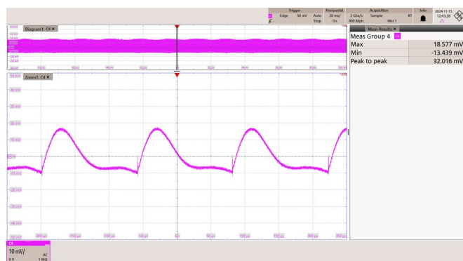
Figure 94 – 115 VAC 60 Hz.
