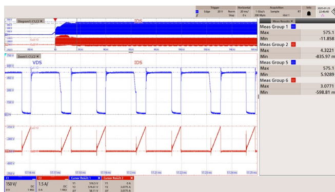
Figure 54 – 265 VAC 50 Hz.
