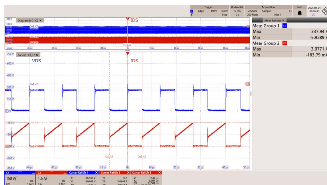
Figure 43 – 85 VAC 60 Hz.
