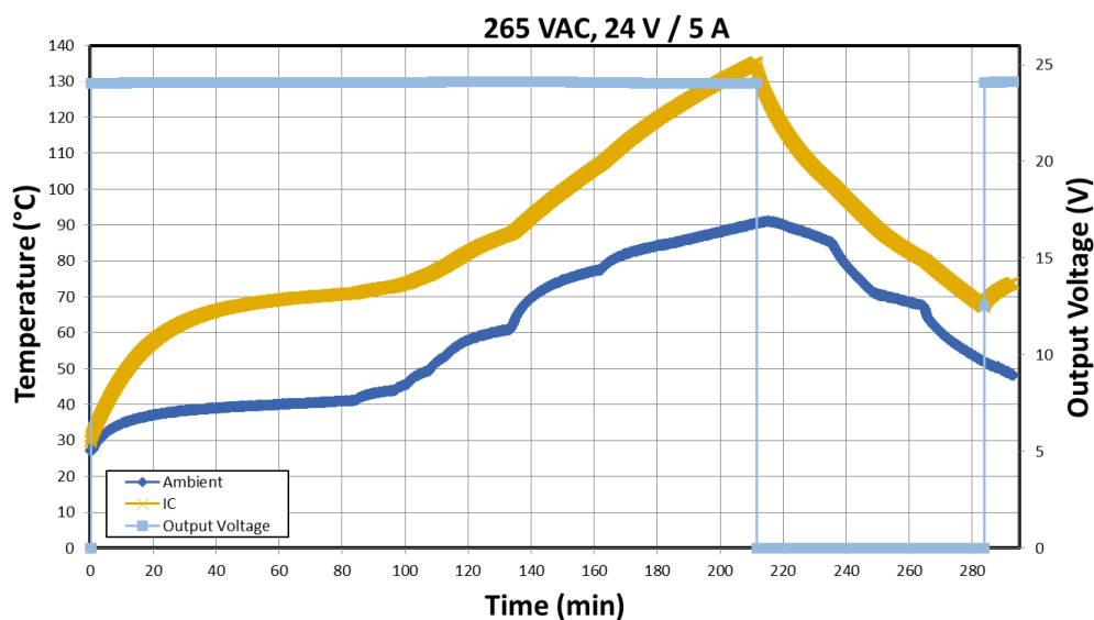
Figure 109 – 265 VAC, I_o = 5 A (100% load)
