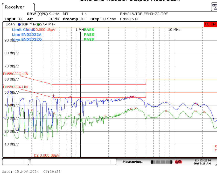
Figure 112 – 230 VAC 60 Hz. Line and Neutral Output Float Scan
