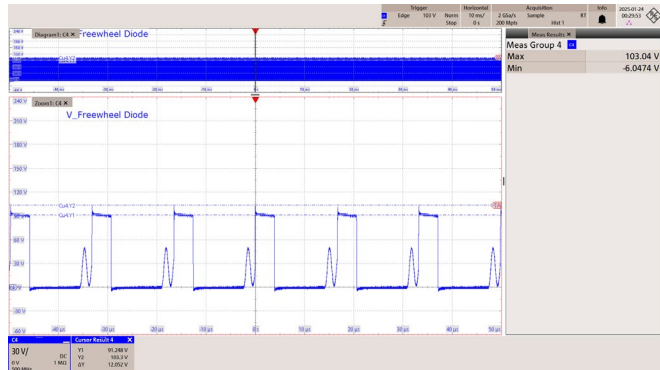
Figure 62 – 265 VAC 50 Hz.
