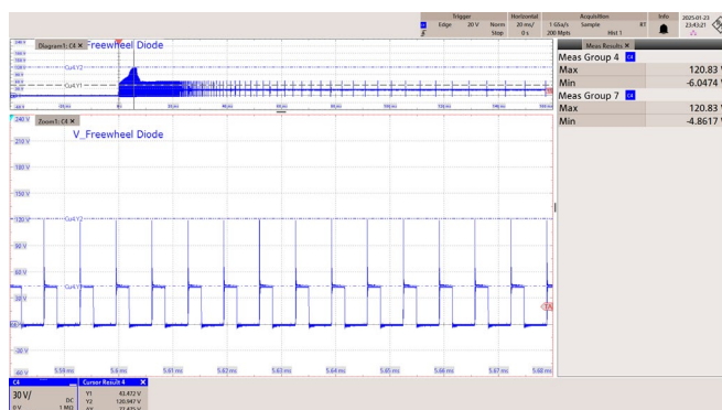
Figure 72 – 115 VAC 60 Hz.
