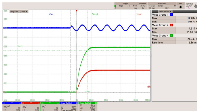
Figure 31 – 85 VAC 60 Hz.
