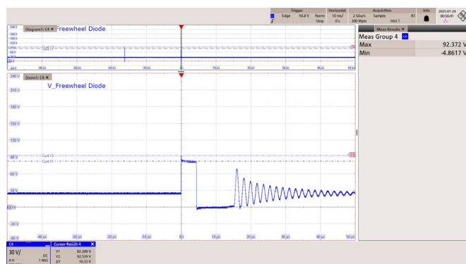
Figure 65 – 230 VAC 50 Hz.
