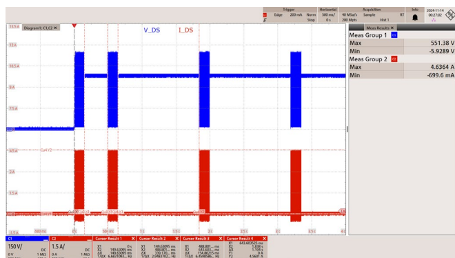
Figure 103 – 265 VAC 50 Hz Output Short.
