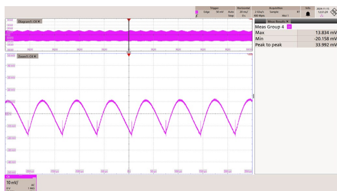
Figure 92 – 265 VAC 50 Hz.
