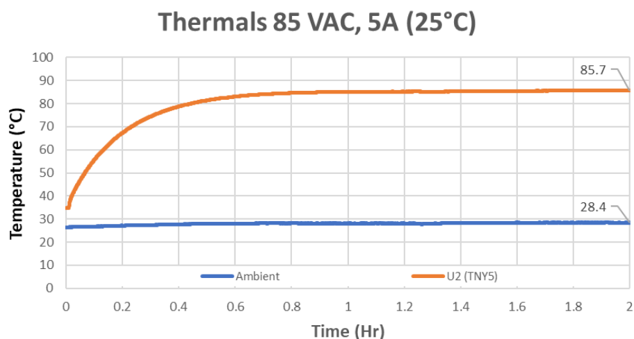
Figure 98 – 85 VAC 60 Hz. TNY5077E Thermals.
