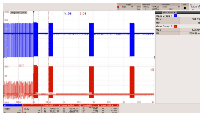
Figure 107 – 265 VAC 50 Hz. Output Short.
