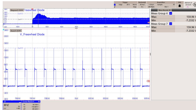
Figure 69 – 230 VAC 50 Hz.
