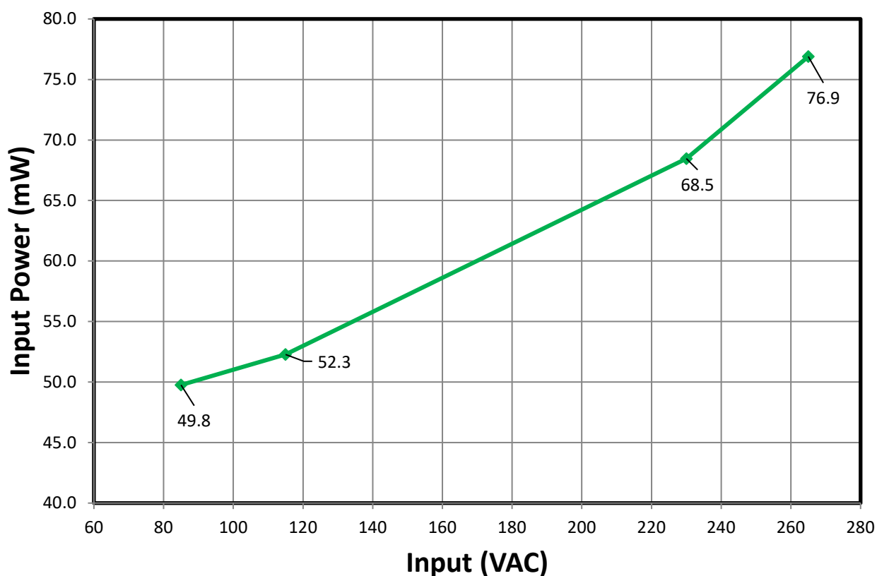
Figure 24 – No-Load Input Power vs. Line at Room Temperature.
