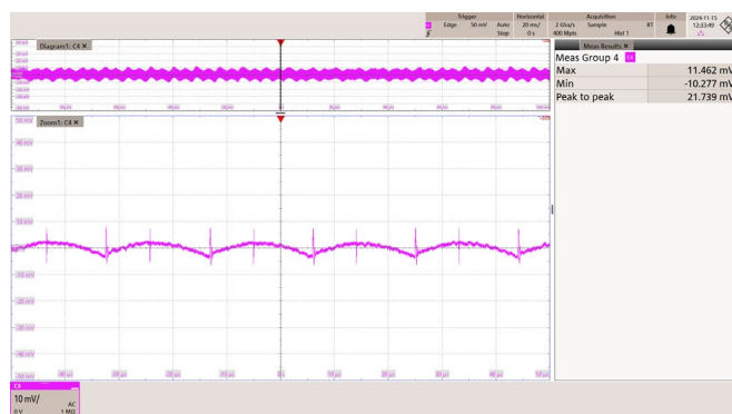
Figure 81 – 85 VAC 60 Hz.
