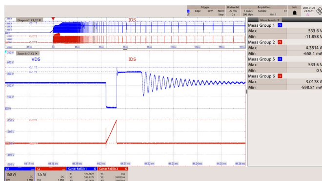
Figure 57 – 230 VAC 50 Hz.
