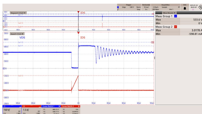
Figure 49 – 230 VAC 50 Hz.
