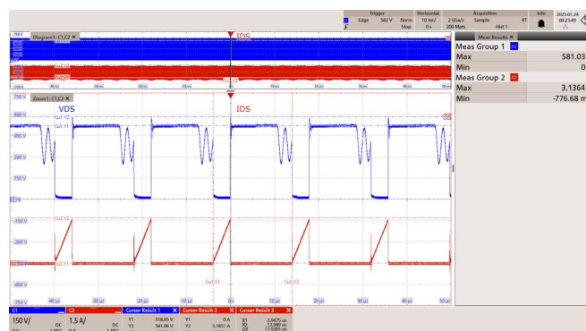
Figure 46 – 265 VAC 50 Hz.
