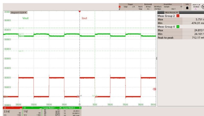
Figure 39 – 85 VAC 60 Hz.
