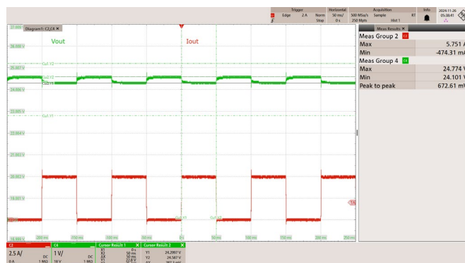
Figure 41 – 230 VAC 50 Hz.
