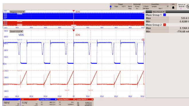
Figure 45 – 230 VAC 50 Hz.
