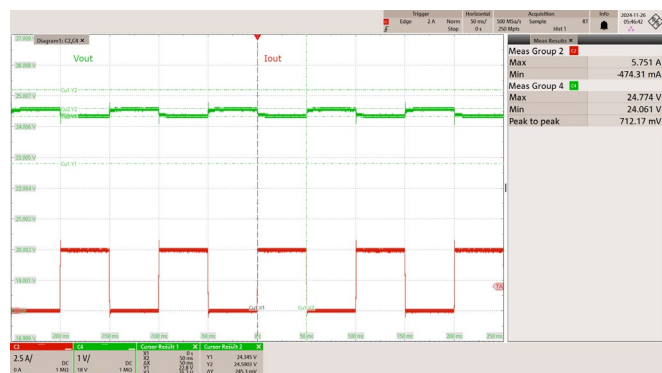
Figure 40 – 115 VAC 60 Hz.
