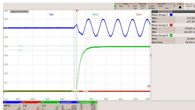
Figure 38 – 265 VAC 50 Hz.
