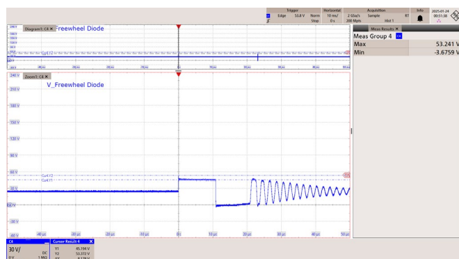
Figure 63 – 85 VAC 60 Hz.
