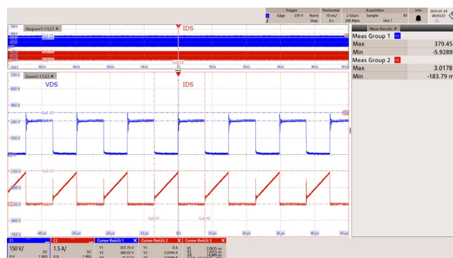
Figure 44 – 115 VAC 60 Hz.
