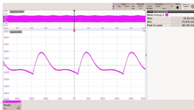
Figure 95 – 230 VAC 50 Hz.
