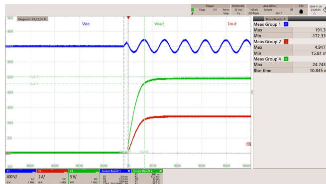
Figure 32 – 115 VAC 60 Hz.
