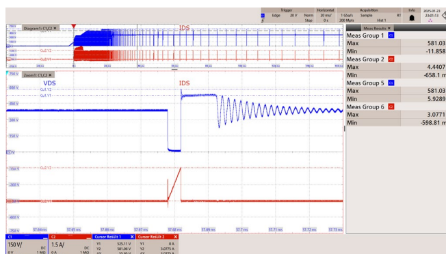
Figure 58 – 265 VAC 50 Hz.
