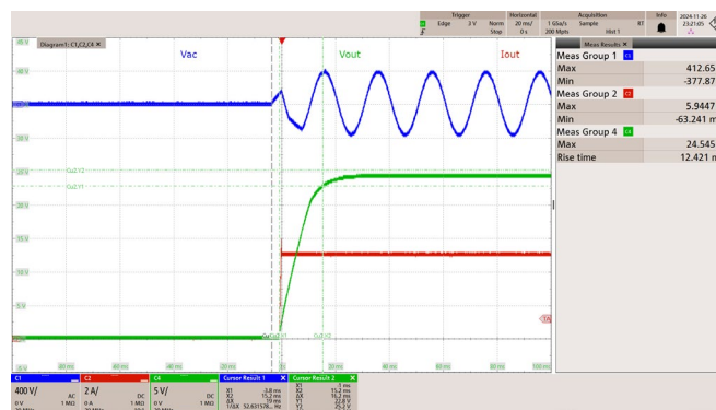
Figure 30 – 265 VAC 50 Hz.
