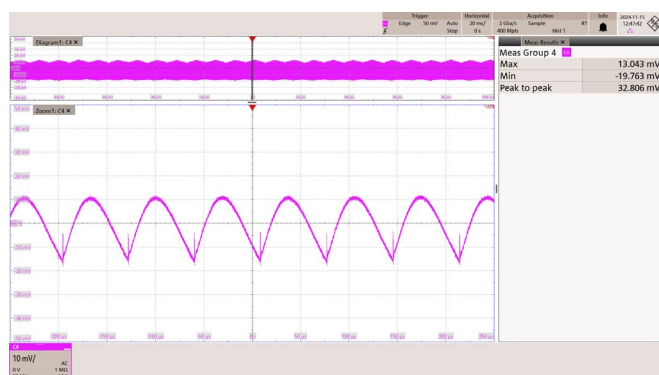
Figure 91 – 230 VAC 50 Hz.
