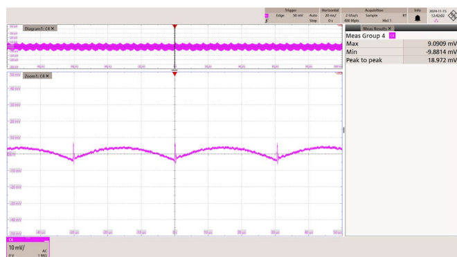
Figure 86 – 115 VAC 60 Hz.
