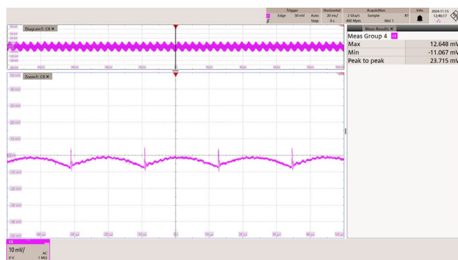
Figure 83 – 230 VAC 50 Hz.
