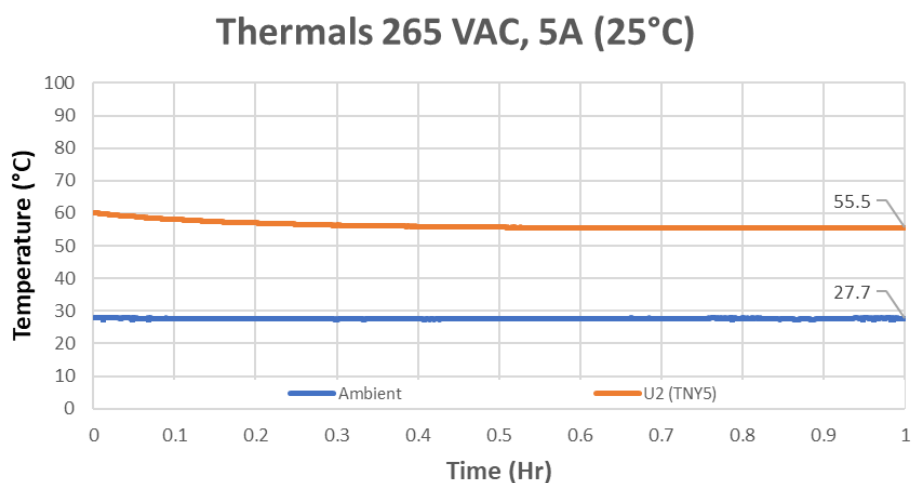
Figure 100 – 265 VAC 50 Hz. TNY5077E Thermals.
