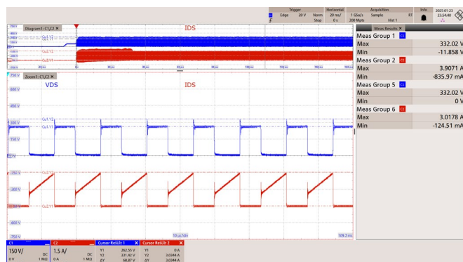
Figure 51 – 85 VAC 60 Hz.
