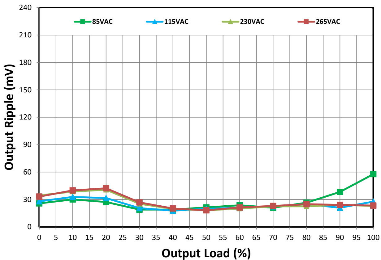
Figure 97 – Voltage Ripple (Measured at PCB End at Room Temperature).
