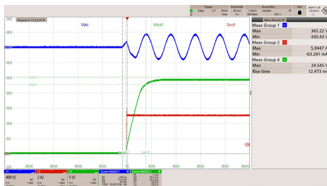
Figure 29 – 230 VAC 50 Hz.
