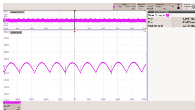
Figure 89 – 85 VAC 60 Hz.
