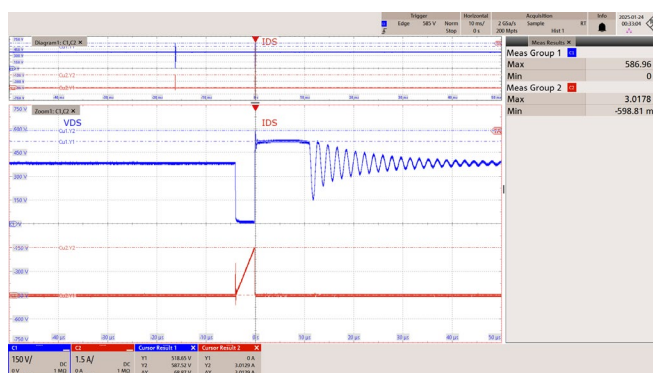
Figure 50 – 265 VAC 50 Hz.
