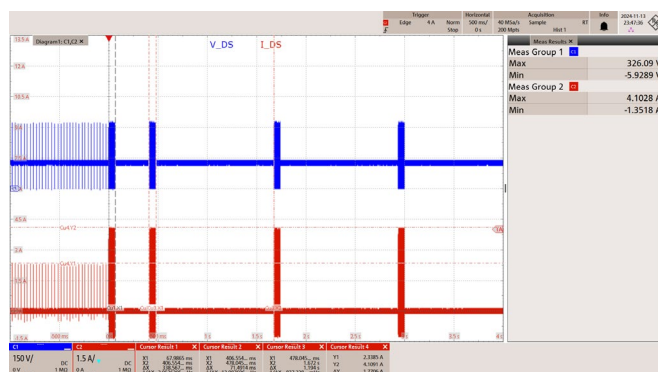
Figure 106 – 85 VAC 60 Hz. Output Short.
