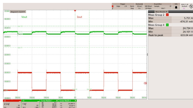
Figure 42 – 265 VAC 50 Hz.
