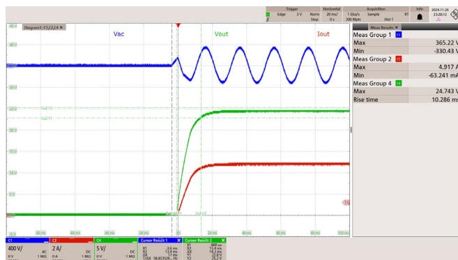
Figure 33 – 230 VAC 50 Hz.
