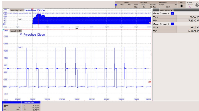
Figure 70 – 265 VAC 50 Hz.
