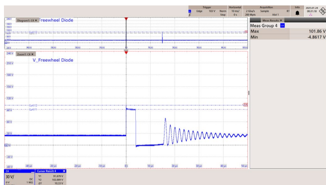
Figure 66 – 265 VAC 50 Hz.
