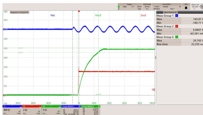
Figure 27 – 85 VAC 60 Hz.
