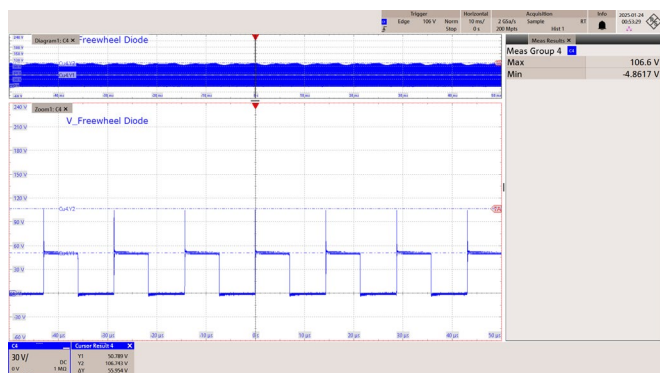
Figure 60 – 115 VAC 60 Hz.
