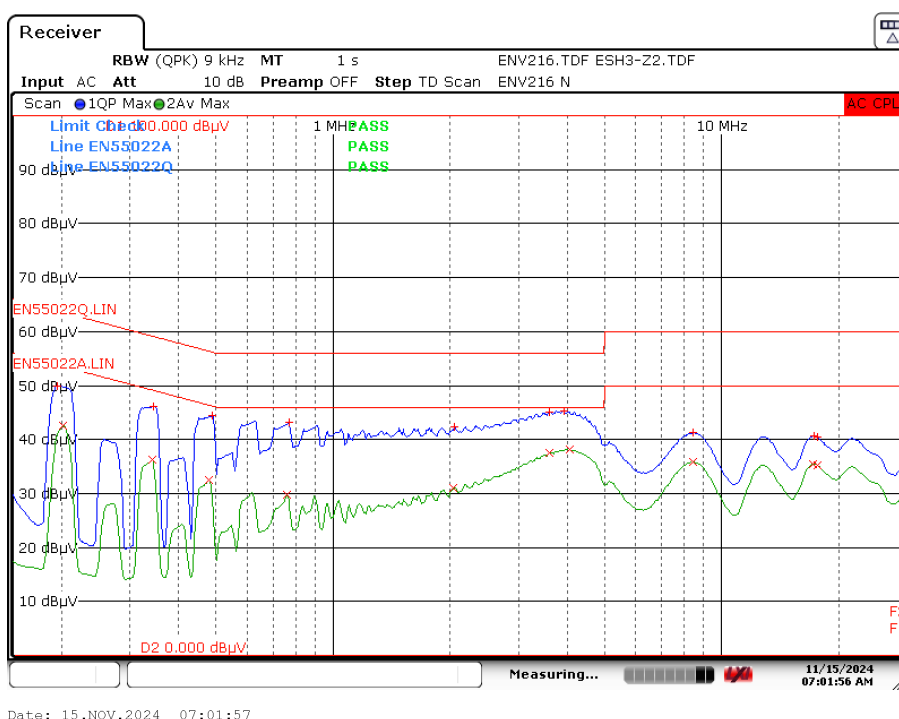
Figure 111 – 115 VAC 60 Hz. Line and Neutral Output Float Scan
