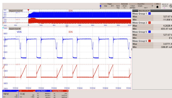
Figure 53 – 230 VAC 50 Hz.
