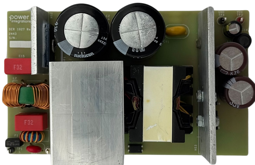
Figure 1 –Top View.
