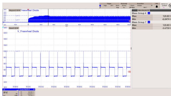
Figure 67 – 85 VAC 60 Hz.
