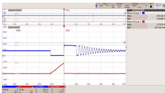
Figure 47 – 85 VAC 60 Hz.
