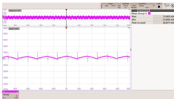
Figure 78 – 115 VAC 60 Hz.
