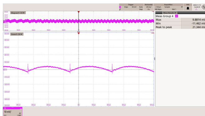
Figure 85 – 85 VAC 60 Hz.
