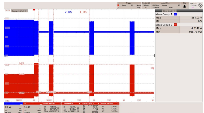
Figure 105 – 265 VAC 50 Hz. Output Short.
