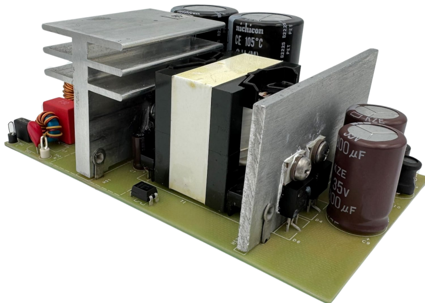
Figure 3 – Oblique View.
