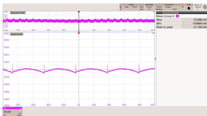
Figure 82 – 115 VAC 60 Hz.
