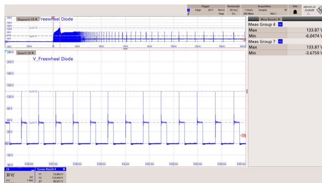
Figure 73 – 230 VAC 50 Hz.
