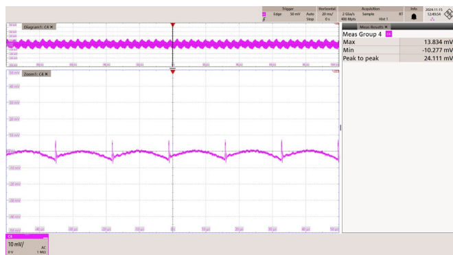
Figure 80 – 265 VAC 50 Hz.
