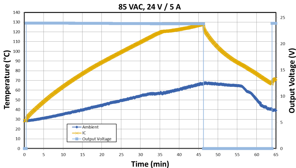
Figure 108 – 85 VAC, I_o = 5 A (100% load)
