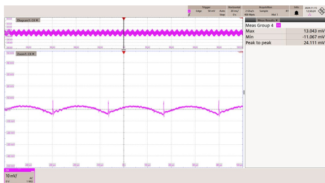
Figure 84 – 265 VAC 50 Hz.
