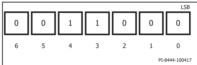
Figure 1. Slave Address.
