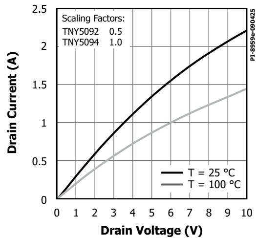
Figure 20. Output Characteristics.
