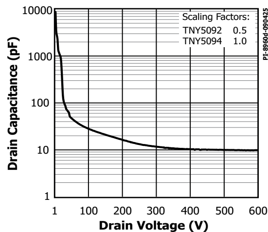
Figure 21. COSS vs. Drain Voltage.
