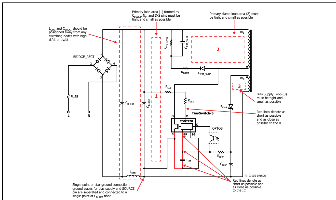
Figure 8. Typical Schematic of TinySwitch-5 Primary-Side Showing Critical Loops Areas, Critical Component Traces, and Single-Point or Star Grounding.
