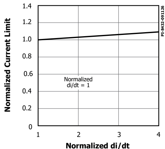
Figure 24. I_{LM} vs. di/dt
