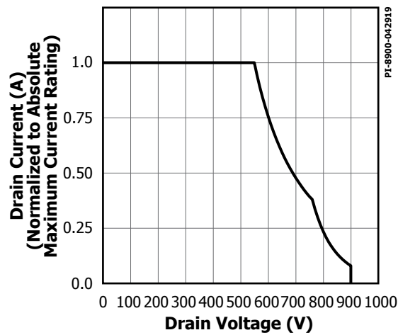
Figure 19. Maximum Allowable Drain Current vs. Drain Voltage (TNY5092K and TNY5094K)
