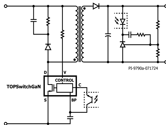
Figure 1. Typical Flyback Schematic.
