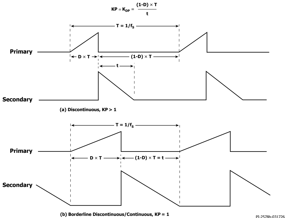
Figure 13. Discontinuous Conduction Mode Current Waveform, KP > 1 .
