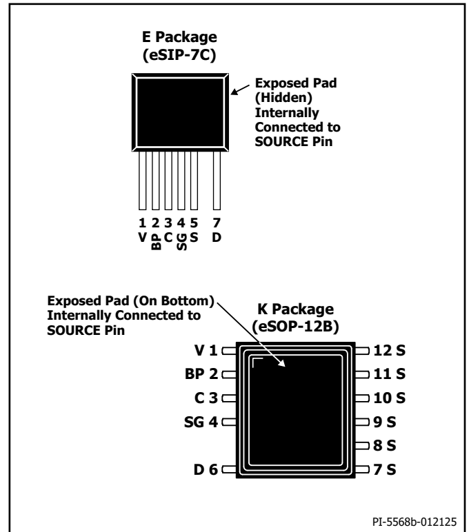
Figure 4. Pin Configuration (Top View).
