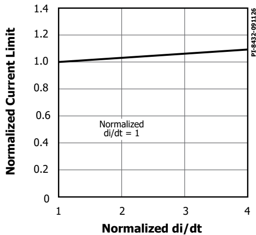
Figure 18. I_{LIM} vs. di/dt
