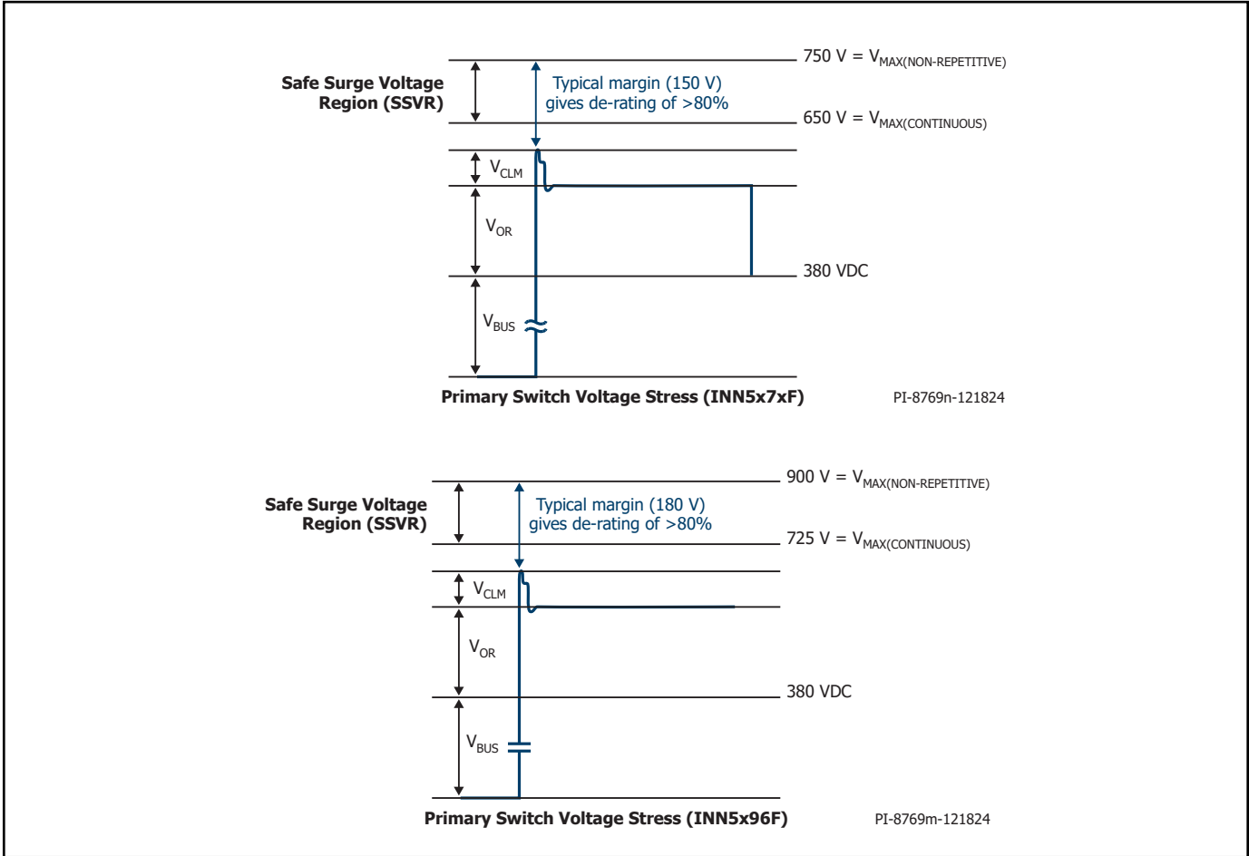
Figure 37. Peak Drain Voltage for 264 VAC Input Voltage.
