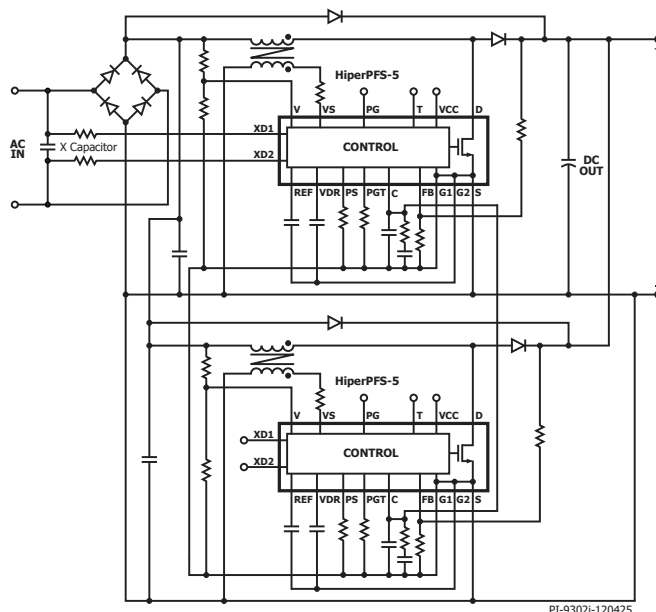
Figure 4. Compensation Pin Connection for Parallel Operation.
