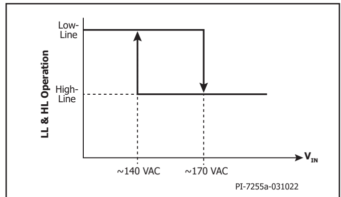
Figure 13. Boost Follower Low-Line and High-Line operation vs. Input Voltage.
