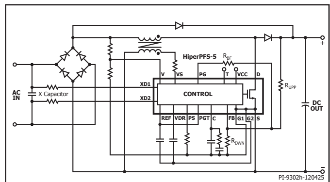
Figure 14. System Schematic with a Line Dependent V_{OUT} (Boost Follower).
