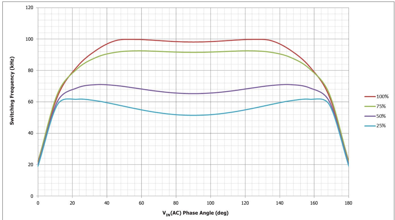
Figure 9. Frequency Variation Over Line Half-Cycle as a Function of Input Voltage.
