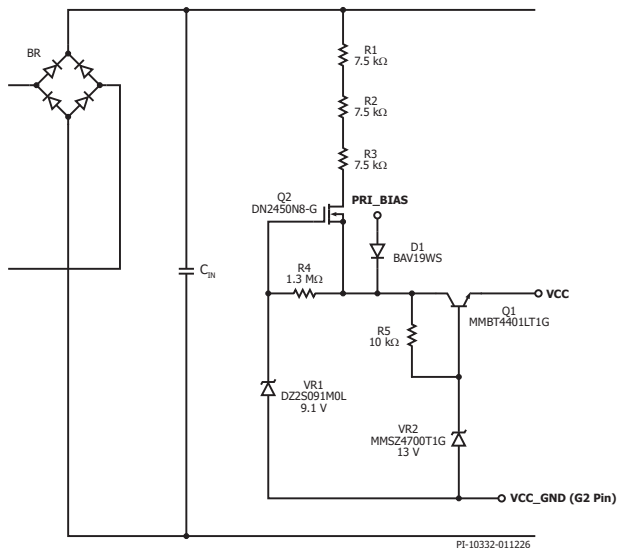
Figure 7. Minimum Recommended High Voltage Bias Start-Up Supply Circuit for HiperPFS-5.
