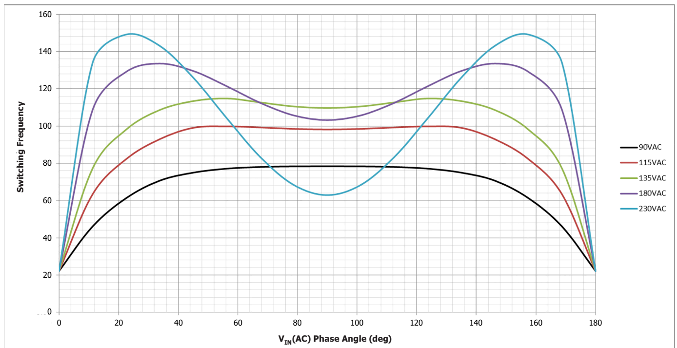
Figure 10. Frequency Variation Over Line Half-Cycle as a Function of load ( V_{IN} = 115 \text{ VAC} ).
