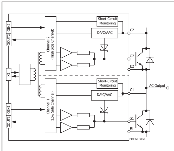
Figure 4. Functional Block Diagram of 2SP0430V2xxC
