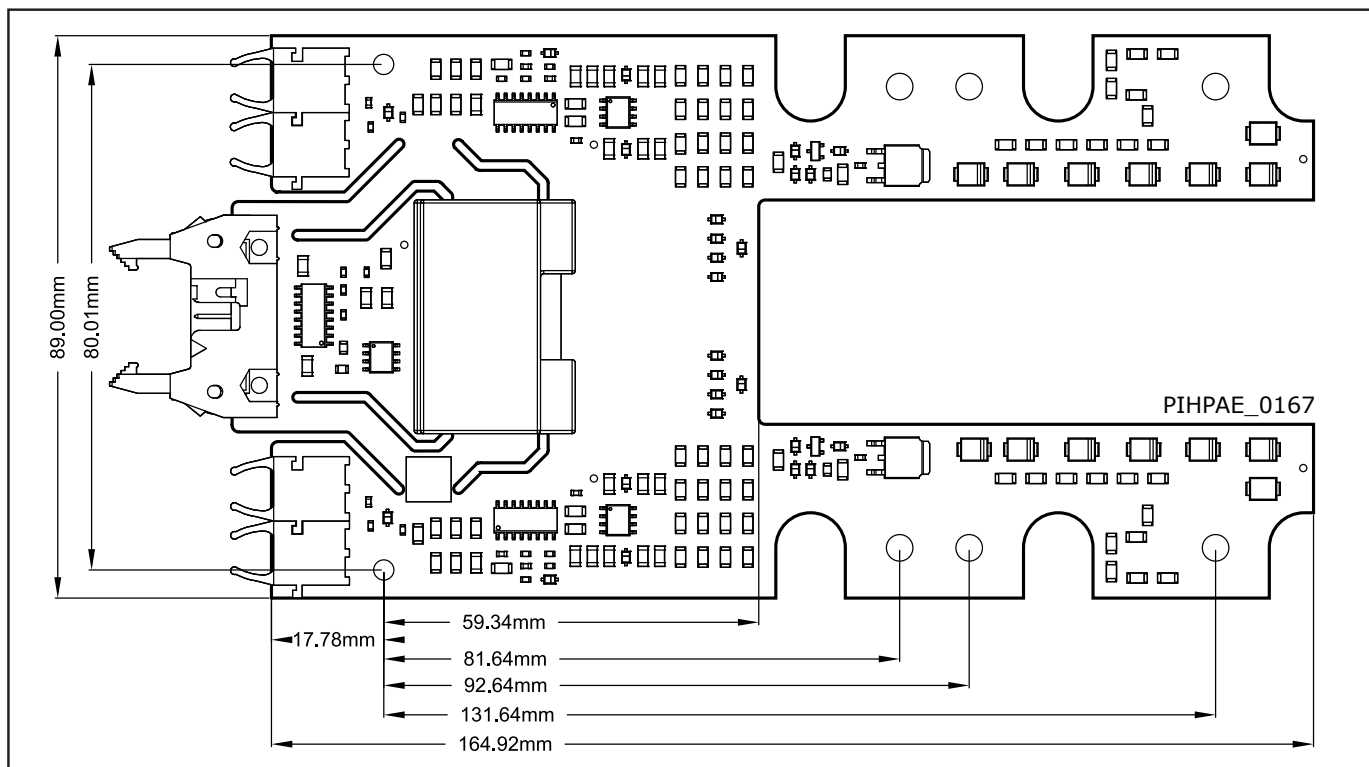
Figure 8. Top View of 2SP0430V2A0C
