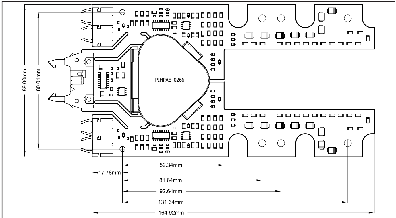
Figure 12. Top View of 2SP0430V2D0C
