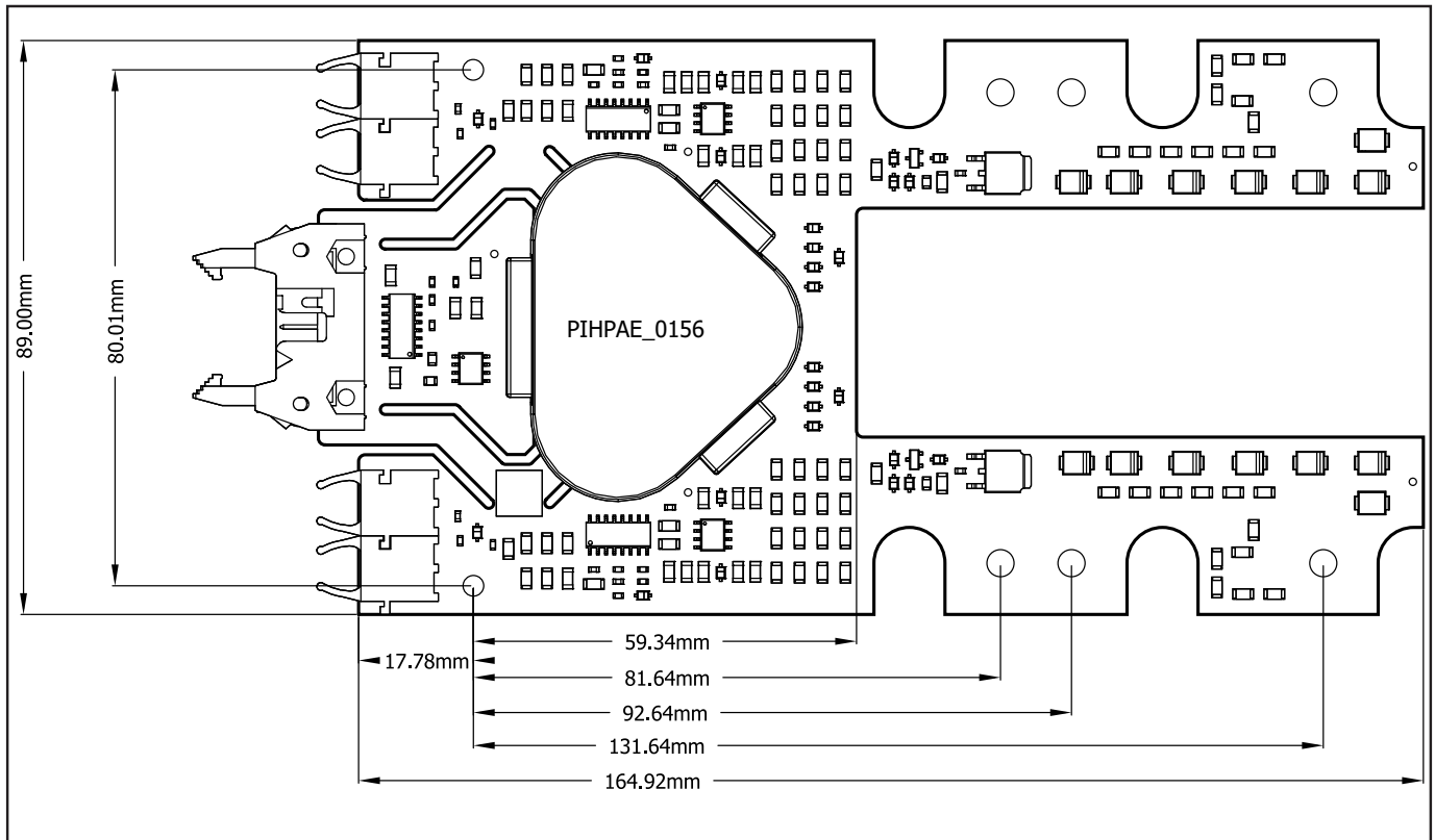
Figure 10. Top View of 2SP0430V2B0C
