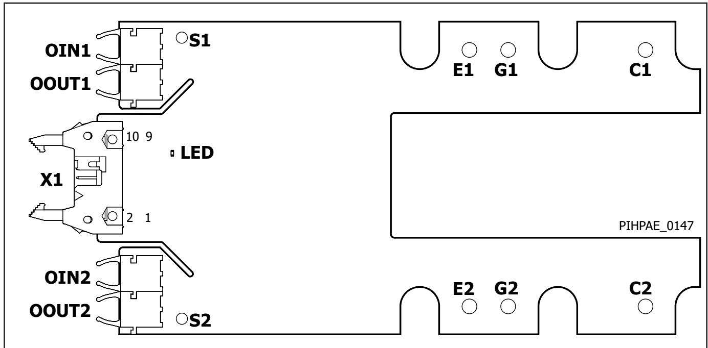
Figure 3. Pin Configuration.
