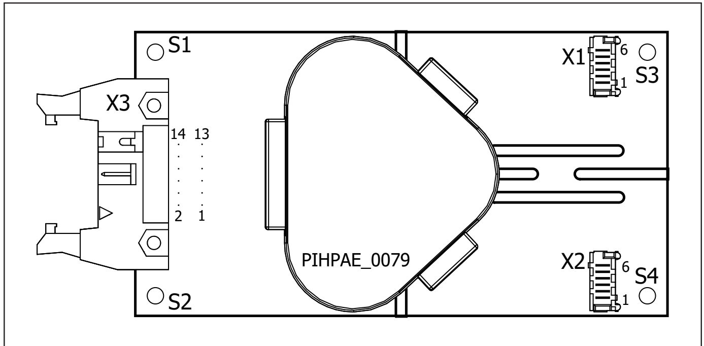
Figure 2. Pin Configuration.
