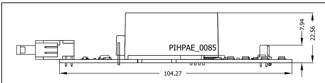
Figure 5. Side View.
