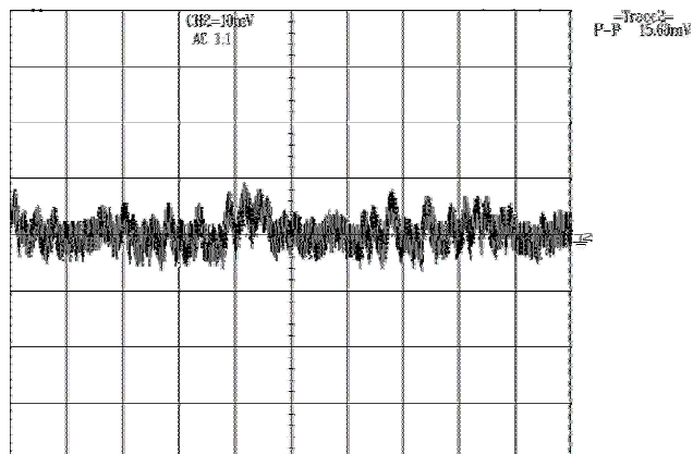
Figure 21 – Ripple, 85 VAC, Full Load. 2 ms, 10 mV / div.
