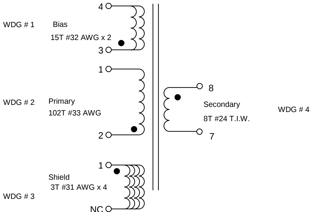
Figure 5 –Transformer Electrical Diagram.
