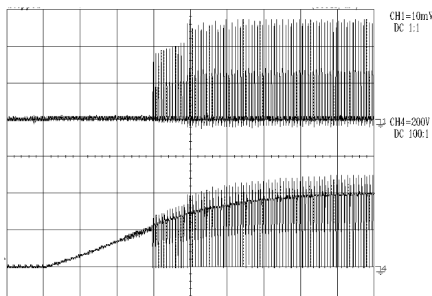
Figure 16 – 265 VAC Input and Maximum Load. Upper: I_{DRAIN} , 0.1 A / div. Lower: V_{DRAIN} , 200 V, 100 \mu s / div.
