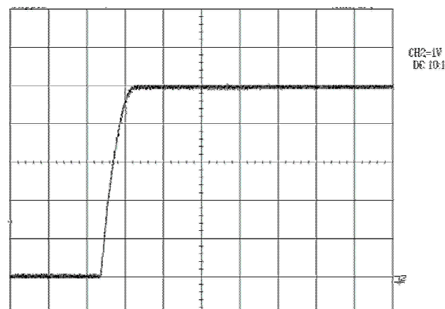
Figure 14 – Start-up Profile, 230 VAC 1 V, 5 ms / div.
