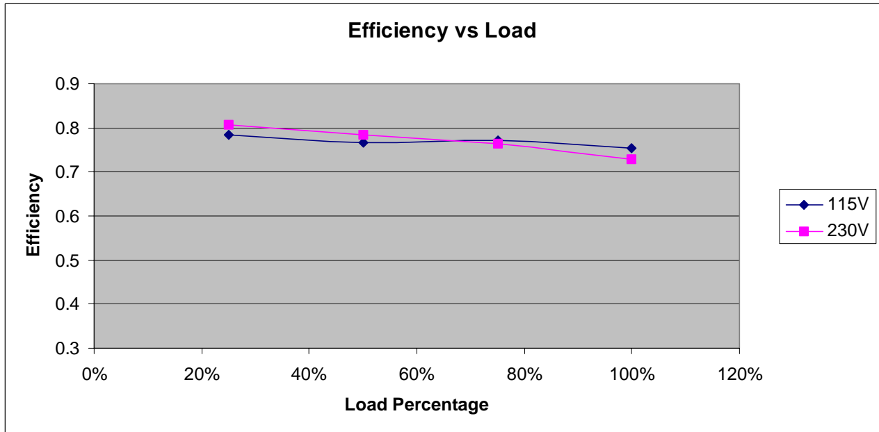
Figure 8 – Efficiency
