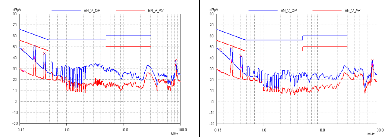
Figure 33 - Line, Secondary Floating
