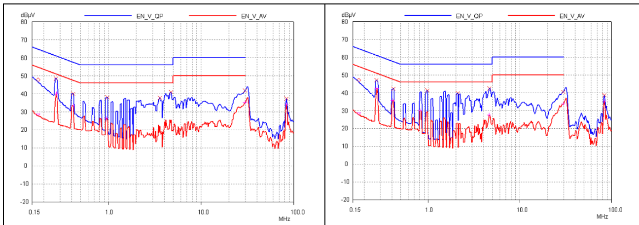
Figure 31 - Line, Secondary Grounded
