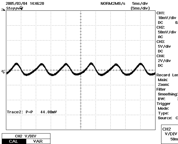
Figure 25 85 VAC, 12V. 5 ms, 50 mV / div
