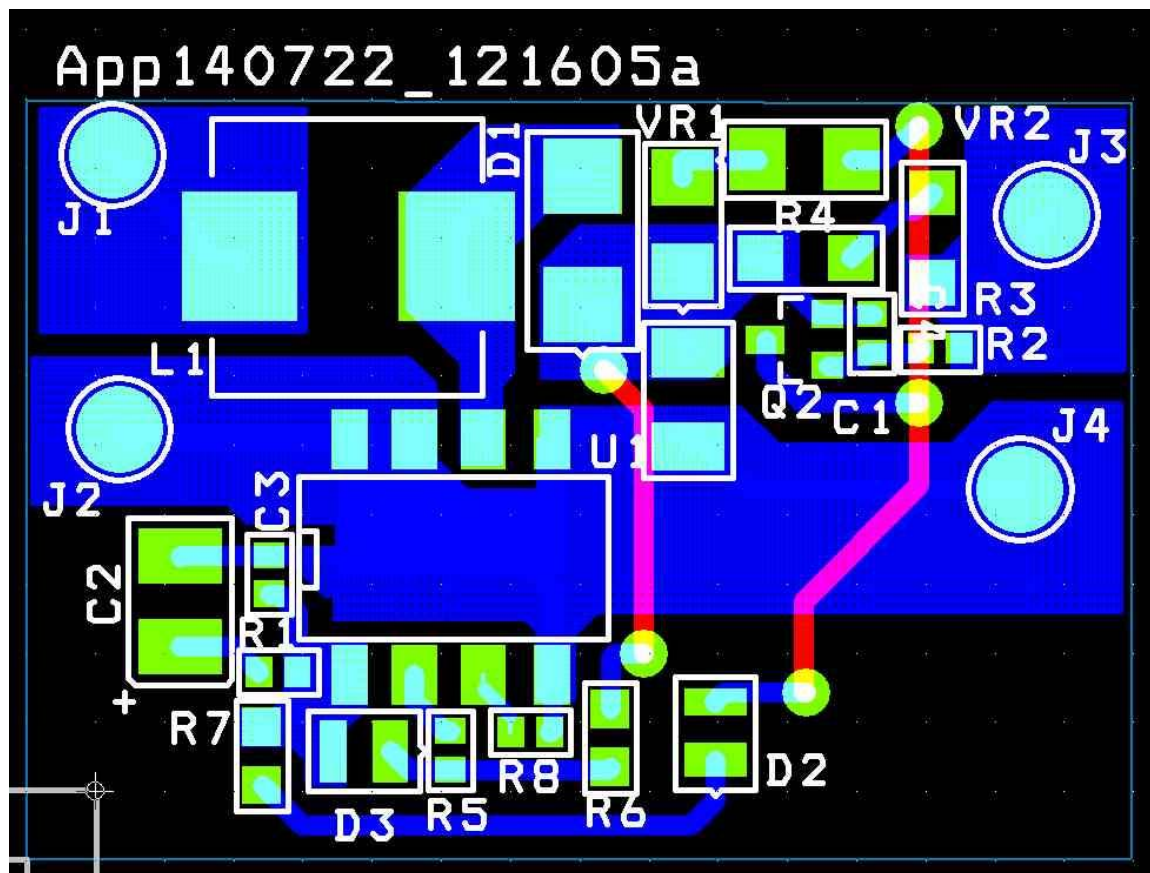
Figure 7 – Layout
