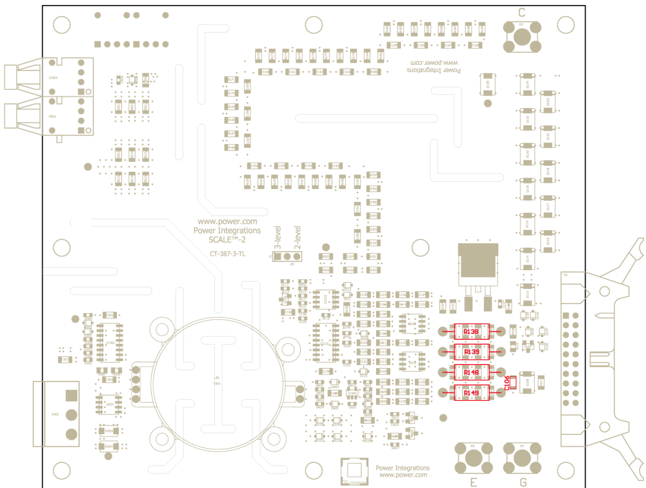
Fig. 1 Assembly drawing of 1SP0350V with highlighted gate resistors and auxiliary gate capacitor
