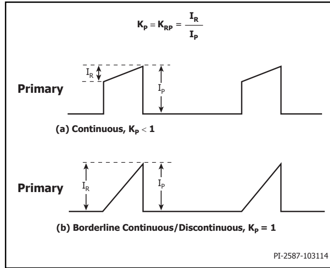
Figure 13. Continuous Conduction Mode Current Waveform, K_p < 1 .
