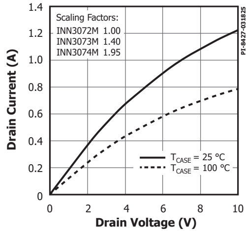
Figure 16. Output Characteristics.
