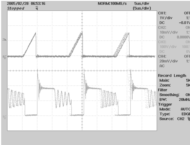
Figure 10 – 90 VAC, Full Load. Upper: I_{DRAIN} , 0.5 A / div Lower: V_{DRAIN} , 100 V, 2 \mu s / div
