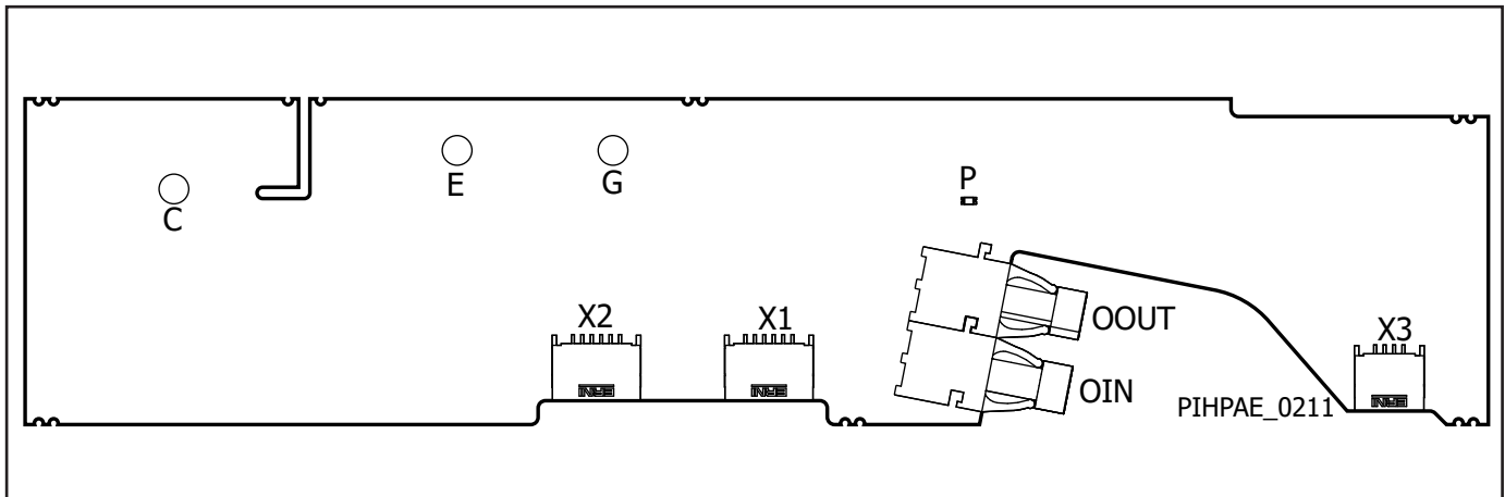
Figure 2. 1SP0635V2M1R Interfaces.
