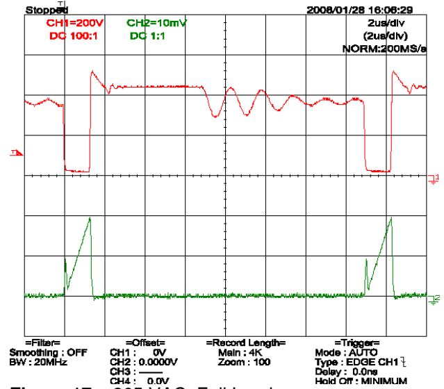
Figure 17 – 265 VAC, Full Load. Upper: V_{DRAIN} , 200 V / div. Lower: I_{DRAIN} , 200 mA / div, 2 us / div.
