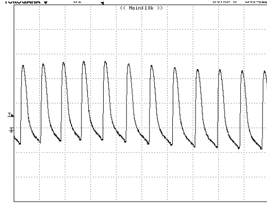
Figure 36 – Ripple, 265 VAC, Full Load, 20 mV, 20 \mu s / div.
