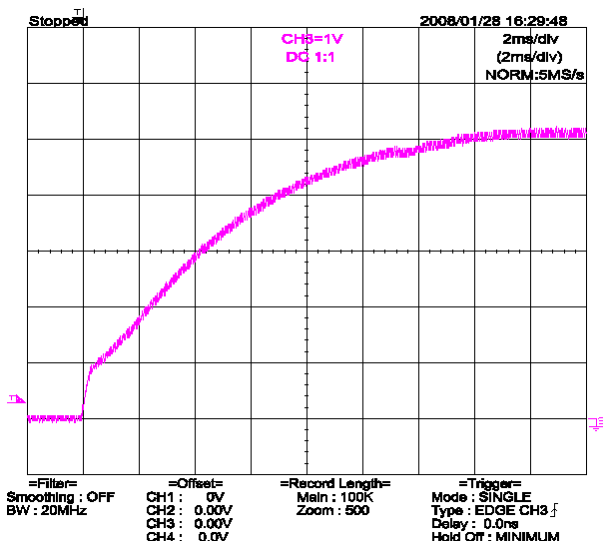
Figure 20 – Start-up Profile, 115 VAC, 1 V, 2 ms / div.
