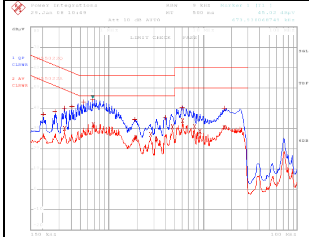
Figure 45 – 230 VAC Line, Output Earth Grounded.
