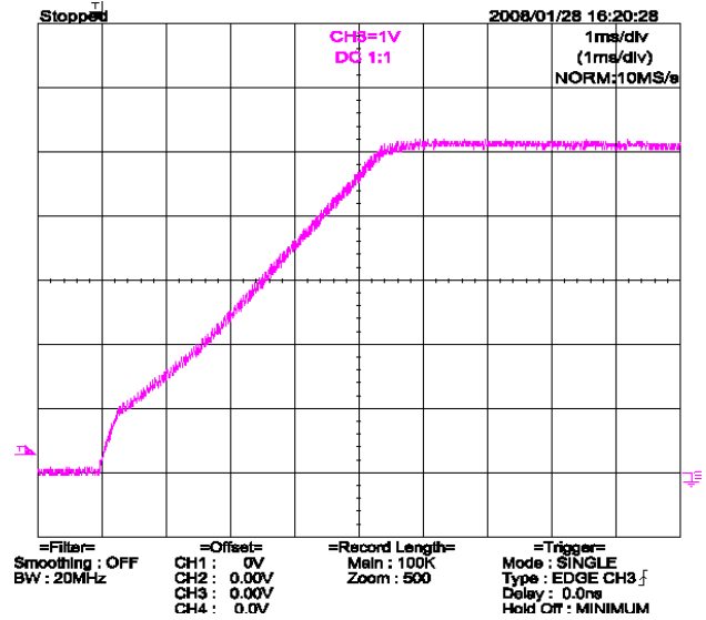
Figure 19 – Start-up Profile (No Load), 230 VAC, 1 V, 1 ms / div.
