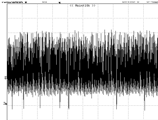
Figure 37 – Ripple, 265 VAC, Worst Case Noise, 20 mV / div, 5 ms / div.
