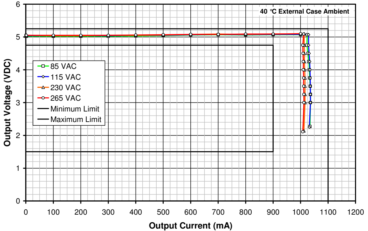
Figure 14 – Typical CV/CC Characteristic Over Line at 40 °C.
