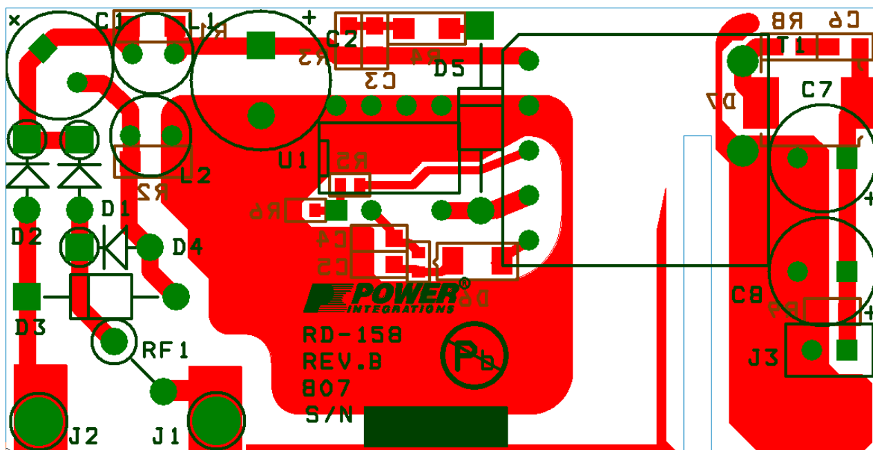
Figure 3 – Printed Circuit Layout.
