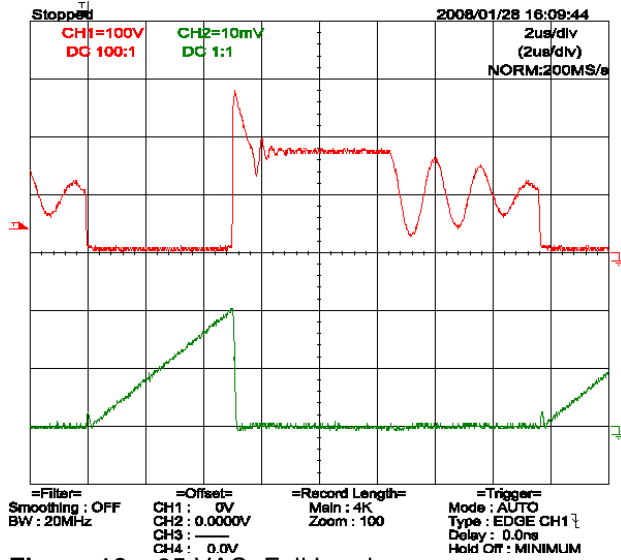
Figure 16 – 85 VAC, Full Load. Upper: V_{DRAIN} , 100 V / div. Lower: I_{DRAIN} , 200 mA / div, 2 us / div.
