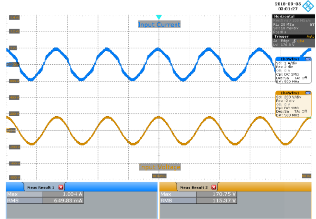
Figure 46 – 115 VAC 60 Hz, Full Load. Upper: I_{IN} , 1 A / div. Lower: V_{IN} , 200 V / div., 10 ms / div.
