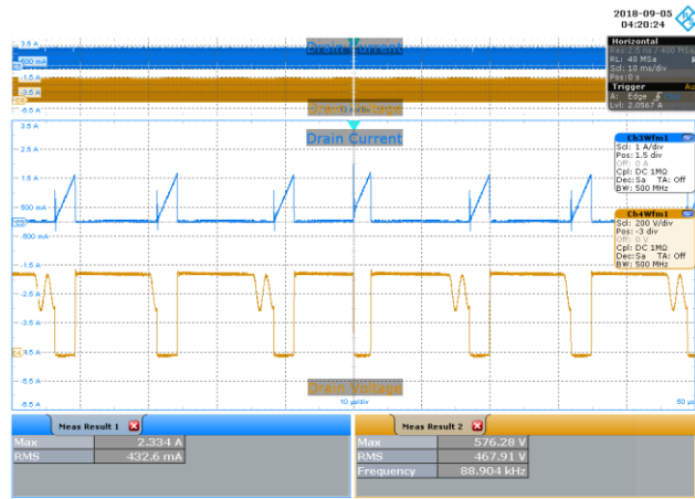
Figure 66 – 90 VAC 60 Hz, Full Load Normal. Upper: I_{DRAIN} , 1 A / div. Lower: V_{DRAIN} , 200 V / div., 10 \mu s / div.
