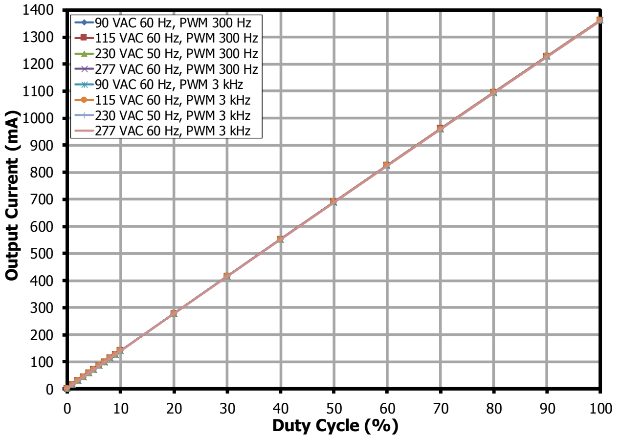
Figure 24 – Dimming Performance vs. Variable Duty PWM (300 Hz – 3 kHz)
