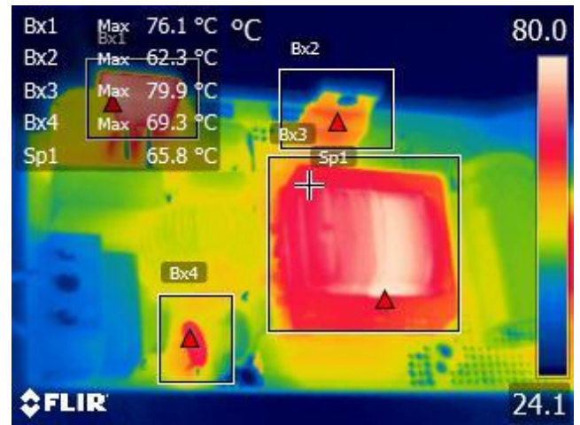
Figure 31 – Bx1 – Bridge Diode (BR1). Bx2 – PFC Output Diode (D5). Bx3 – PFC Inductor Winding (T2 Wire). Bx4 – Input Thermistor (RT1). Sp1 – PFC Inductor Core (T2 Core).
