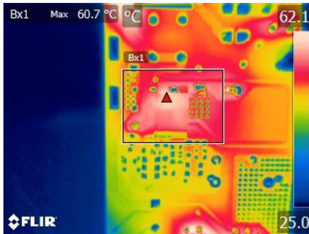
Figure 30 – HiperPFS-4 (U2).
