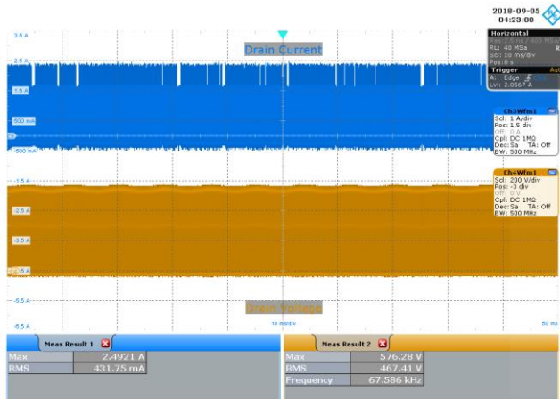
Figure 67 – 115 VAC 60 Hz, Full Load Normal. Upper: I_{DRAIN} , 1 A / div. Lower: V_{DRAIN} , 200 V / div., 10 ms / div.
