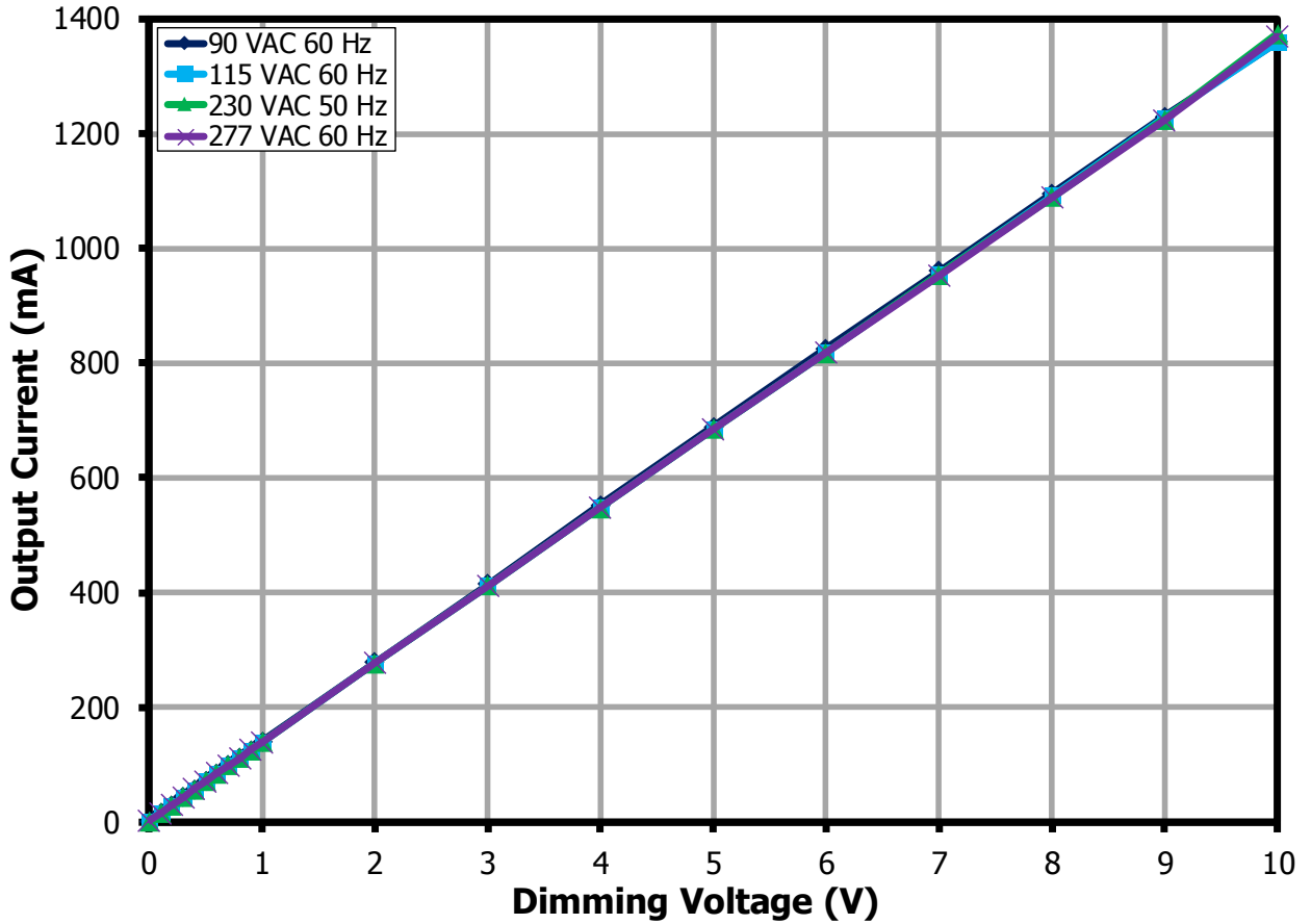
Figure 22 – Dimming Performance vs. Variable Supply (0 – 10 V)
