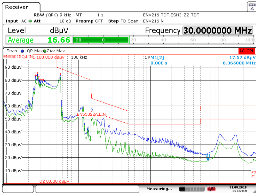
Figure 104 – Conducted EMI QP Scan at Full Load, Earthed, 115 VAC 60 Hz and EN55015 B Limits.
