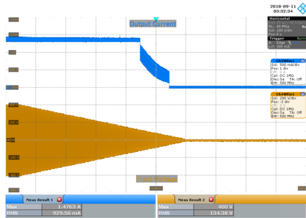
Figure 90 – 277 to 0 VAC 60 Hz, 1350 mA LED Load. Upper: 500 mA / div. Lower: 200 V / div. Horizontal: 100 s / div.
