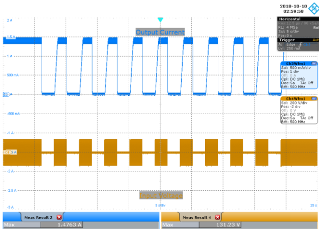
Figure 95 – 90 VAC 60 Hz, 36 V LED Load. 2 s On – 2 s Off. Upper: 500 mA / div. Lower: 200 V / div., 5 s / div. I_{OUT} Maximum: 1.48 A.
