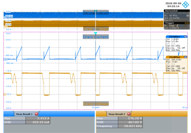
Figure 70 – 230 VAC 50 Hz, Full Load Normal. Upper: I_{DRAIN} , 1 A / div. Lower: V_{DRAIN} , 200 V / div., 10 \mu s / div.
