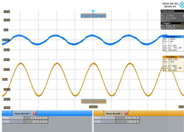
Figure 47 – 230 VAC 50 Hz, Full Load. Upper: I_{IN} , 1 A / div. Lower: V_{IN} , 200 V / div., 10 ms / div.
