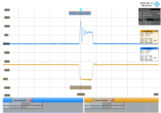
Figure 86 – 230 VAC 50 Hz, Output Shorted. Upper: I_{DRAIN} , 1 A / div. Lower: V_{DRAIN} , 200 V / div., 500 ns / div.
