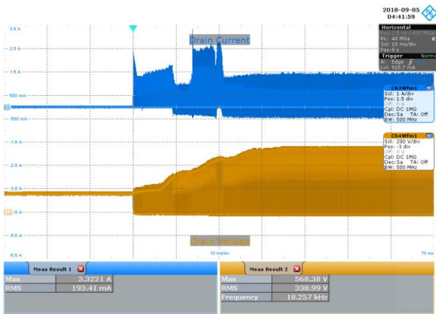
Figure 75 – 115 VAC 60 Hz, Full Load Start-up. Upper: I_{DRAIN} , 1 A / div. Lower: V_{DRAIN} , 200 V / div., 10 ms / div.
