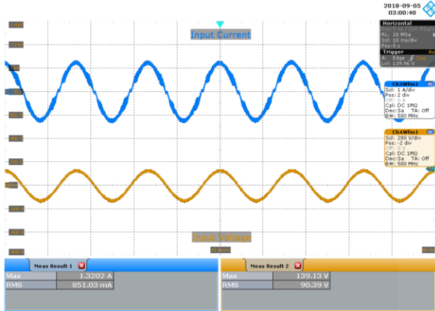
Figure 45 – 90 VAC 60 Hz, Full Load. Upper: I_{IN} , 1 A / div Lower: V_{IN} , 200 V / div, 10 ms / div.
