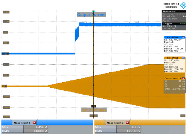
Figure 89 – 0 to 277 VAC 60 Hz, 1350 mA LED Load. Upper: 500 mA / div. Lower: 200 V / div. Horizontal: 100 s / div.
