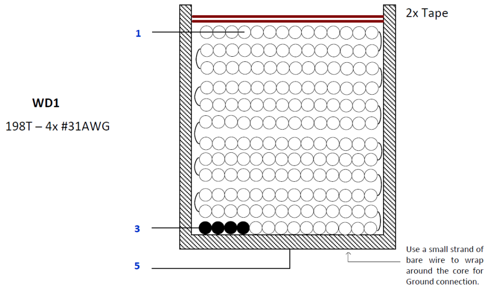
Figure 13 – Inductor Build Diagram.
