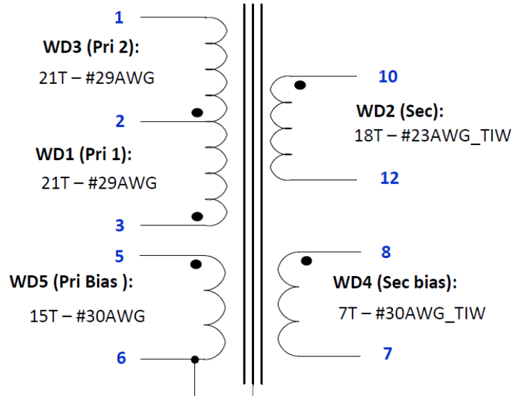
Figure 10 – Transformer Electrical Diagram.
