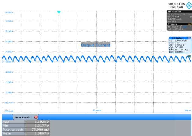
Figure 101 – 230 VAC 50 Hz, 1350 mA LED Load. 20 MHz Bandwidth. I_{OUT} , 100 mA / div., 50 \mu s / div. Ripple Current: 75.099 mA PK-PK .
