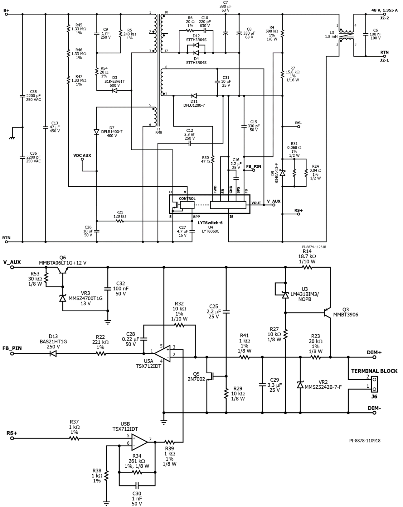
Figure 4 – Schematic.
