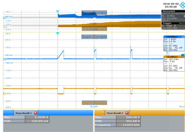
Figure 74 – 90 VAC 60 Hz, Full Load Start-up. Upper: I_{DRAIN} , 1 A / div. Lower: V_{DRAIN} , 200 V / div., 20 \mu s / div.
