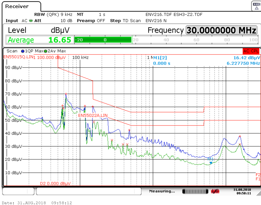
Figure 106 – Conducted EMI QP Scan at Full Load, Earthed, 230 VAC 60 Hz and EN55015 B Limits.
