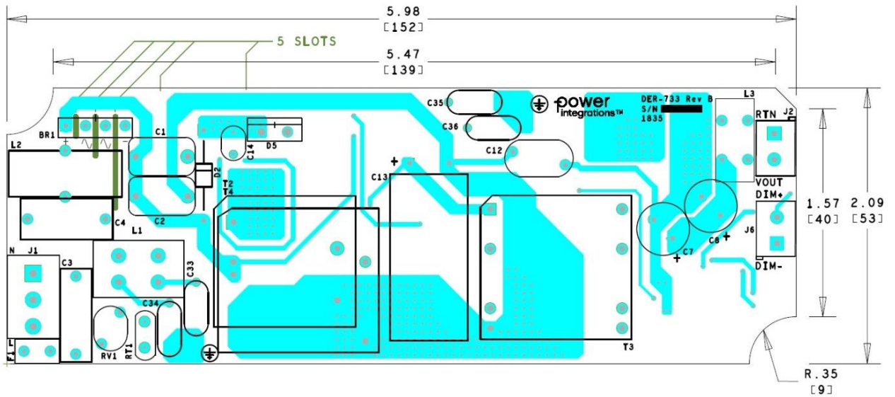
Figure 8 – Top Side.
