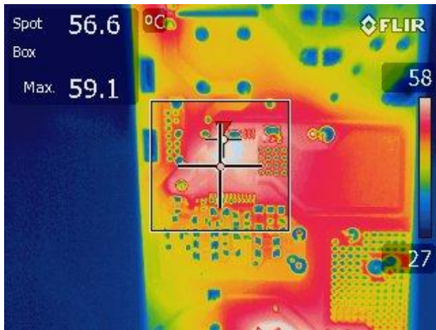
Figure 34 – HiperPFS-4 (U2).
