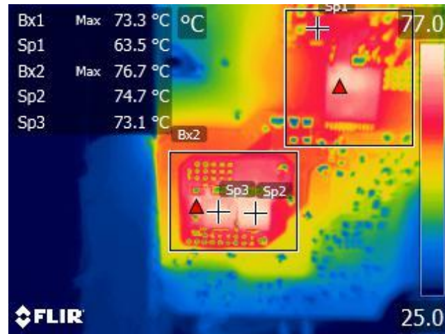
Figure 37 – Bx1 – LYTSwitch-6 (U4). Bx2 – Output Diode Snubber Resistor (R6). Sp1 – DCDC Primary Snubber Clamp Diode (D3). Sp2 – Output Diode (D12). Sp3 – Output Diode (D4).
