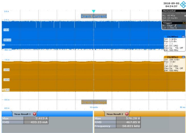
Figure 69 – 230 VAC 50 Hz, Full Load Normal. Upper: I_{DRAIN} , 1 A / div. Lower: V_{DRAIN} , 200 V / div., 10 ms / div.
