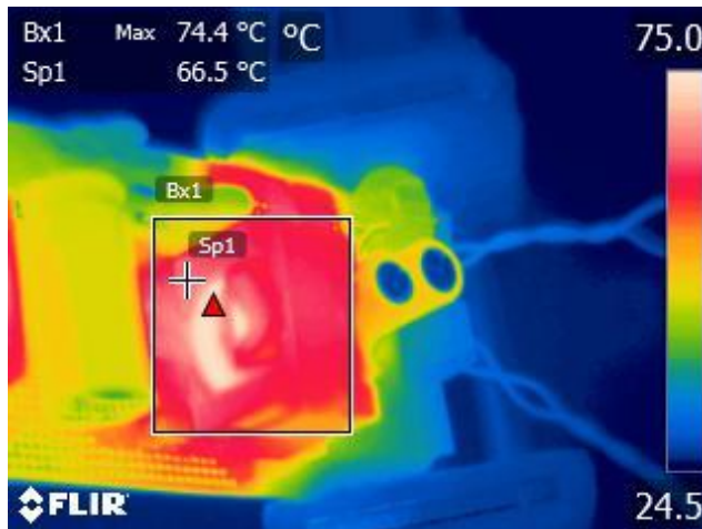
Figure 32 – Bx1 – DCDC Main Transformer Winding (T3 Wire). Sp1 – DCDC Main Transformer Core (T3 Core).
