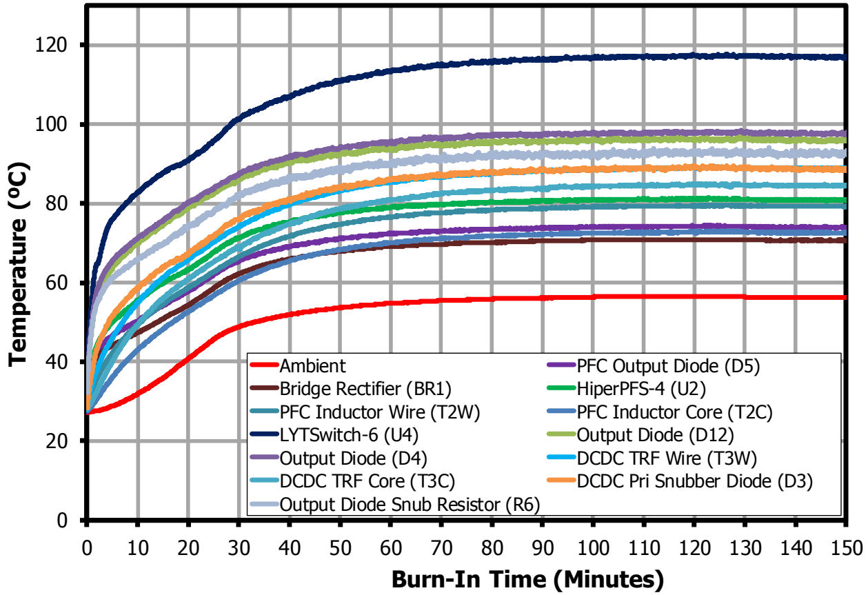
Figure 44 – Component Temperature at 55 °C Ambient - Open Frame (High Line – 277 VAC).
