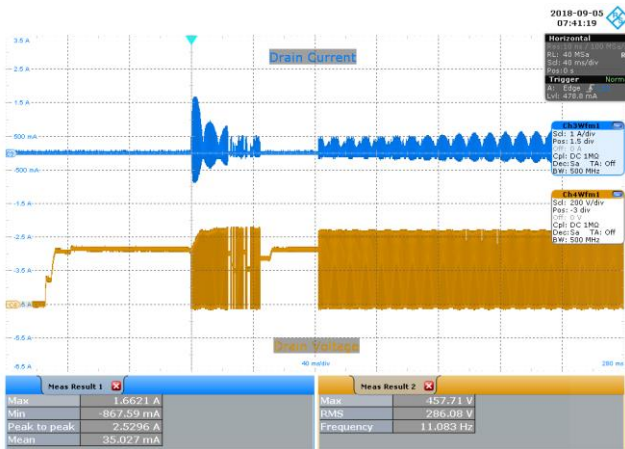
Figure 63 – 230 VAC 50 Hz, Full Load Start-up. Upper: I_{DRAIN} , 1 A / div. Lower: V_{DRAIN} , 200 V / div., 40 ms / div.
