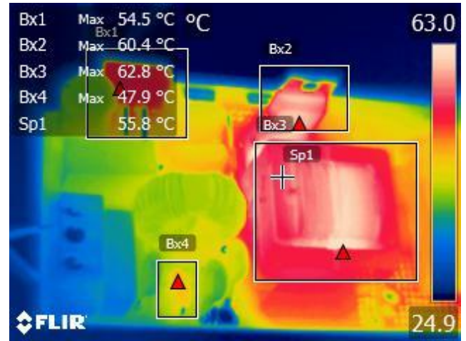
Figure 39 – Bx1 – Bridge Diode (BR1). Bx2 – PFC Output Diode (D5). Bx3 – PFC Inductor Winding (T2 Wire). Bx4 – Input Thermistor (RT1). Sp1 – PFC Inductor Core (T2 Core).
