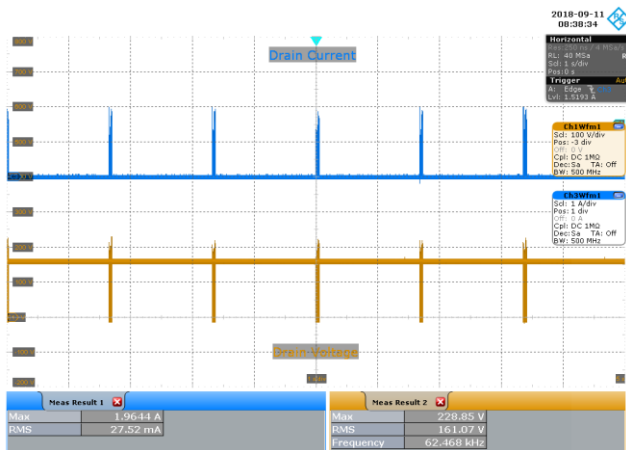
Figure 81 – 90 VAC 60 Hz, Output Shorted. Upper: I_{DRAIN} , 1 A / div. Lower: V_{DRAIN} , 100 V / div., 1 s / div. P_{IN} Average: 34 mW.
