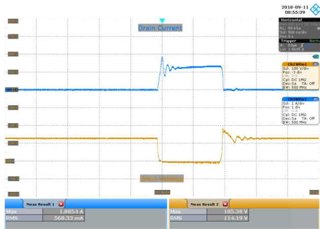
Figure 82 – 90 VAC 60 Hz, Output Shorted. Upper: I_{DRAIN} , 1 A / div. Lower: V_{DRAIN} , 100 V / div., 500 ns / div.
