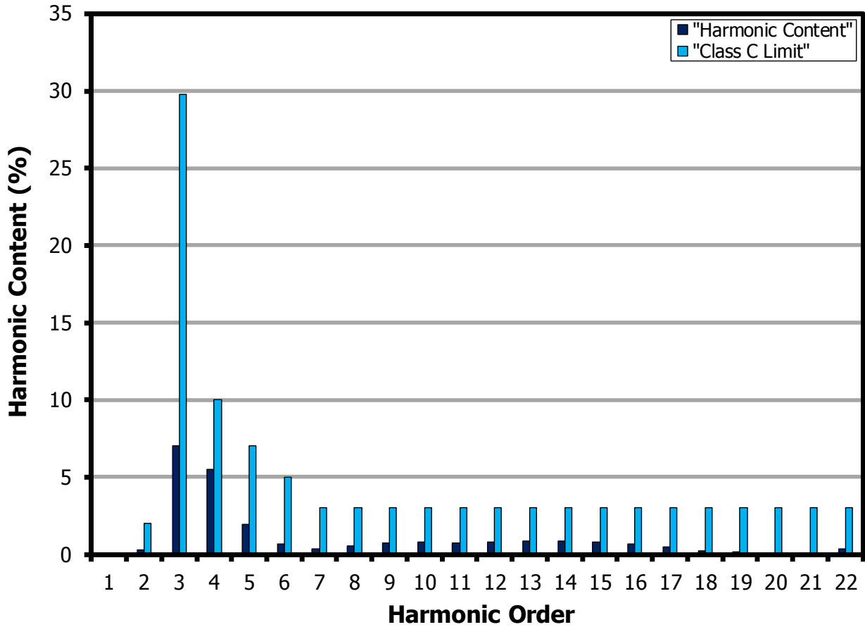
Figure 18 – Full Load Input Current Harmonics at 115 VAC 60 Hz.
