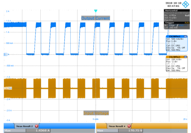
Figure 92 – 115 VAC 60 Hz, 48 V LED Load. 2 s On – 2 s Off. Upper: 500 mA / div. Lower: 200 V / div., 5 s / div. I_{OUT} Maximum: 1.44 A.
