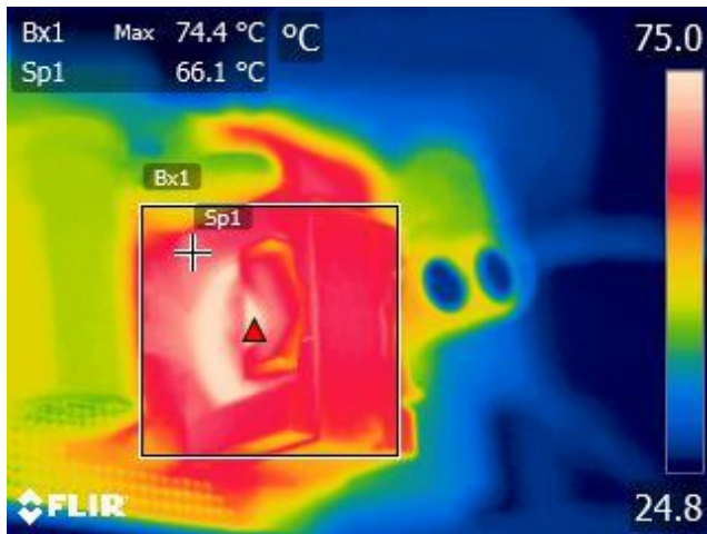
Figure 36 – Bx1 – DCDC Main Transformer Winding (T3 Wire). Sp1 – DCDC Main Transformer Core (T3 Core).
