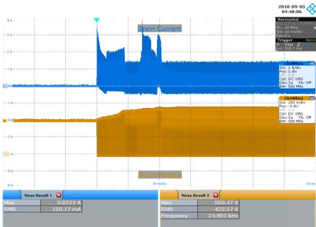
Figure 79 – 277 VAC 60 Hz, Full Load Start-up. Upper: I_{DRAIN} , 1 A / div. Lower: V_{DRAIN} , 200 V / div., 10 ms / div.
