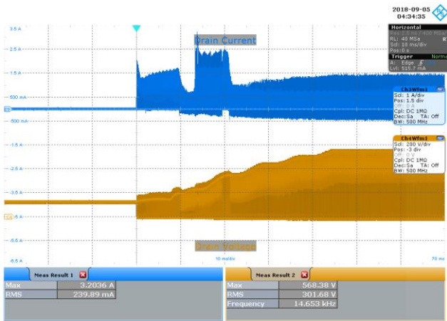
Figure 73 – 90 VAC 60 Hz, Full Load Start-up. Upper: I_{DRAIN} , 1 A / div. Lower: V_{DRAIN} , 200 V / div., 10 ms / div.
