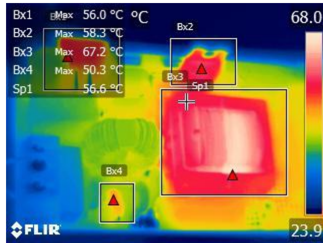
Figure 35 – Bx1 – Bridge Diode (BR1). Bx2 – PFC Output Diode (D5). Bx3 – PFC Inductor Winding (T2 Wire). Bx4 – Input Thermistor (RT1). Sp1 – PFC Inductor Core (T2 Core).
