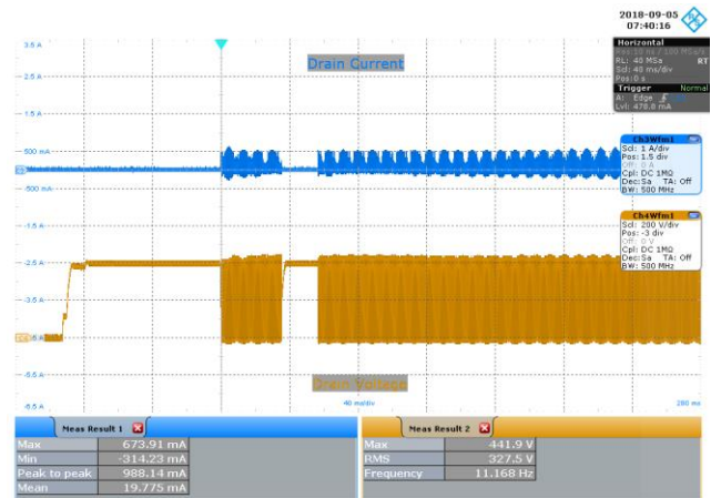
Figure 64 – 277 VAC 60 Hz, Full Load Start-up. Upper: I_{DRAIN} , 1 A / div. Lower: V_{DRAIN} , 200 V / div., 40 ms / div.
