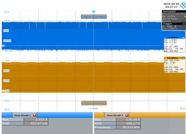
Figure 71 – 277 VAC 60 Hz, Full Load Normal. Upper: I_{DRAIN} , 1 A / div. Lower: V_{DRAIN} , 200 V / div., 10 ms / div.
