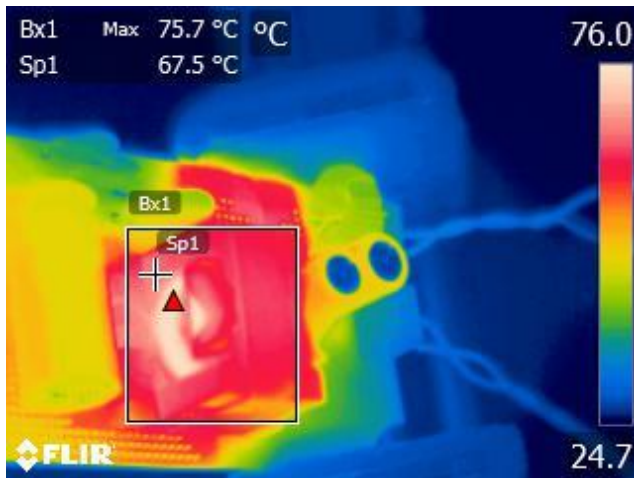
Figure 28 – Bx1 – DCDC Main Transformer Winding (T3 Wire). Sp1 – DCDC Main Transformer Core (T3 Core).
