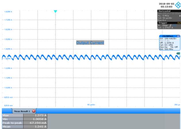
Figure 99 – 90 VAC 60 Hz, 1350 mA LED Load. 20 MHz Bandwidth. I_{OUT} , 100 mA / div., 50 \mu s / div. Ripple Current: 67.194 mA PK-PK .
