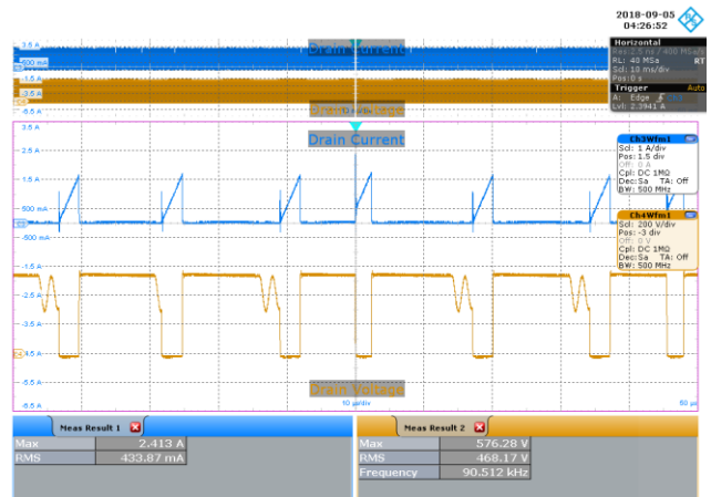
Figure 72 – 277 VAC 60 Hz, Full Load Normal. Upper: I_{DRAIN} , 1 A / div. Lower: V_{DRAIN} , 200 V / div., 10 \mu s / div.
