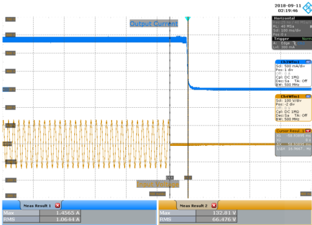
Figure 53 – 90 VAC 60 Hz, Full Load, Output Fall. Upper: I_{OUT} , 500 mA / div. Lower: V_{IN} , 100 V / div., 100 ms / div. Turn On Time: 59 ms.
