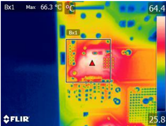
Figure 38 – HiperPFS-4 (U2).
