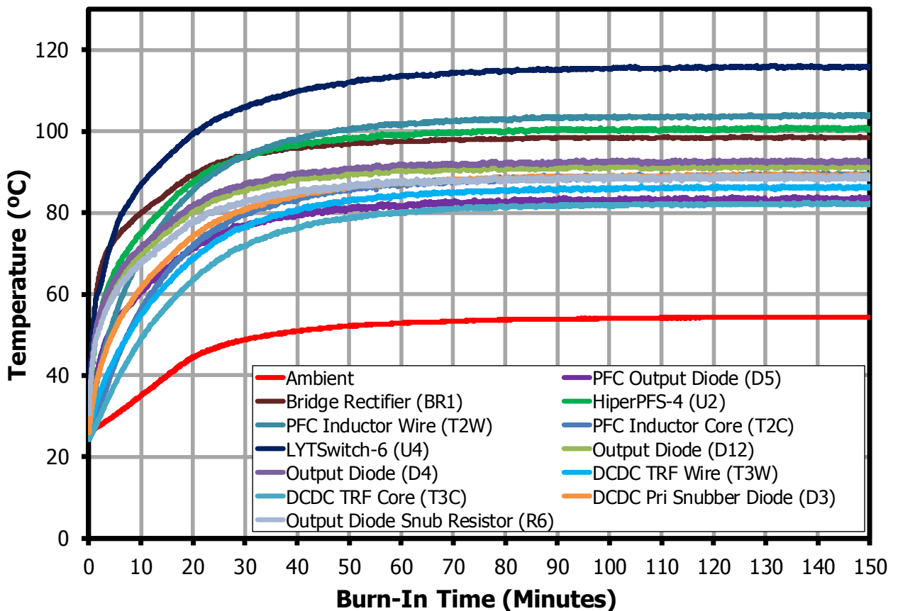
Figure 43 – Component Temperature at 55 °C Ambient - Open Frame (Low Line – 90 VAC).
