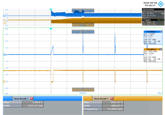
Figure 78 – 230 VAC 50 Hz, Full Load Start-up. Upper: I_{DRAIN} , 1 A / div. Lower: V_{DRAIN} , 200 V / div., 20 \mu s / div.
