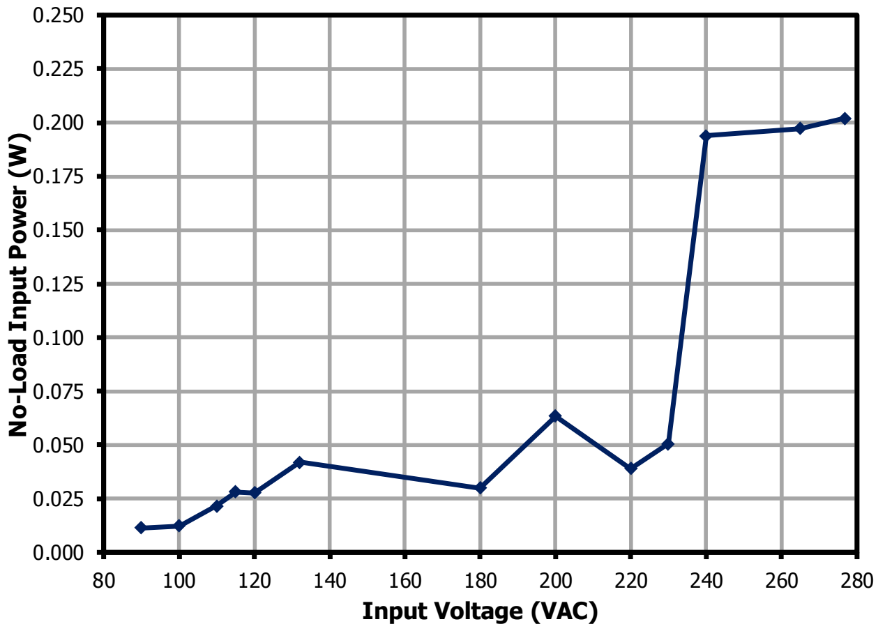
Figure 20 – No-Load Input Power vs. Input Line Voltage.
