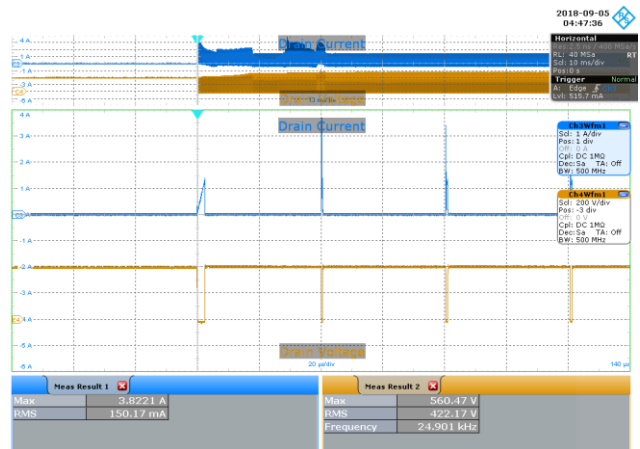
Figure 80 – 277 VAC 60 Hz, Full Load Start-up. Upper: I_{DRAIN} , 1 A / div. Lower: V_{DRAIN} , 200 V / div., 20 \mu s / div.
