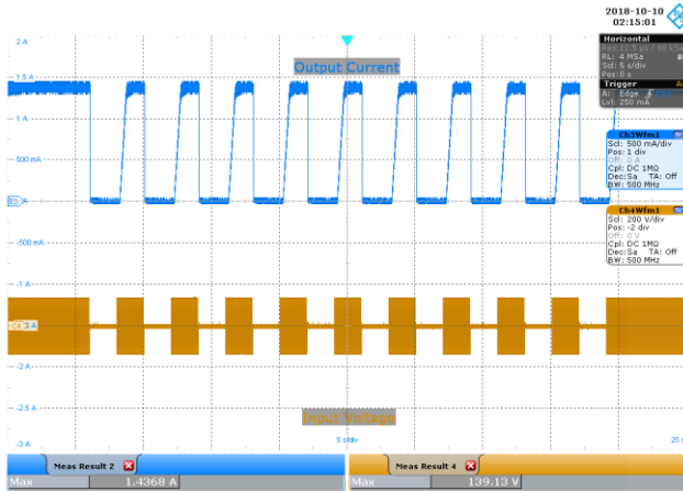
Figure 91 – 90 VAC 60 Hz, 48 V LED Load. 2 s On – 2 s Off. Upper: 500 mA / div. Lower: 200 V / div., 5 s / div. I_{OUT} Maximum: 1.44 A.
