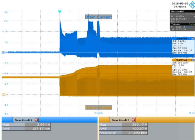
Figure 77 – 230 VAC 50 Hz, Full Load Start-up. Upper: I_{DRAIN} , 1 A / div. Lower: V_{DRAIN} , 200 V / div., 10 ms / div.
