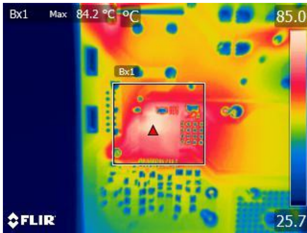
Figure 26 – HiperPFS-4 (U2).
