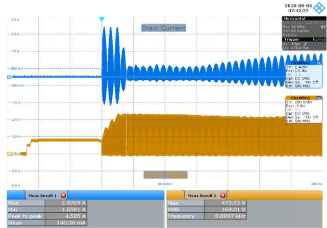
Figure 62 – 115 VAC 60 Hz, Full Load Start-up. Upper: I_{DRAIN} , 1 A / div. Lower: V_{DRAIN} , 200 V / div., 40 ms / div.
