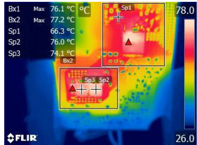
Figure 29 – Bx1 – LYTSwitch-6 (U4). Bx2 – Output Diode Snubber Resistor (R6). Sp1 – DCDC Primary Snubber Clamp Diode (D3). Sp2 – Output Diode (D12). Sp3 – Output Diode (D4).
