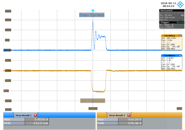
Figure 88 – 277 VAC 60 Hz, Output Shorted. Upper: I_{DRAIN} , 1 A / div. Lower: V_{DRAIN} , 200 V / div., 500 ns / div.
