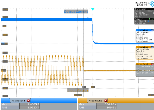
Figure 55 – 230 VAC 50 Hz, Full Load, Output Fall. Upper: V_{OUT} , 500 mA / div. Lower: V_{IN} , 200 V / div., 100 ms / div. Hold-up Time: 59 ms.
