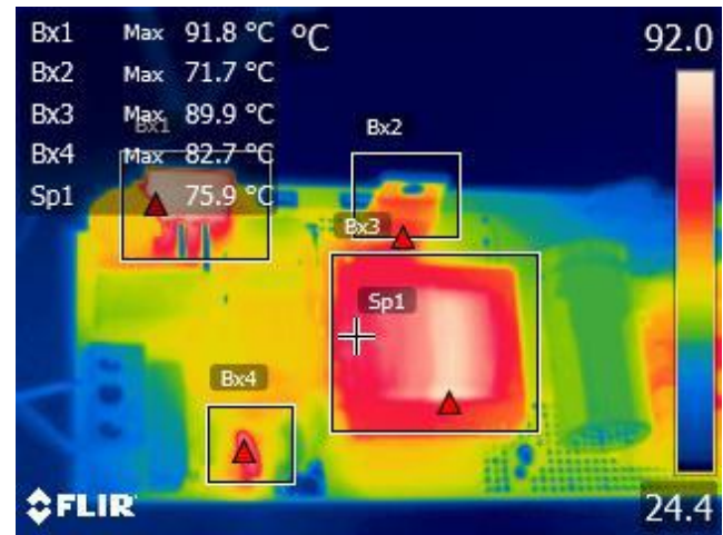
Figure 27 – Bx1 – Bridge Diode (BR1); Bx2 – PFC Output Diode (D5). Bx3 – PFC Inductor Winding (T2 Wire). Bx4 – Input Thermistor (RT1). Sp1 – PFC Inductor Core (T2 Core).
