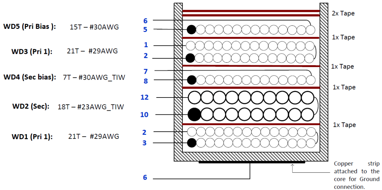
Figure 11 – Transformer Build Diagram.
