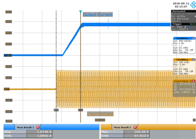
Figure 50 – 115 VAC 60 Hz, Full Load Start-up. Upper: I_{OUT} , 500 mA / div. Lower: V_{IN} , 100 V / div., 500 ms / div. Turn On Time: 637 ms.
