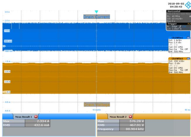
Figure 65 – 90 VAC 60 Hz, Full Load Normal. Upper: I_{DRAIN} , 1 A / div. Lower: V_{DRAIN} , 200 V / div., 10 ms / div.
