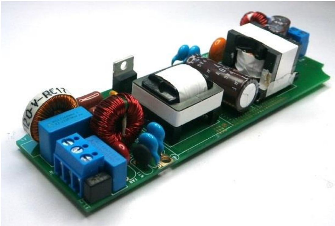
Figure 1 – Populated Circuit Board.
