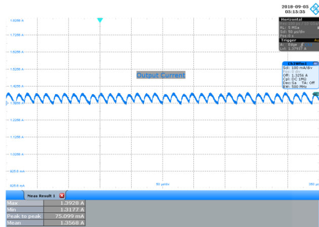
Figure 102 – 277 VAC 50 Hz, 1350 mA LED Load. 20 MHz Bandwidth. I_{OUT} , 100 mA / div., 50 \mu s / div. Ripple Voltage: 75.099 mA PK-PK .
