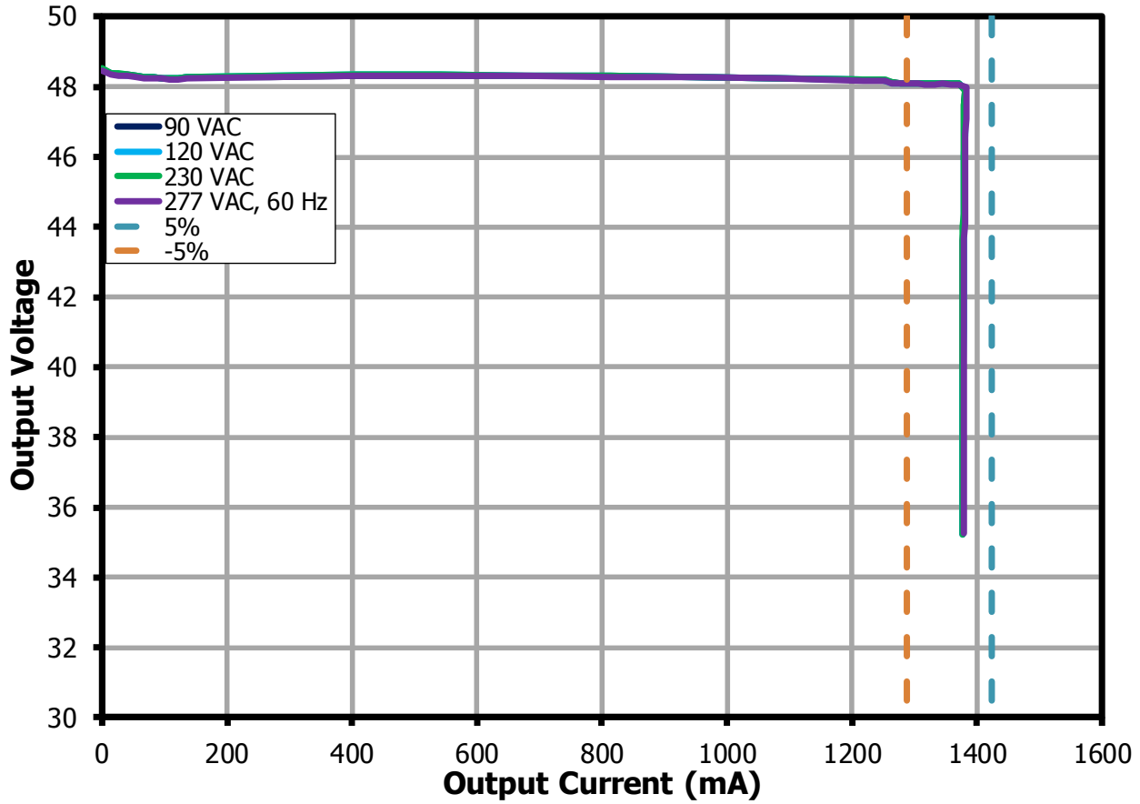
Figure 21 – CV/CC Curve.
