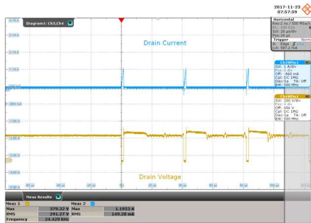
Figure 76 – 115 VAC 60 Hz, Full Load Start-up. Upper: I_{DRAIN} , 1 A / div. Lower: V_{DRAIN} , 200 V / div., 20 \mu s / div.
