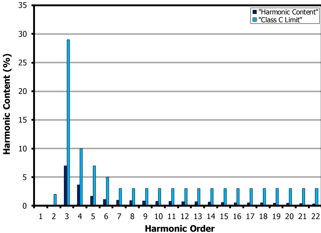
Figure 19 – Full Load Input Current Harmonics at 230 VAC 50 Hz.
