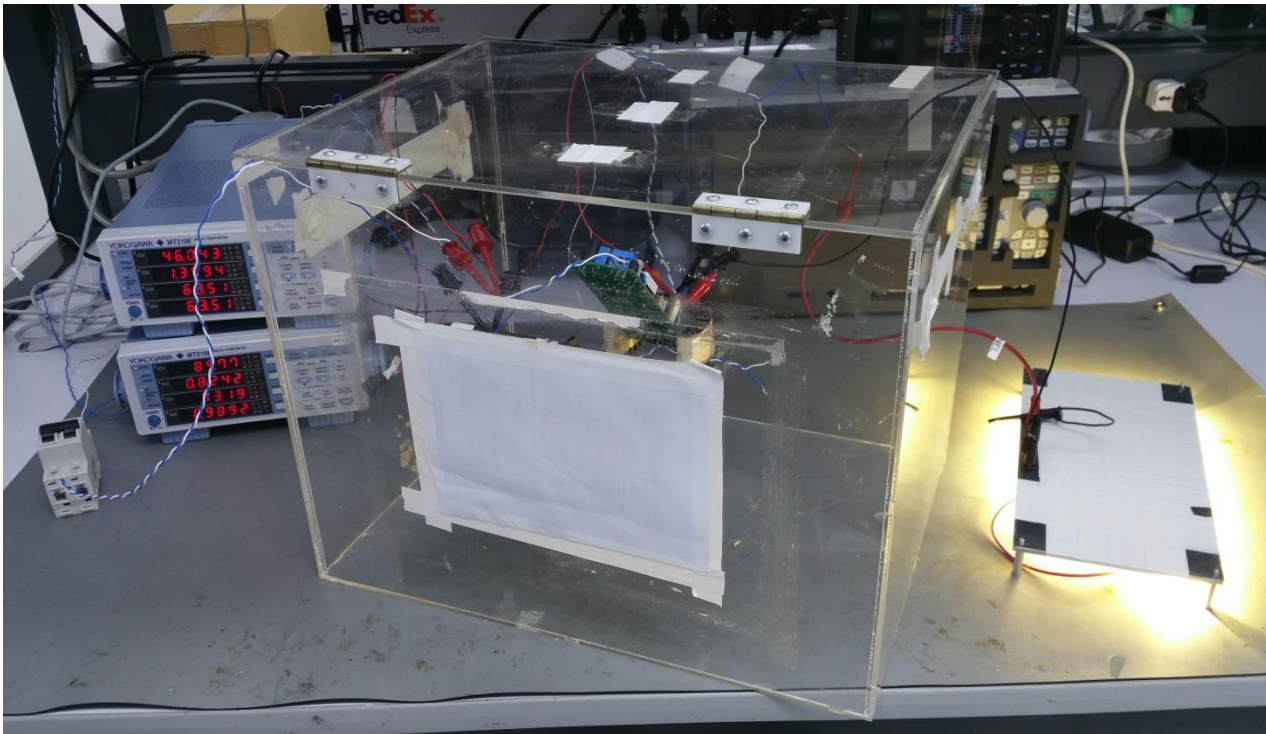
Figure 25 – Test Set-up Picture - Open Frame.
