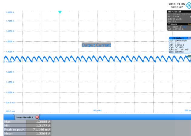
Figure 100 – 115 VAC 60 Hz, 1350 mA LED Load. 20 MHz Bandwidth. I_{OUT} , 100 mA / div., 50 \mu s / div. Ripple Current: 71.146 mA PK-PK .
