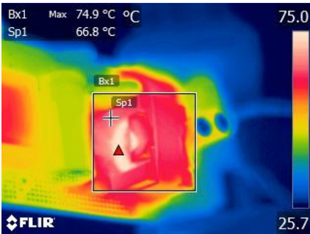
Figure 40 – Bx1 – DCDC Main Transformer Winding (T3 Wire). Sp1 – DCDC Main Transformer Core (T3 Core).
