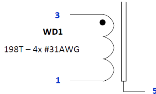
Figure 12 – Inductor Electrical Diagram.
