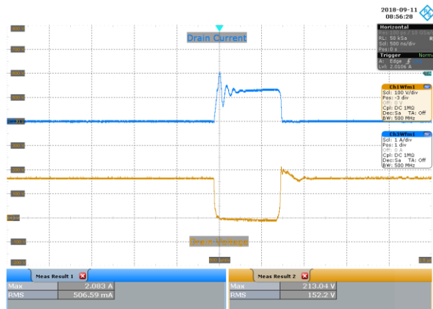
Figure 84 – 115 VAC 60 Hz, Output Shorted. Upper: I_{DRAIN} , 1 A / div. Lower: V_{DRAIN} , 100 V / div., 500 ns / div.
