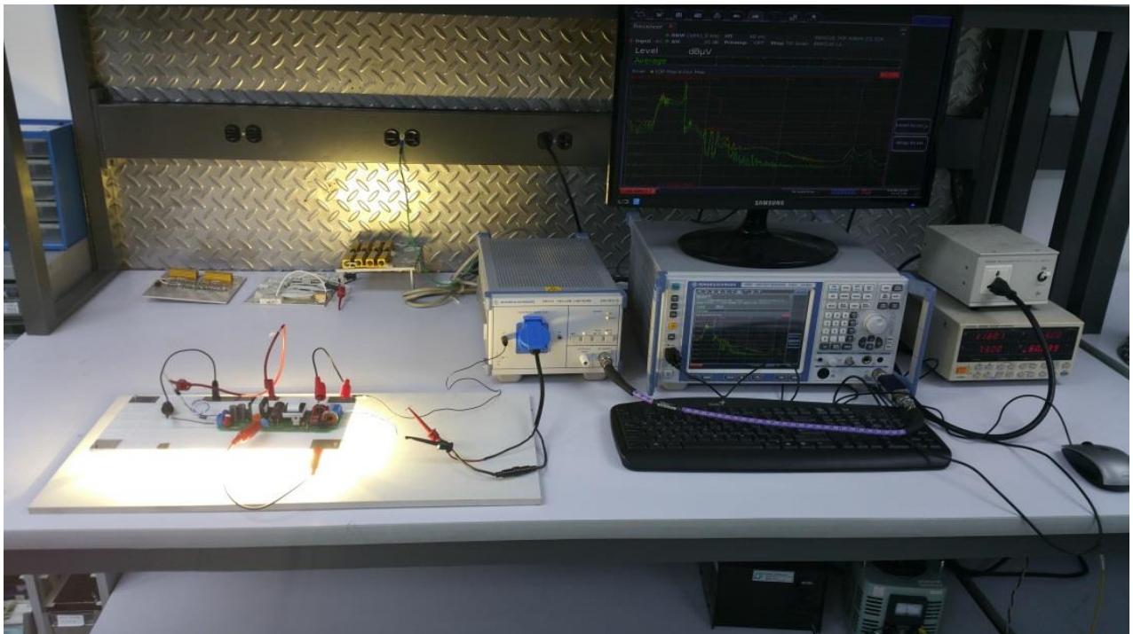
Figure 103 — Conducted EMI Test Set-up.
