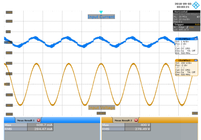
Figure 48 – 277 VAC 60 Hz, Full Load. Upper: I_{IN} , 1 A / div. Lower: V_{IN} , 200 V / div., 10 ms / div.
