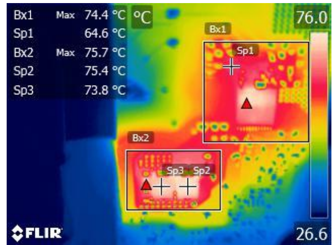
Figure 41 – Bx1 – LYTSwitch-6 (U4). Bx2 – Output Diode Snubber Resistor (R6). Sp1 – DCDC Primary Snubber Clamp Diode (D3). Sp2 – Output Diode (D12). Sp3 – Output Diode (D4).
