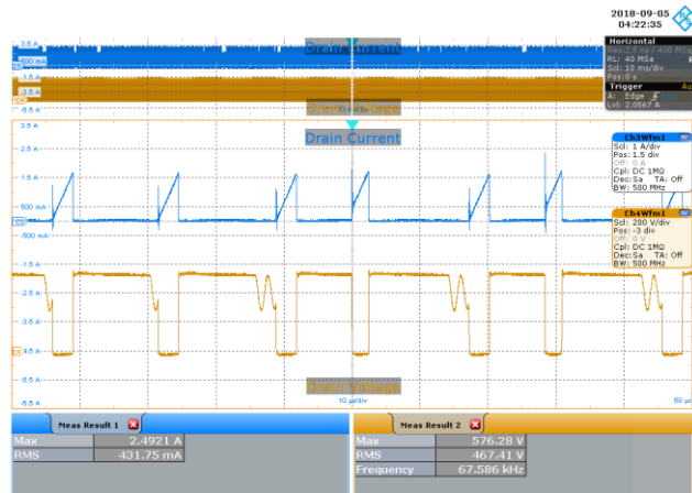
Figure 68 – 115 VAC 60 Hz, Full Load Normal. Upper: I_{DRAIN} , 1 A / div. Lower: V_{DRAIN} , 200 V / div., 10 \mu s / div.
